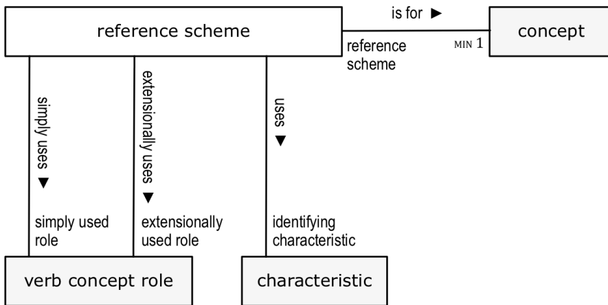
Figure 11.3 - Reference Scheme
