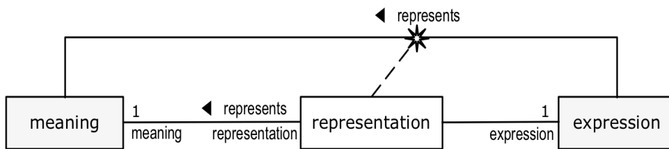
Figure 12.1 - Representation
