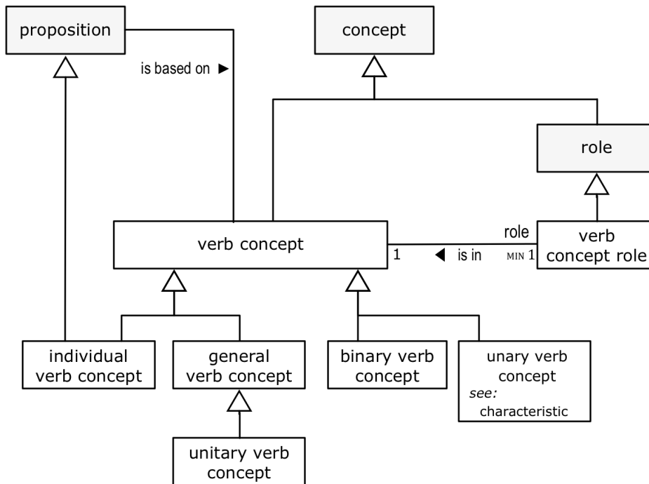
Figure 11.2 - Verb Concepts
