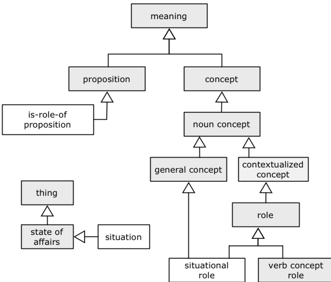
Figure 14.8 - Situations
