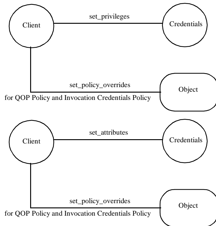
Figure 15-32 Changing Security Attributes
