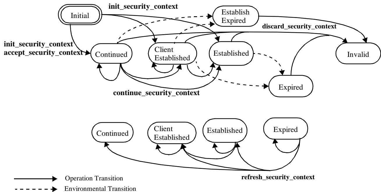
Figure 15-55 Security Context State Transition Diagram
