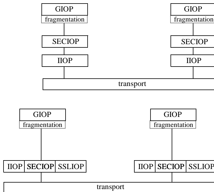
Figure 15-58 Position of SECIOP Protocol
