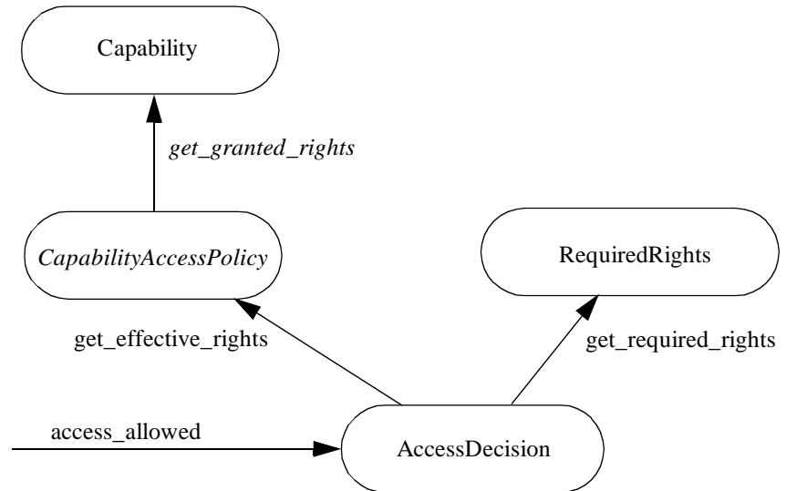
Figure 15-71 Retrieving Granted Rights
