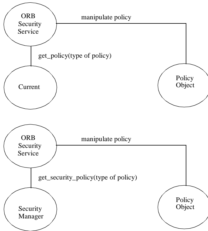
Figure 15-48 get_policy / get_security_policy Operation
