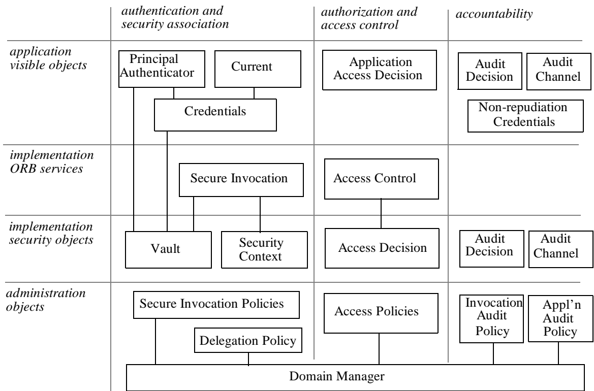
Figure 15-53 Relationship Between Main Objects
