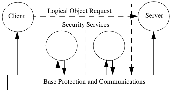
Figure 15-65 Base Protection and Communications
