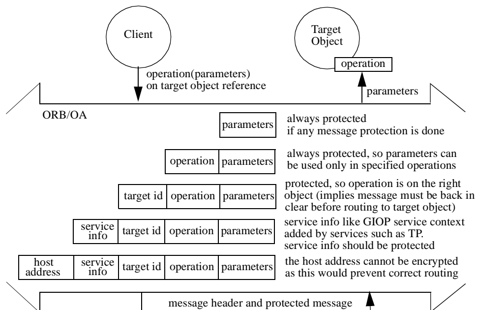
Figure 2-4 Message Protection
