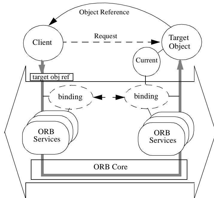
Figure 2-24 Object Reference
