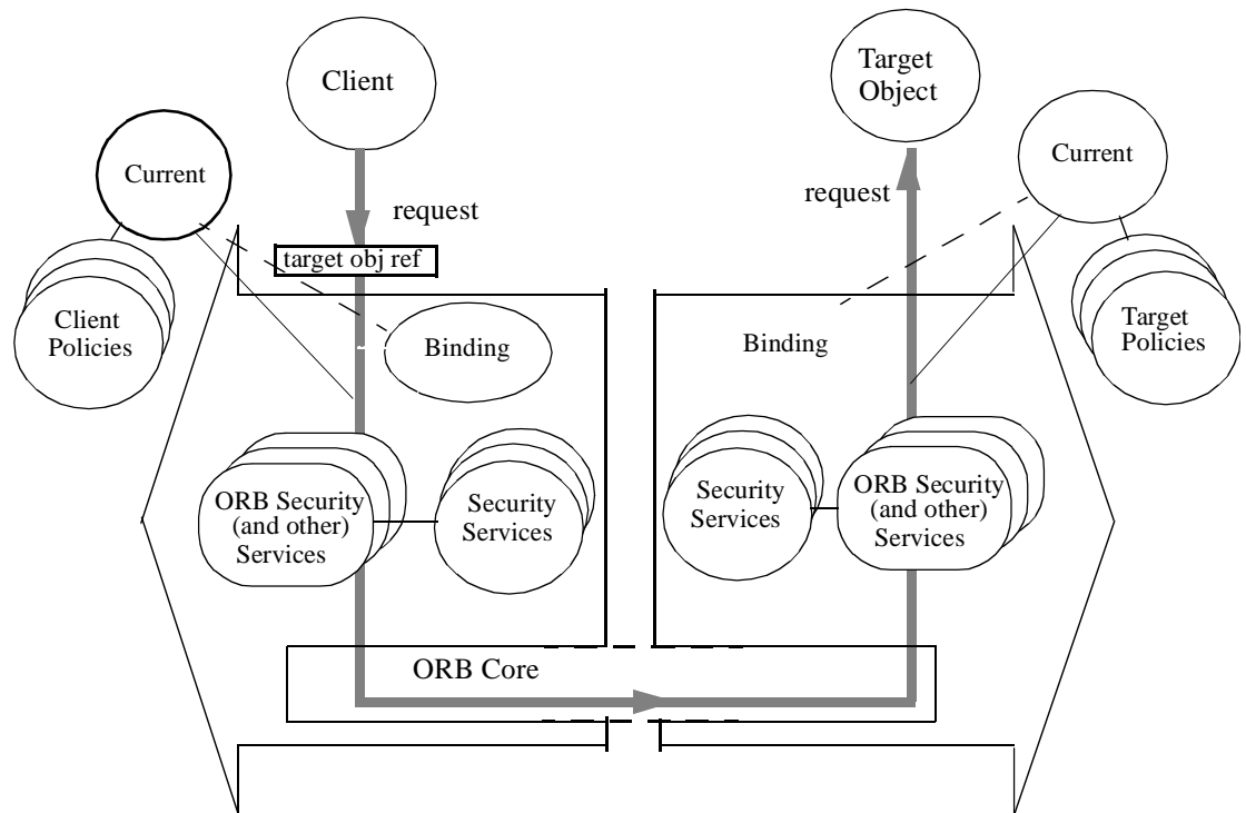
Figure 2-45 Securing Invocations
