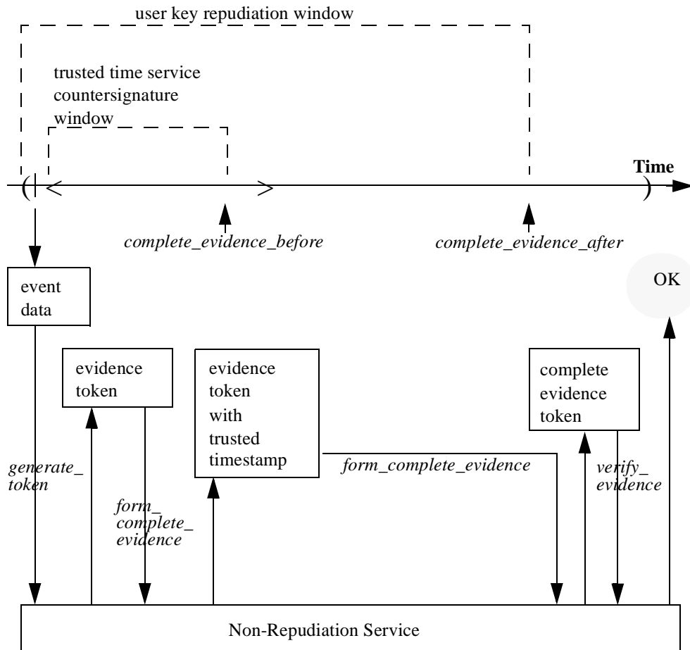
Figure 2-41 Non-repudiation Service
