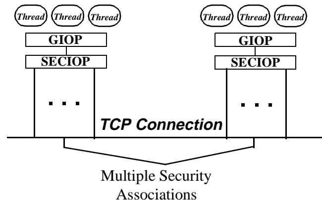
Figure 3-6 Architectural Assumptions
