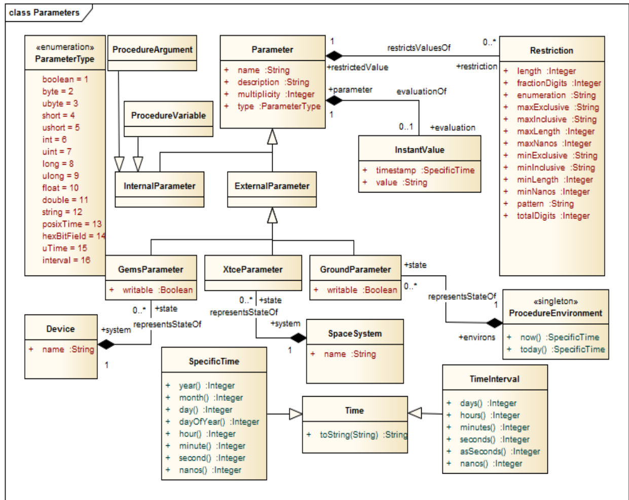
Figure 11: GEMS and XTCE Parameters
