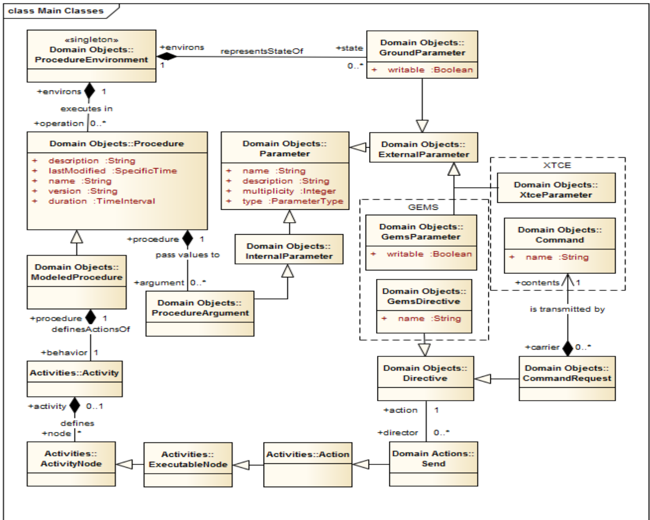
Figure 5: Key SOLM Classes
