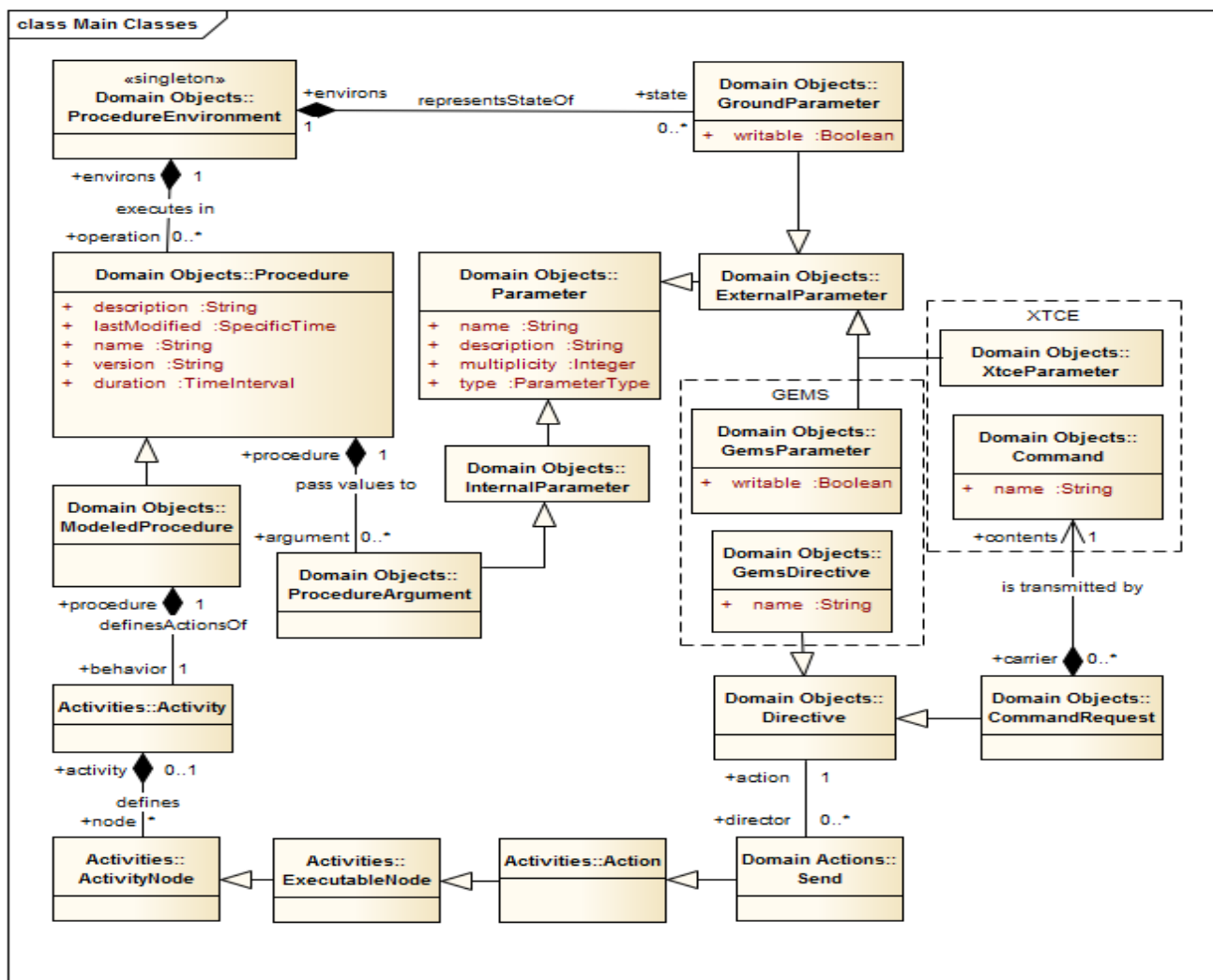
Figure 5 is an overview of the key classes and relationships for SOLM. Each of the following sections will provide subset of the model and descriptions and semantics for the classes. All classes in SOLM are presented as UML in this document, but the normative metamodel is provided as a MOF XMI file. The classes outlined with the dashed XTCE and GEMS box represent classes that will be instantiated from XTCE and GEMS definitions by the SOLM modeling environment.
