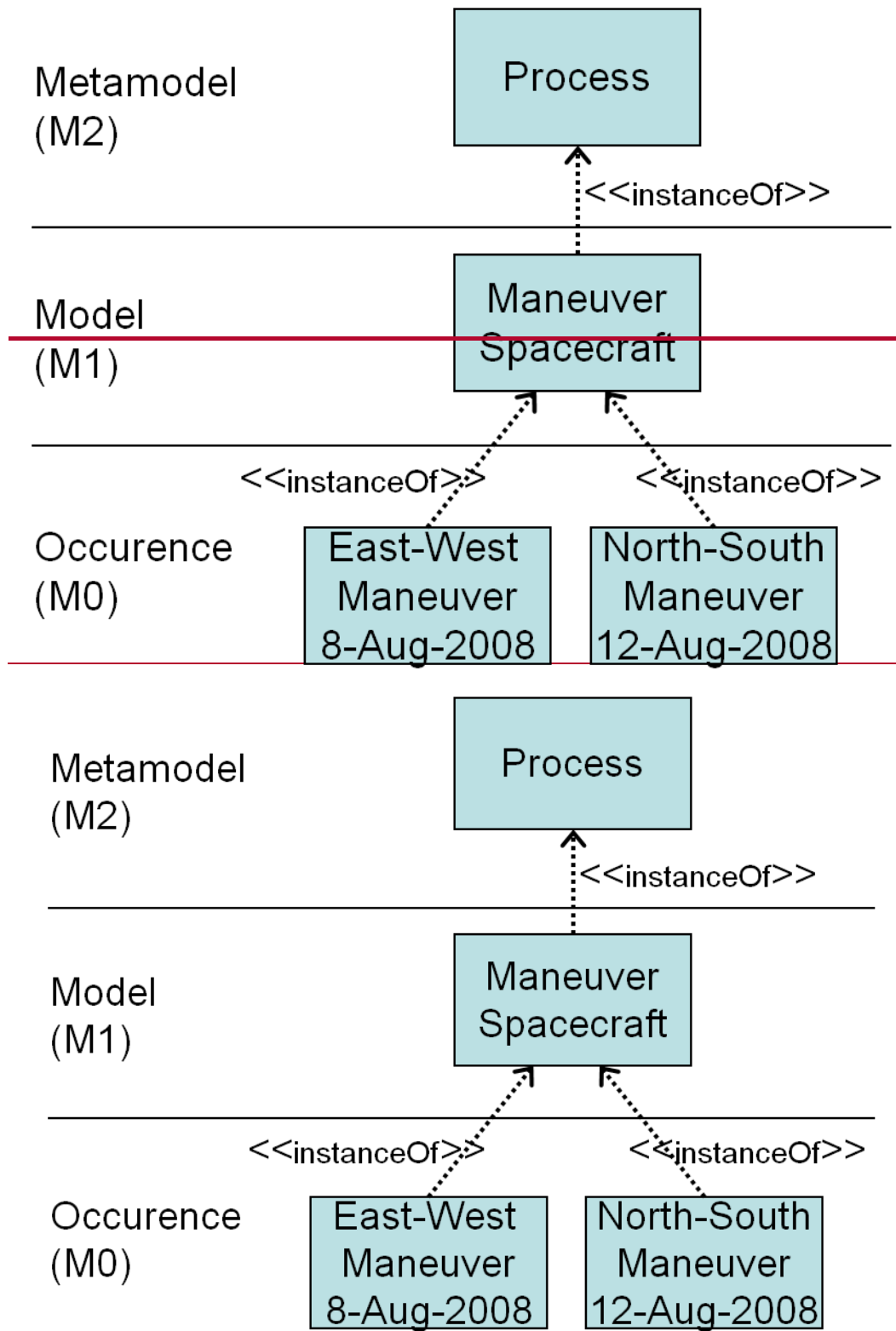
Figure 2: Process Modeling
