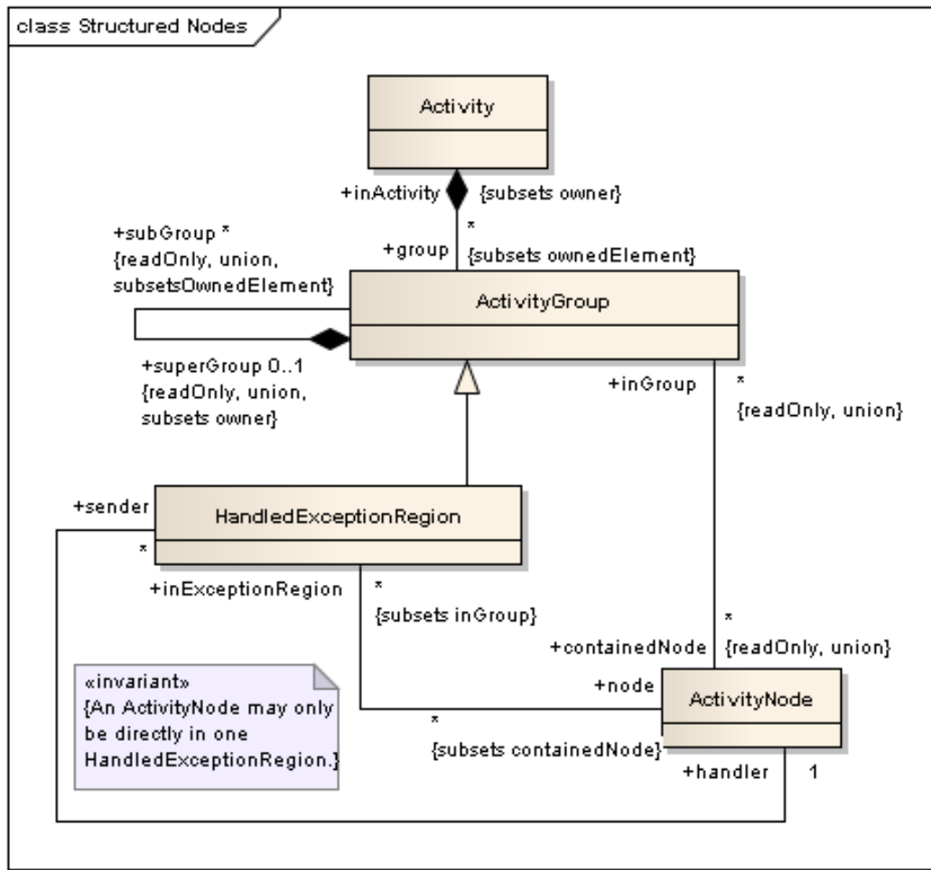
Figure 10: Exception Handling
