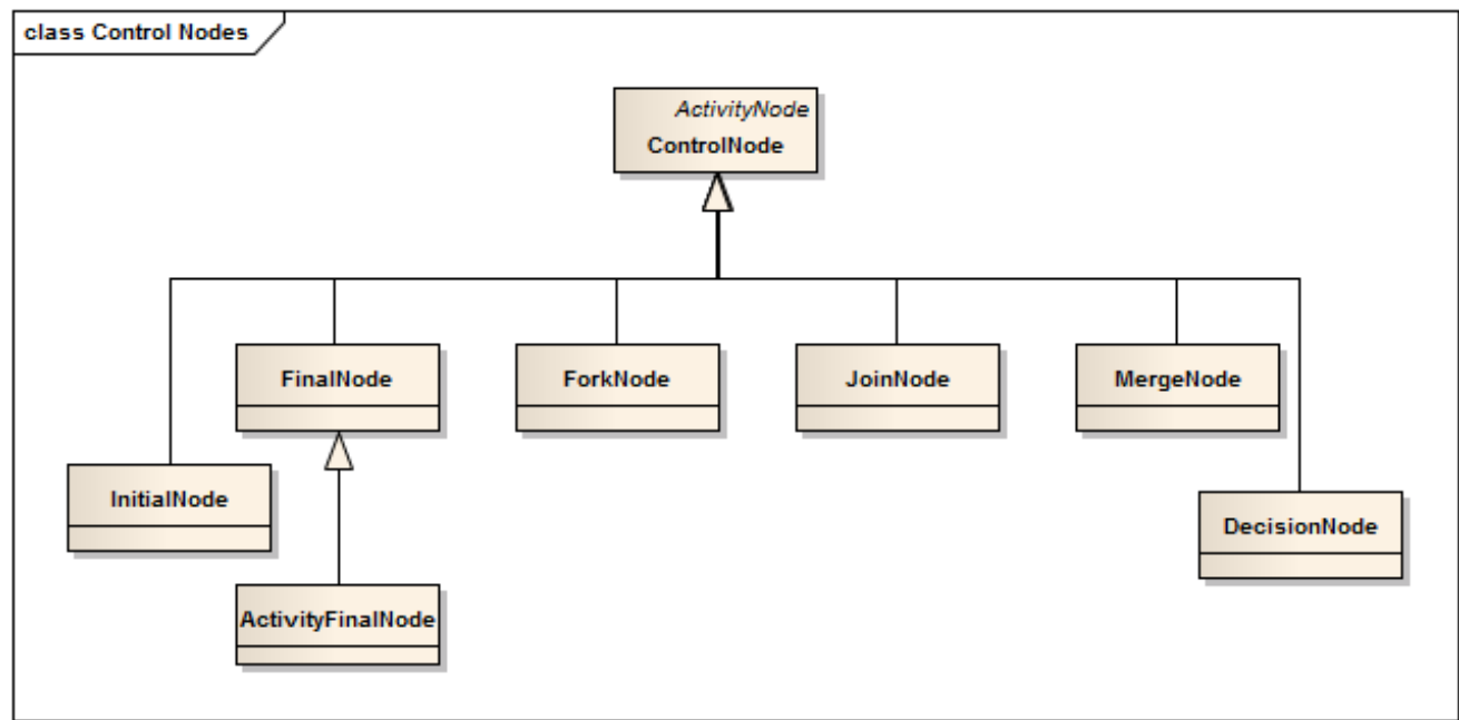
Figure 8: Control Nodes
