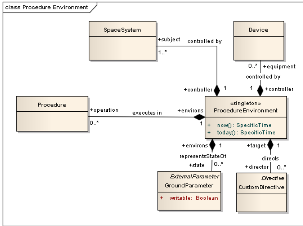
Figure 12: Procedure Environment
