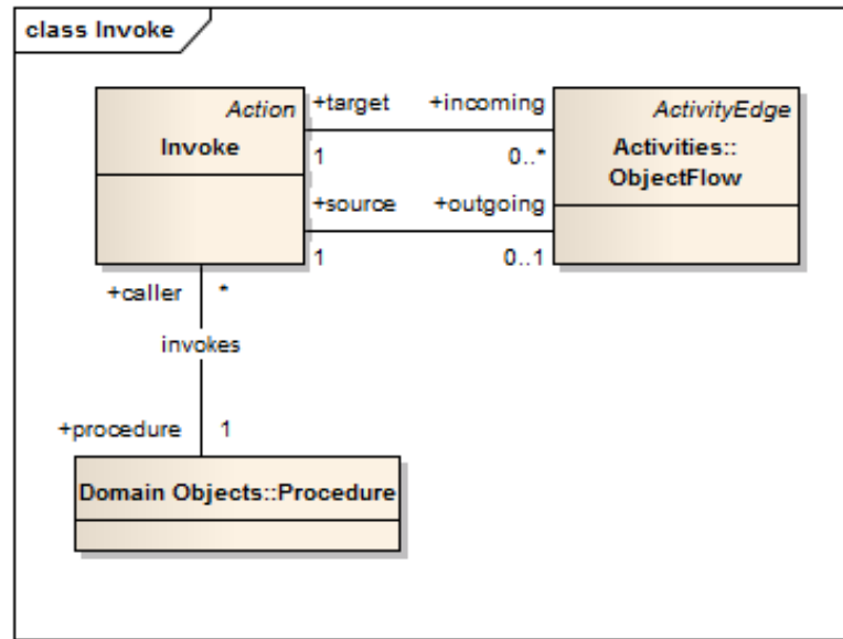
Figure 15: Invoke Subprocedure
