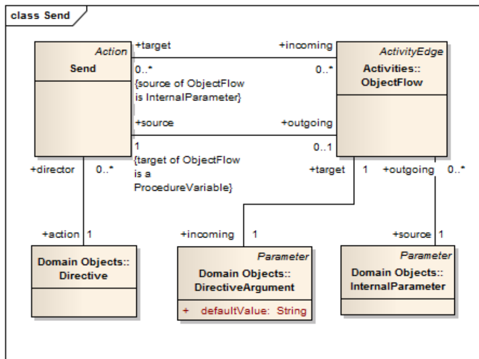
Figure 19: Send Directive
