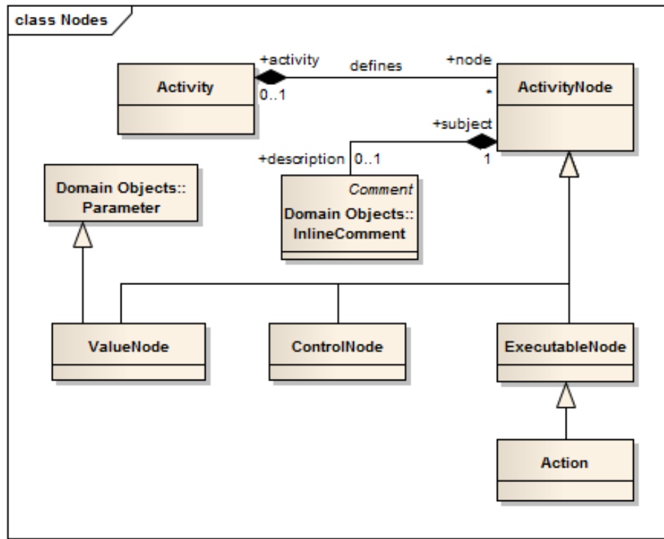
Figure 7: Activities
