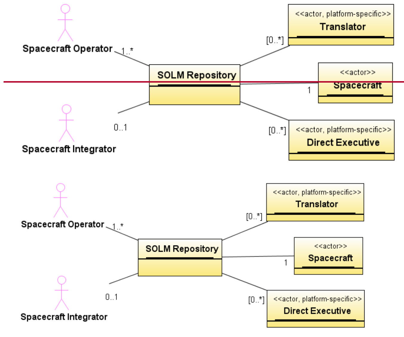
Figure 1: SOLM Context
