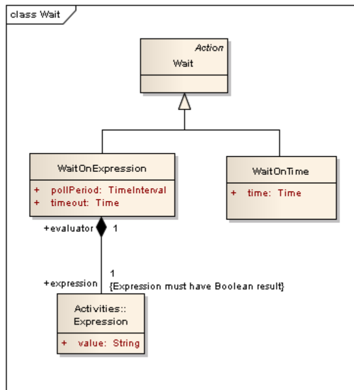
Figure 21: Wait
