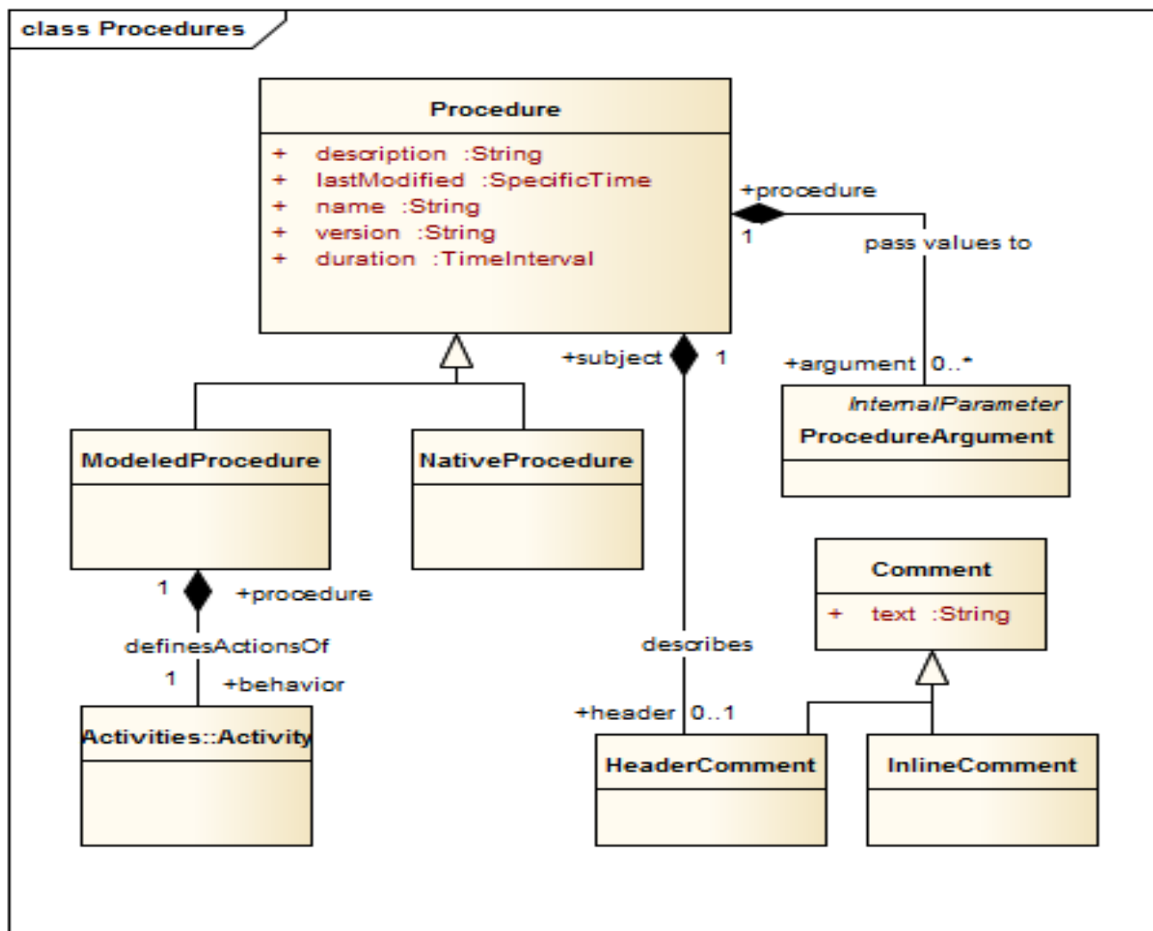
Figure 6: Procedure Signatures
