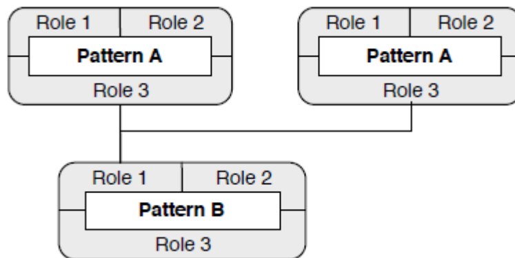
Figure 19: Multiple instances of the same pattern
