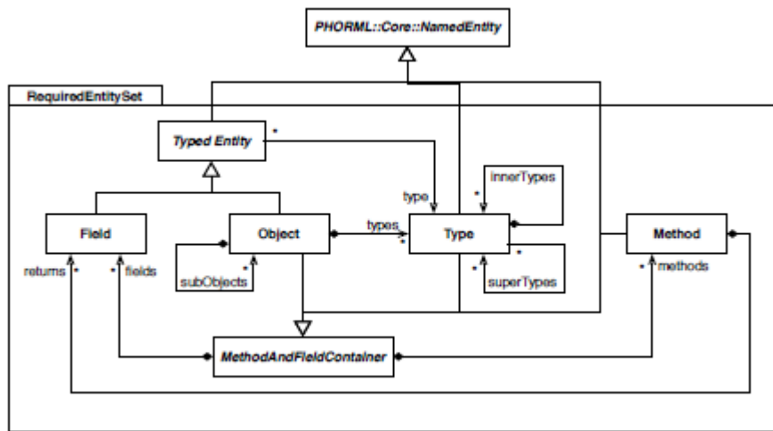
Figure 27: Required Entity Set
