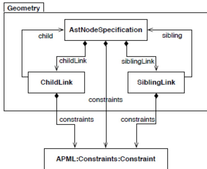
Figure 32: Geometry Package Diagram
