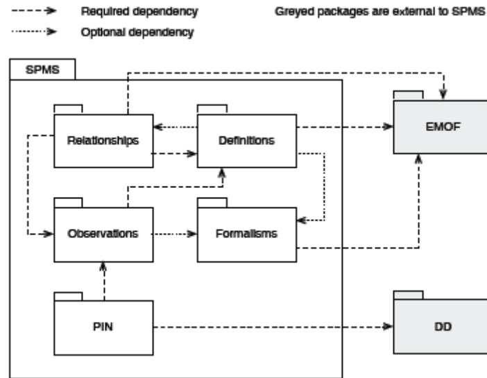
Figure 1: SPMS Metamodels Overview - Normative Packages
