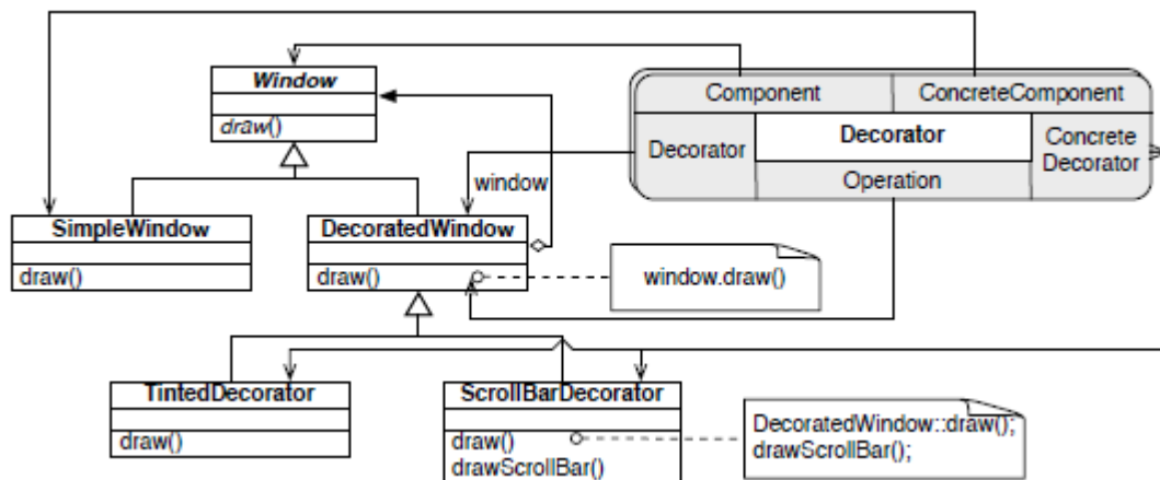
Figure 16: BindingGlyph used to bind to single Decorator instance to UML Class diagram
