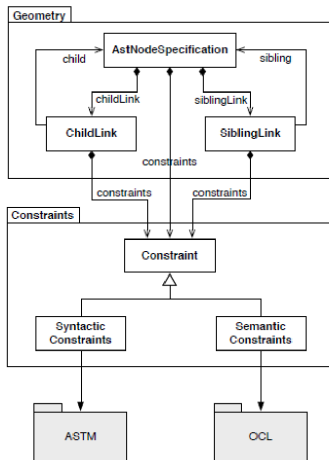
Figure 31: High Level (Composite) Diagram
