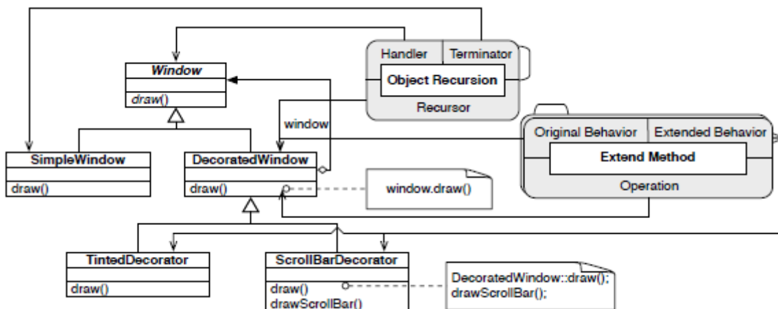
Figure 24: Peeled Decorator instances
