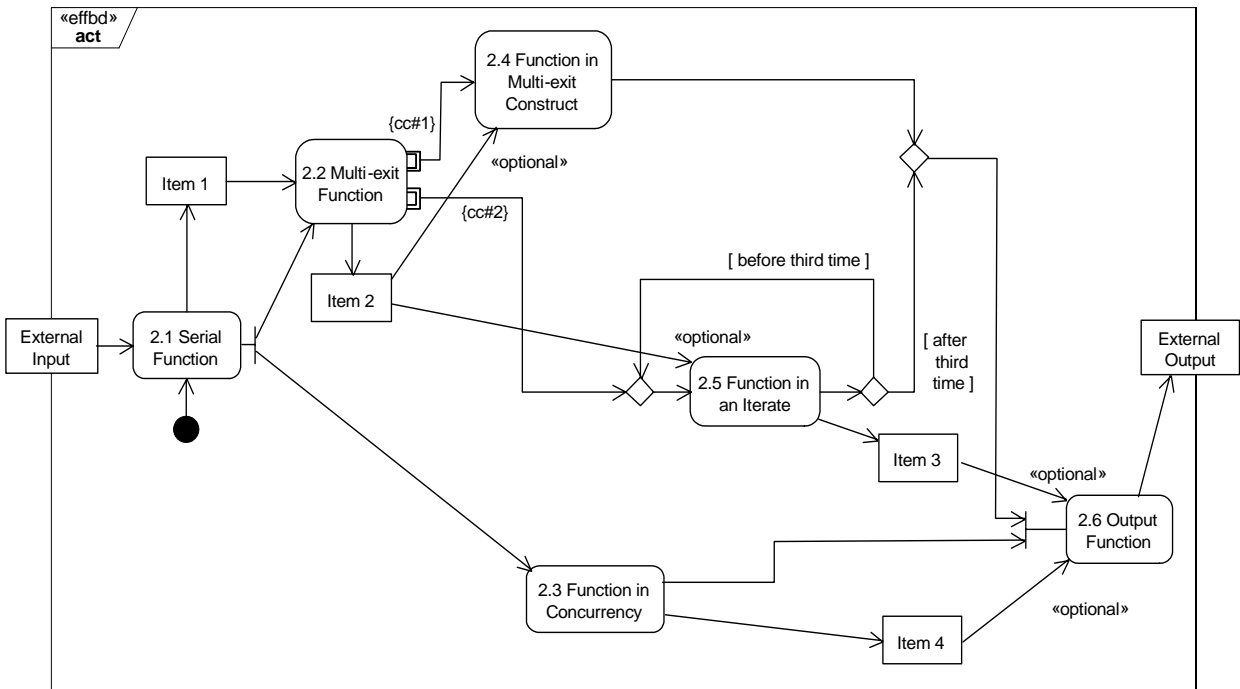
Figure C.1- Example activity with «effbd» stereotype applied
