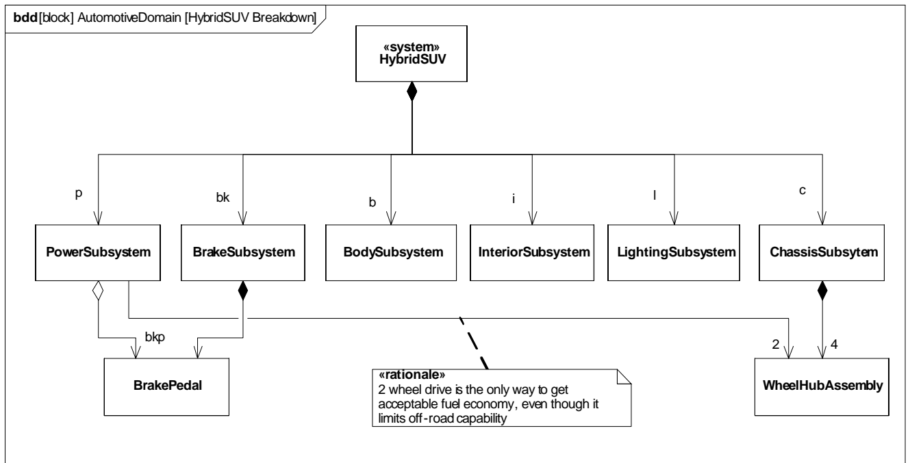
Figure B.16 - Defining Structure of the Hybrid SUV System (Block Definition Diagram)
