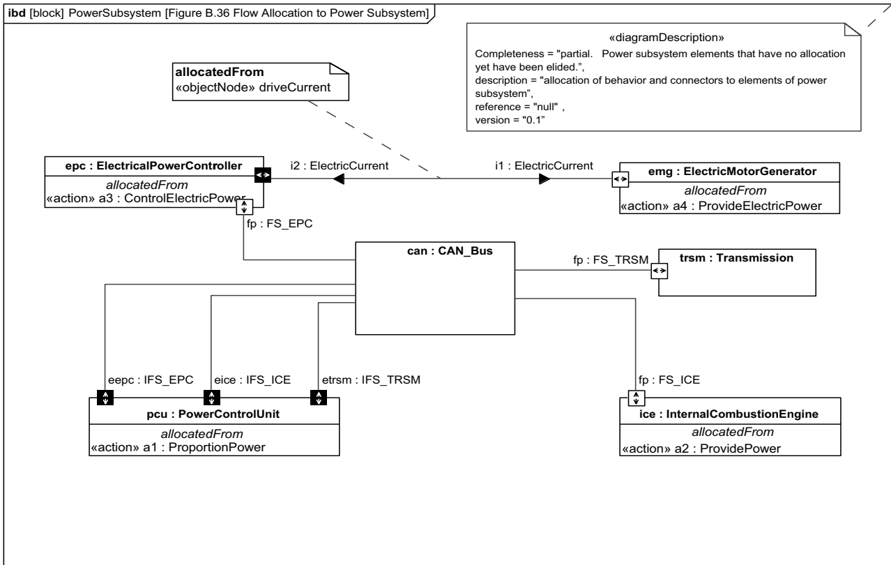
Figure B.36 - Flow Allocation to Power Subsystem (Internal Block Diagram)
