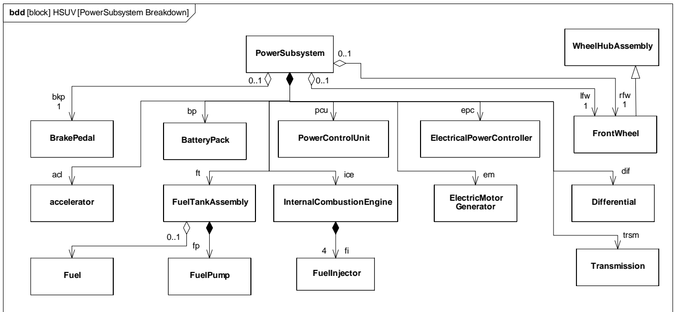
Figure B.18 - Defining Structure of Power Subsystem (Block Definition Diagram)
