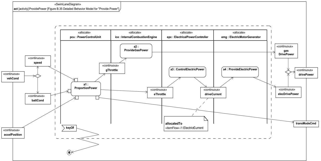
Figure B.35 - Detailed Behavior Model for "Provide Power" (Activity Diagram) Note hierarchical consistency with Figure B.33.
