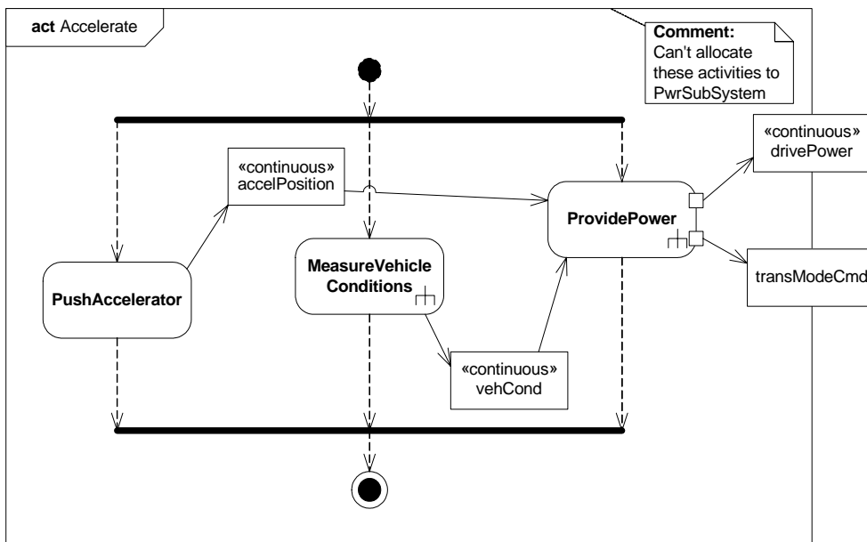
Figure B.33 - Behavior Model for "Accelerate" Function (Activity Diagram)
