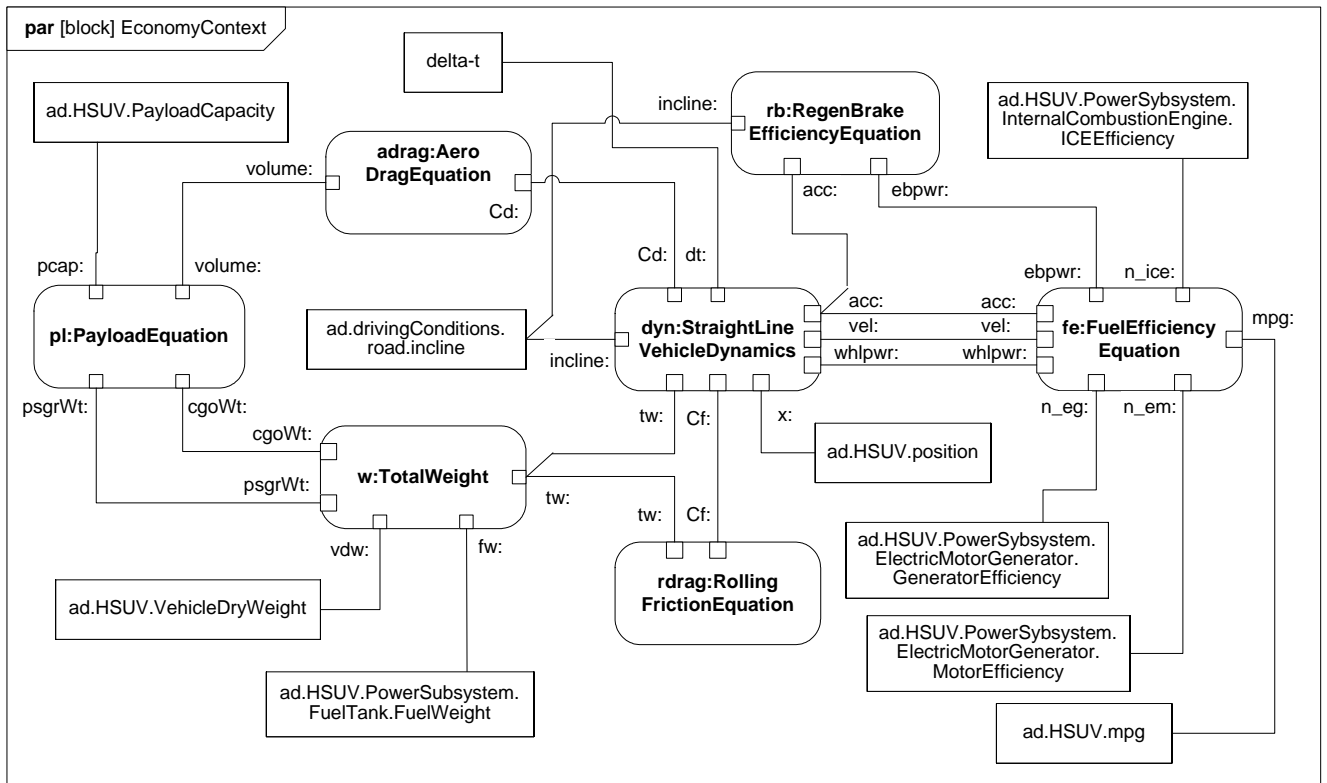
Figure B.29 - Establishing Mathematical Relationships for Fuel Economy Calculations (Parametric Diagram)
