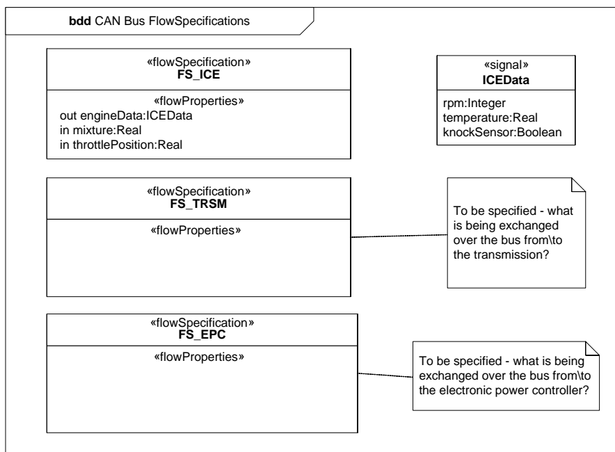
Figure B.21 - Initially Defining Flow Specifications for the CAN Bus (Block Definition Diagram)
