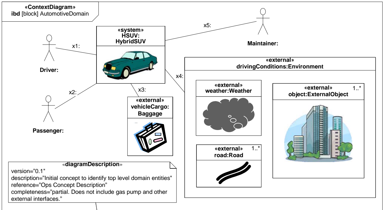
Figure B.4 - Establishing the Context of the Hybrid SUV System using a User-Defined Context Diagram. (Internal Block Diagram) Completeness of Diagram Noted in Diagram Description
