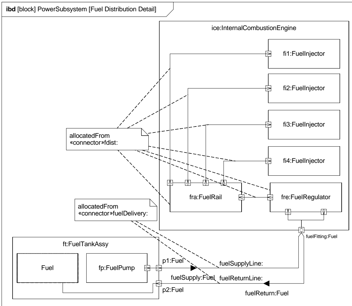
Figure B.25 - Detailed Internal Structure of Fuel Delivery Subsystem (Internal Block Diagram)
