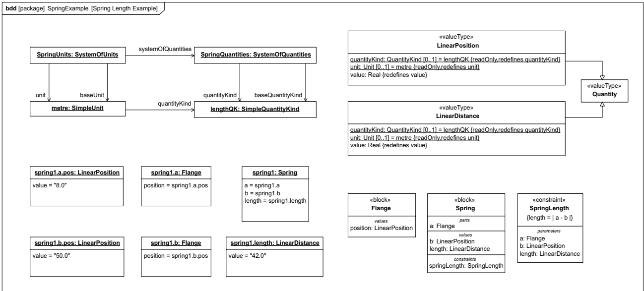
Figure C.13 - Spring Length Example
