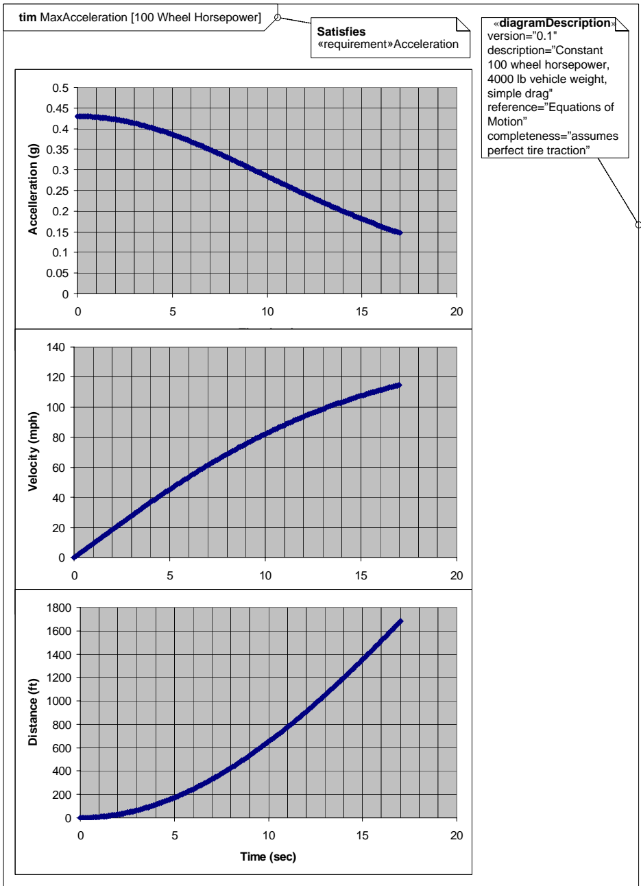
Figure B.32 - Results of Maximum Acceleration Analysis (Timing Diagram)
