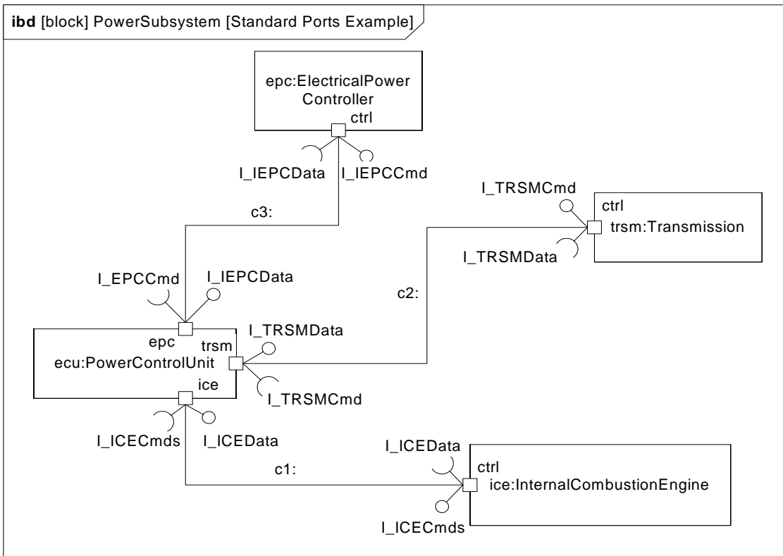
Figure 9.3 - Usage example of standard ports
