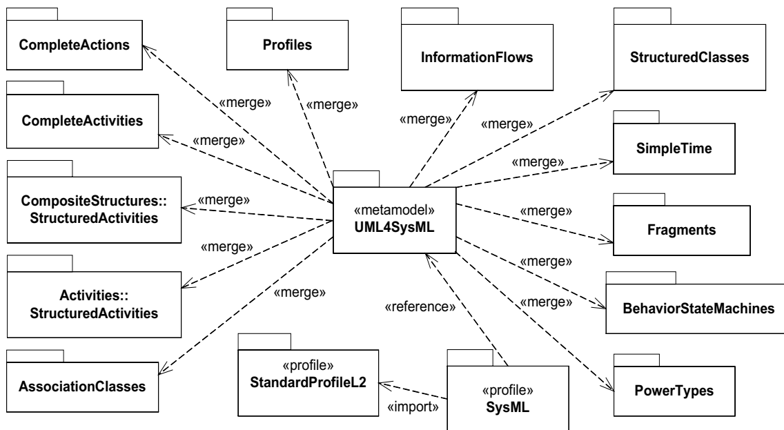
Figure 4.2 - SysML Extension of UML
