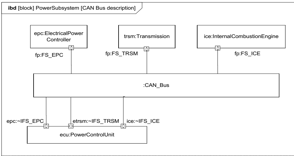
Figure B.22 - Consolidating Interfaces into the CAN Bus. (Internal Block Diagram)
