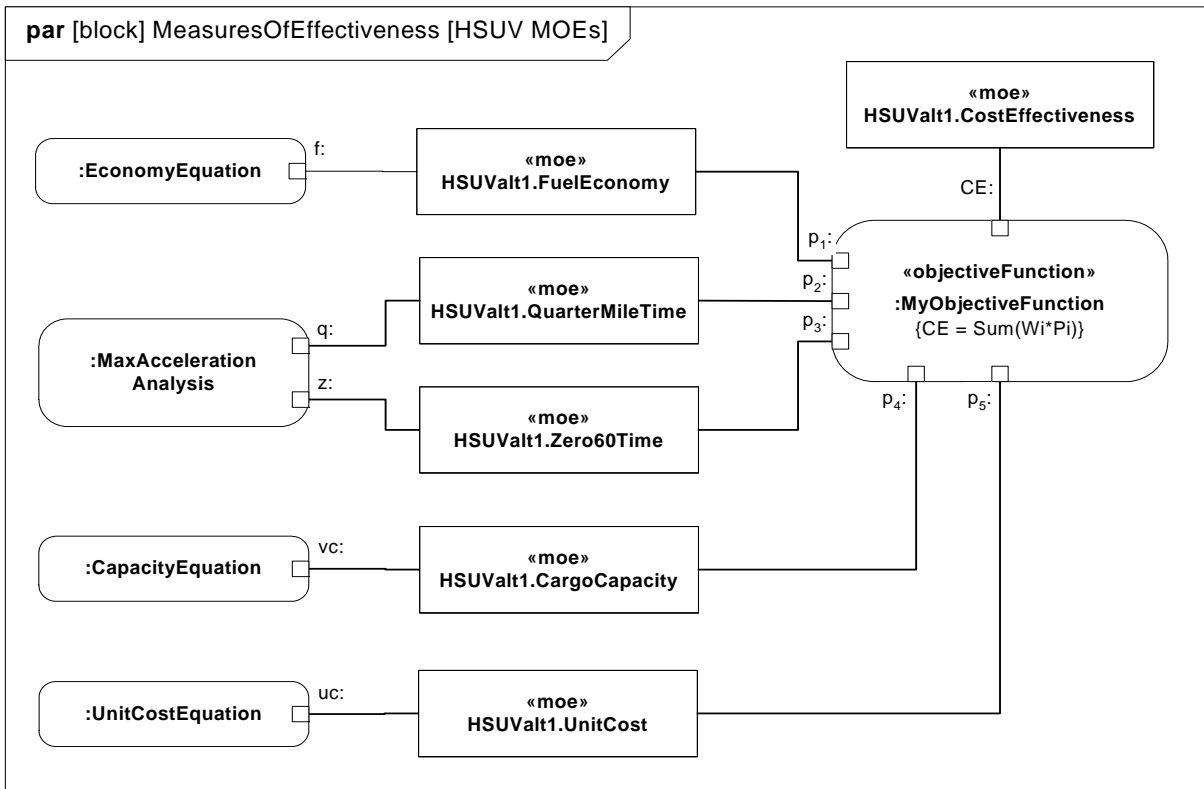
Figure C.28 - Defining Measures of Effectiveness and Key Relationships (Parametric Diagram)
