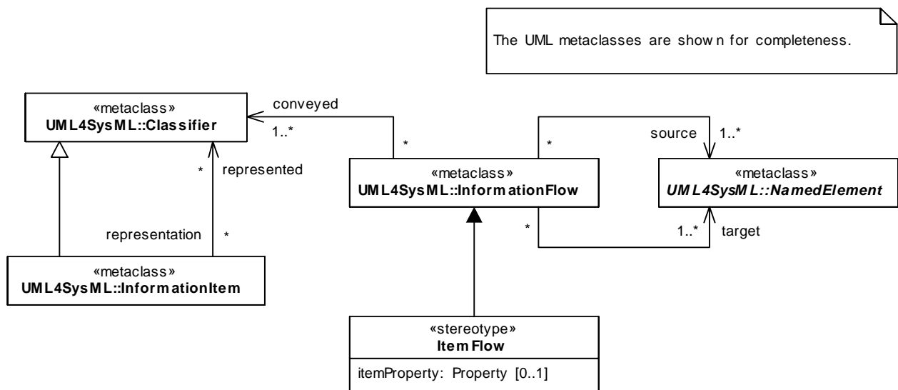
Figure 9.5 - ItemFlow Stereotype
