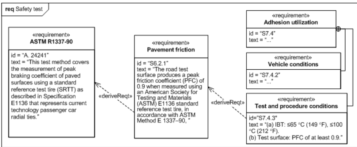
Figure 16.3 - Requirements Derivation
