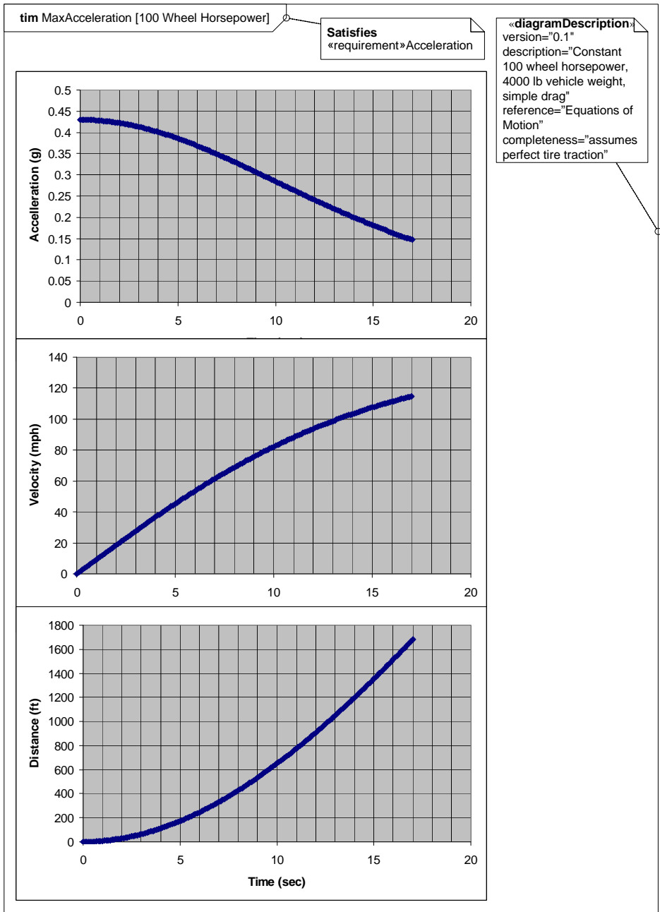
Figure C.32 - Results of Maximum Acceleration Analysis (Timing Diagram)
