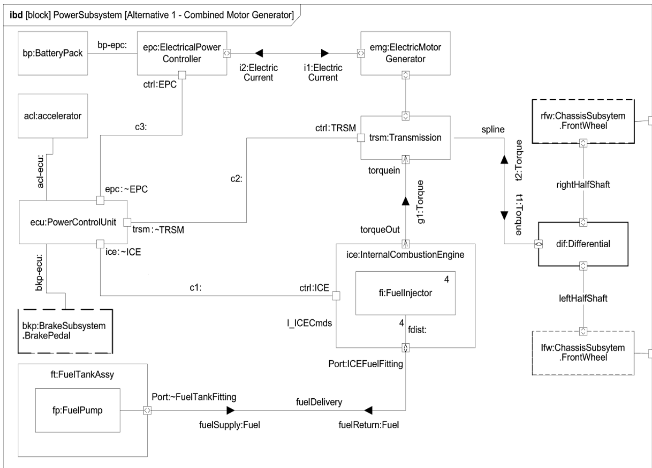
Figure C.19 - Internal Structure of the Power Subsystem (Internal Block Diagram)
