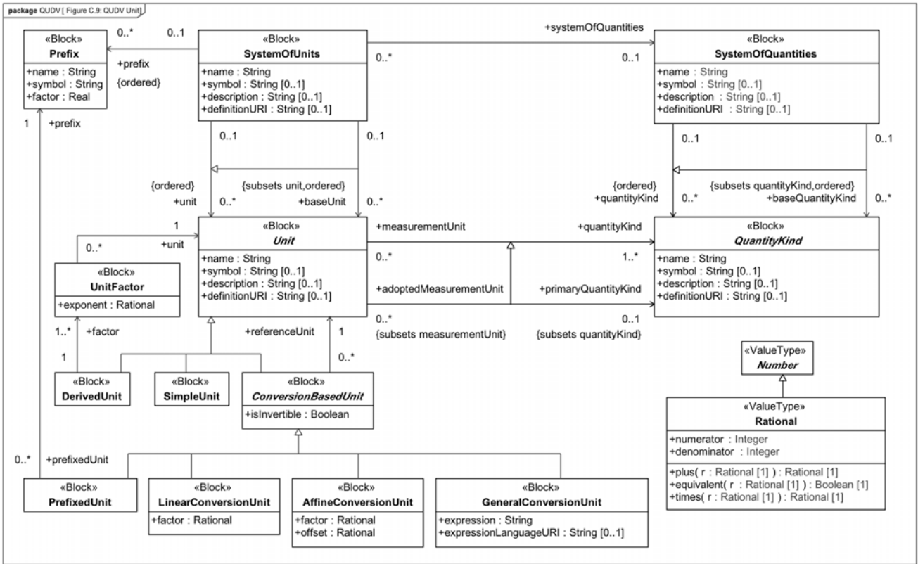
Figure D.9 - QUDV Unit diagram
