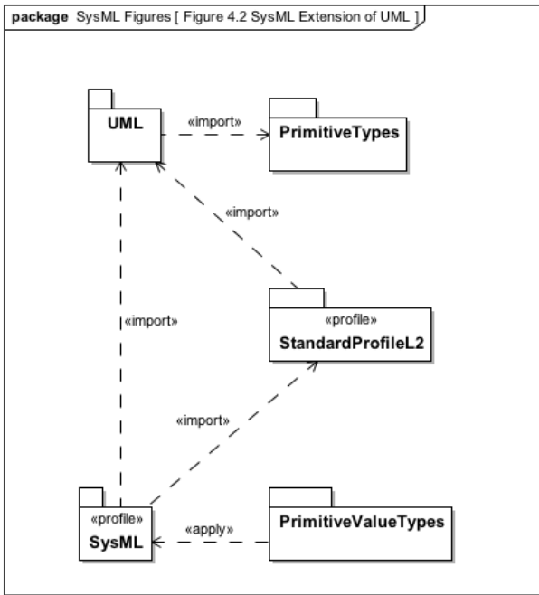
Figure 4.2 - SysML Extension of UML
