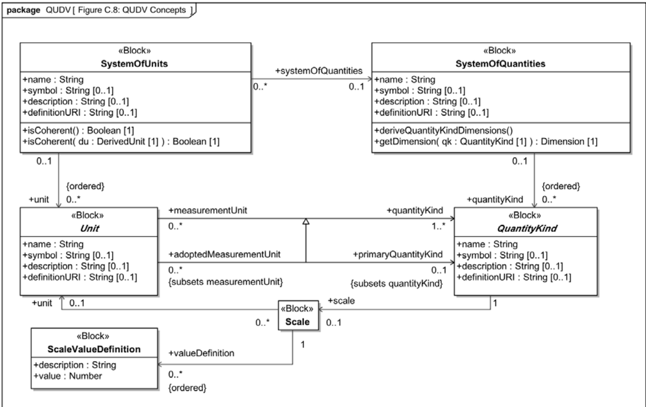
Figure D.8 - QUDV Concepts diagram
