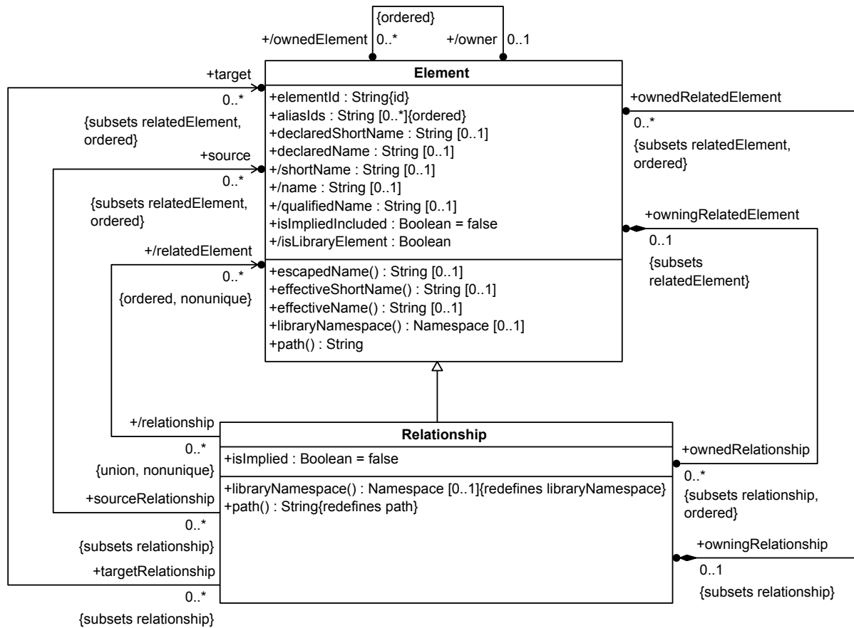
Figure 2. Elements
