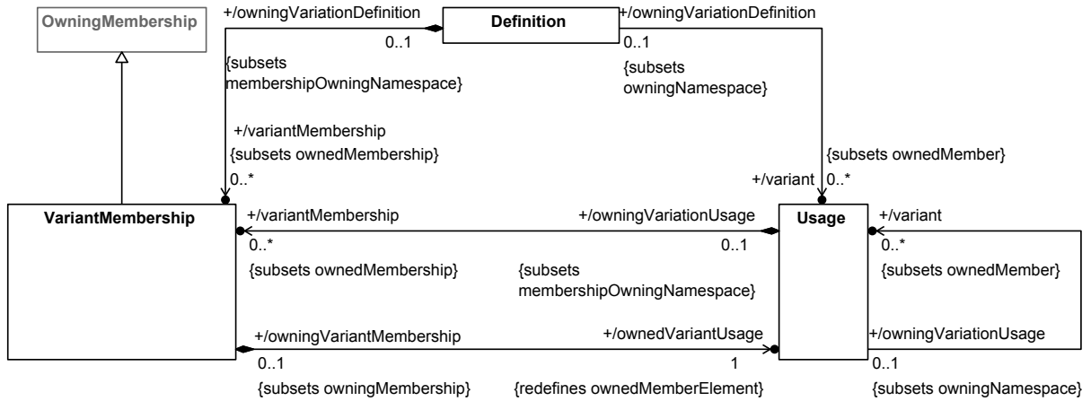
Figure 9. Variant Membership
