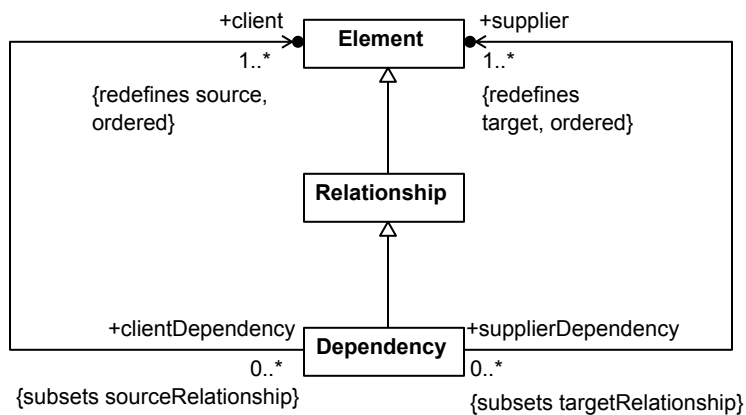
Figure 3. Dependencies
