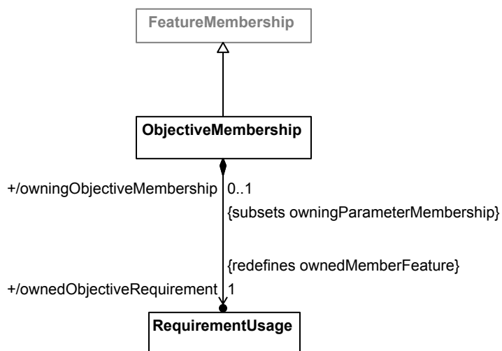
Figure 43. Case Membership
