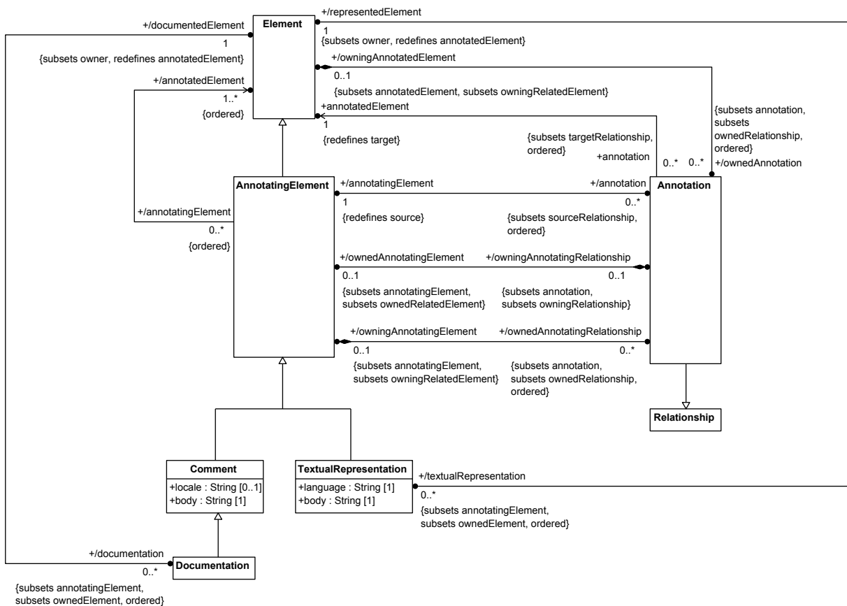
Figure 4. Annotation
