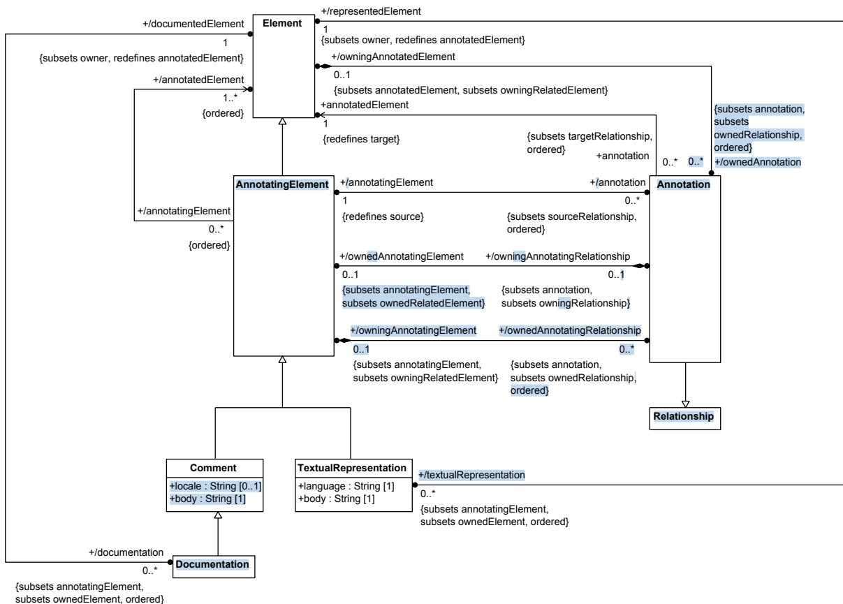
Figure 4. Annotation
