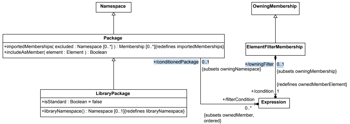
Figure 7. Packages
