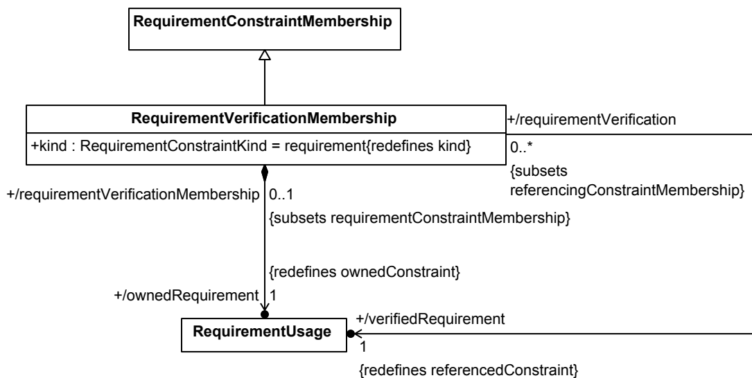
Figure 46. Verification Membership
