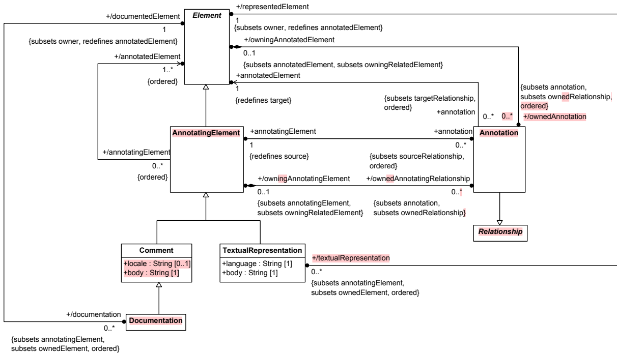
Figure 4. Annotation
