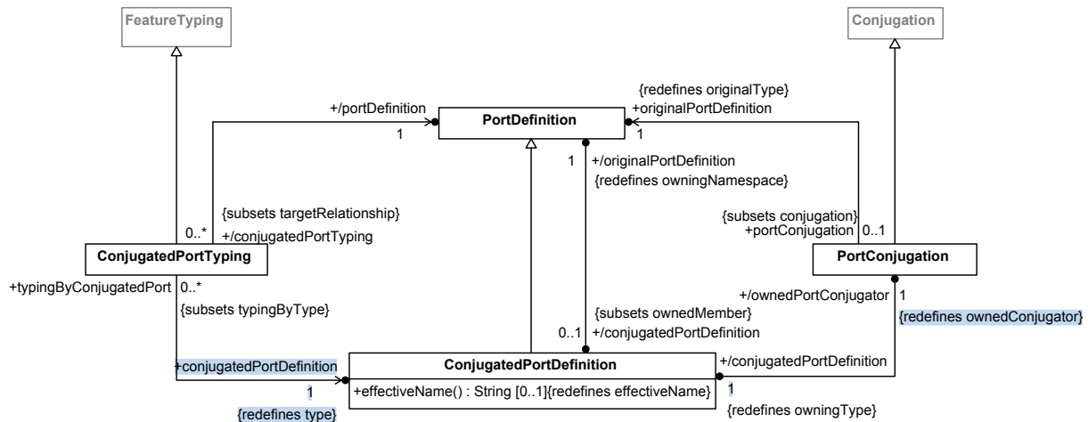
Figure 17. Port Conjugation
