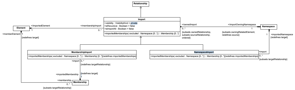
Figure 6. Imports
