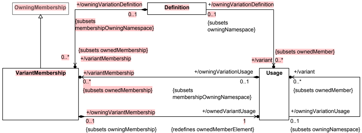
Figure 9. Variant Membership
