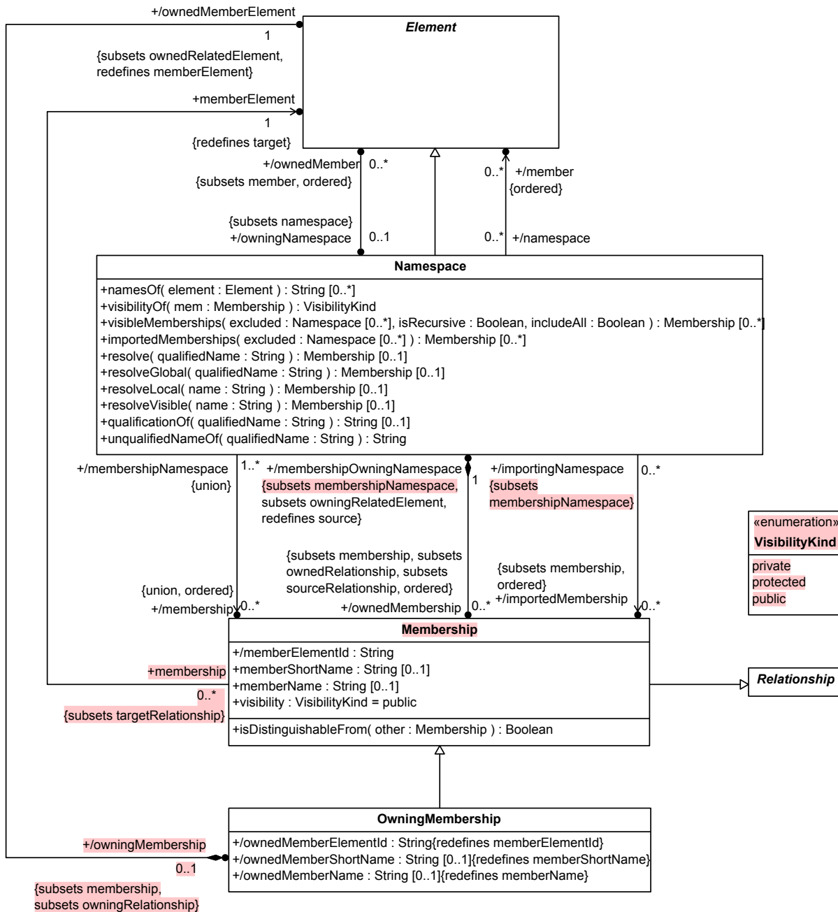
Figure 5. Namespaces
