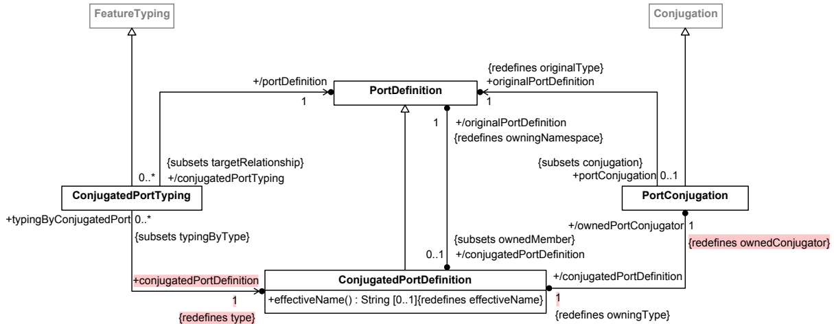
Figure 17. Port Conjugation
