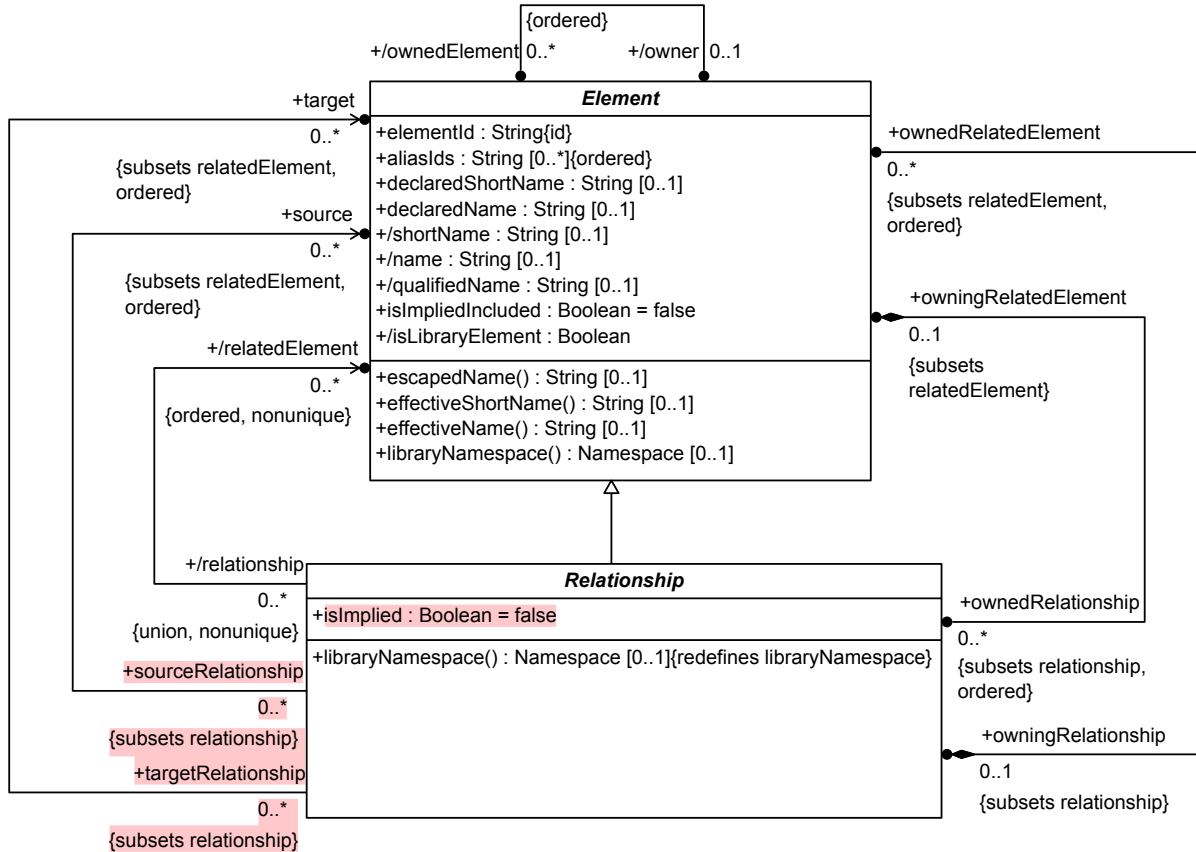
Figure 2. Elements
