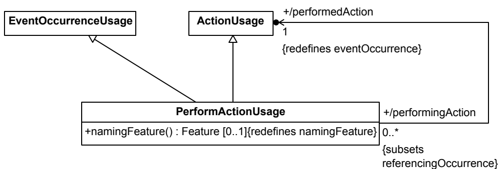
Figure 25. Performed Actions
