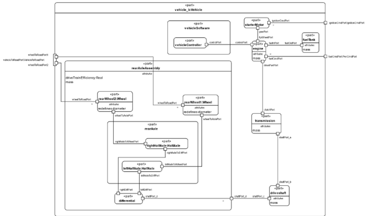
Figure 64. Parts Interconnection for vehicle_b
