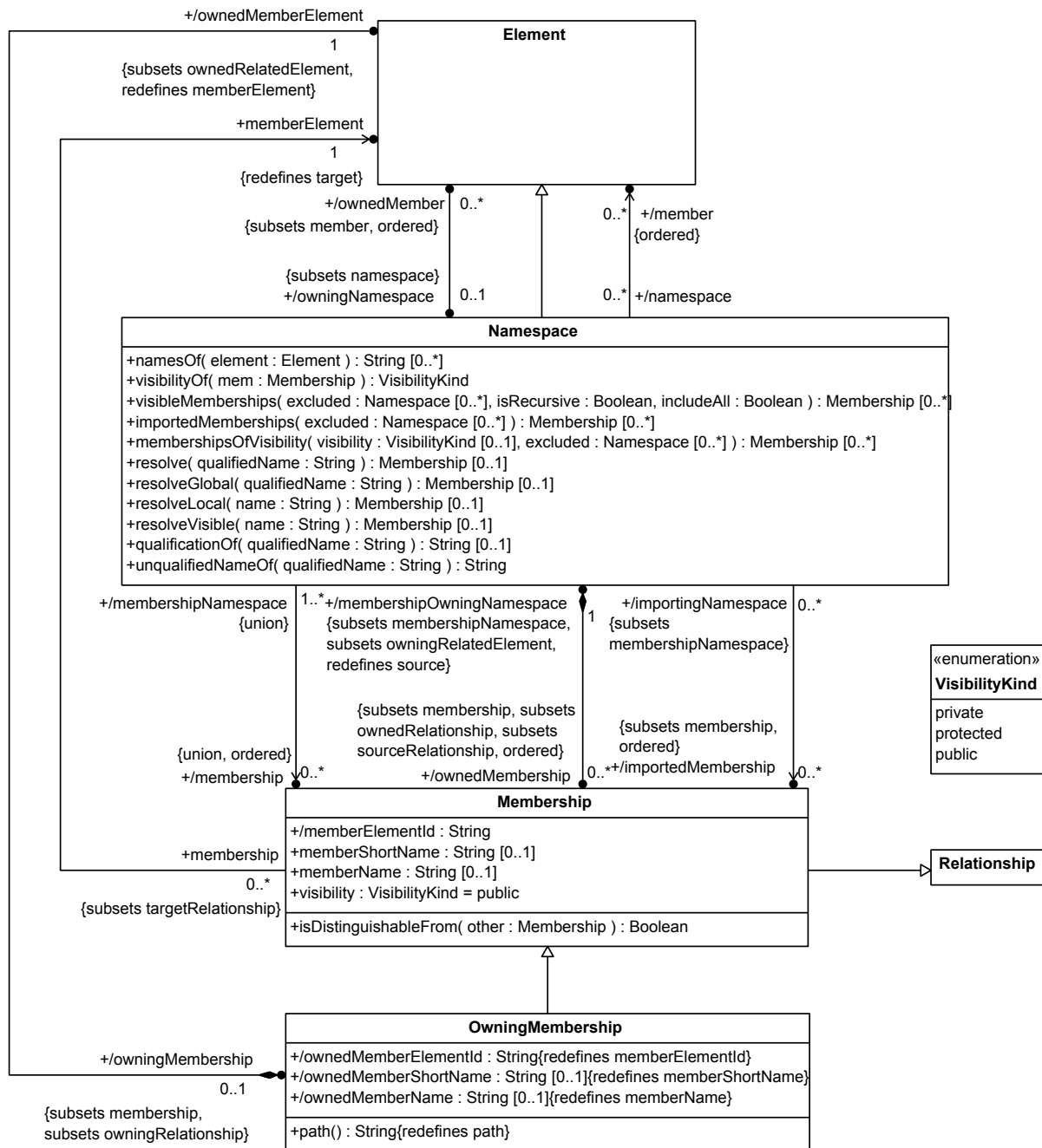
Figure 5. Namespaces
