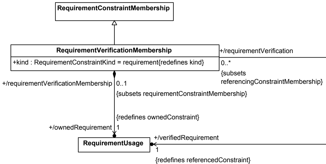
Figure 46. Verification Membership
