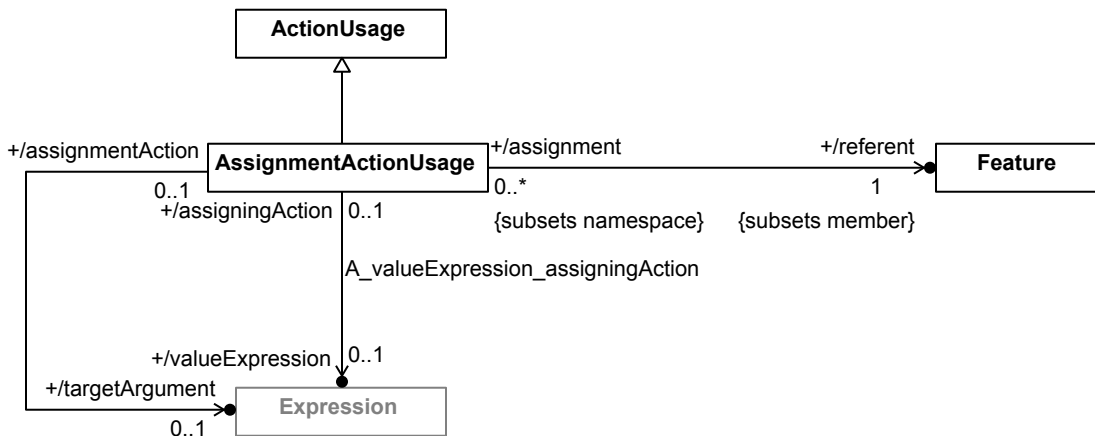
Figure 27. Assignment Actions
