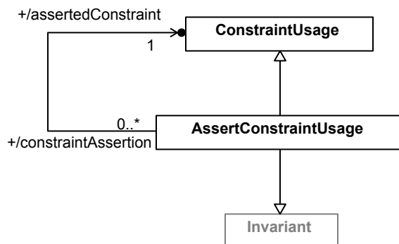
Figure 36. Asserted Constraints
