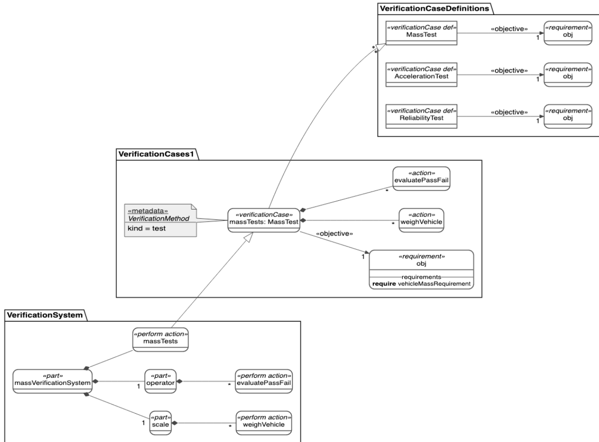
Figure 72. Vehicle Mass Verification Test
