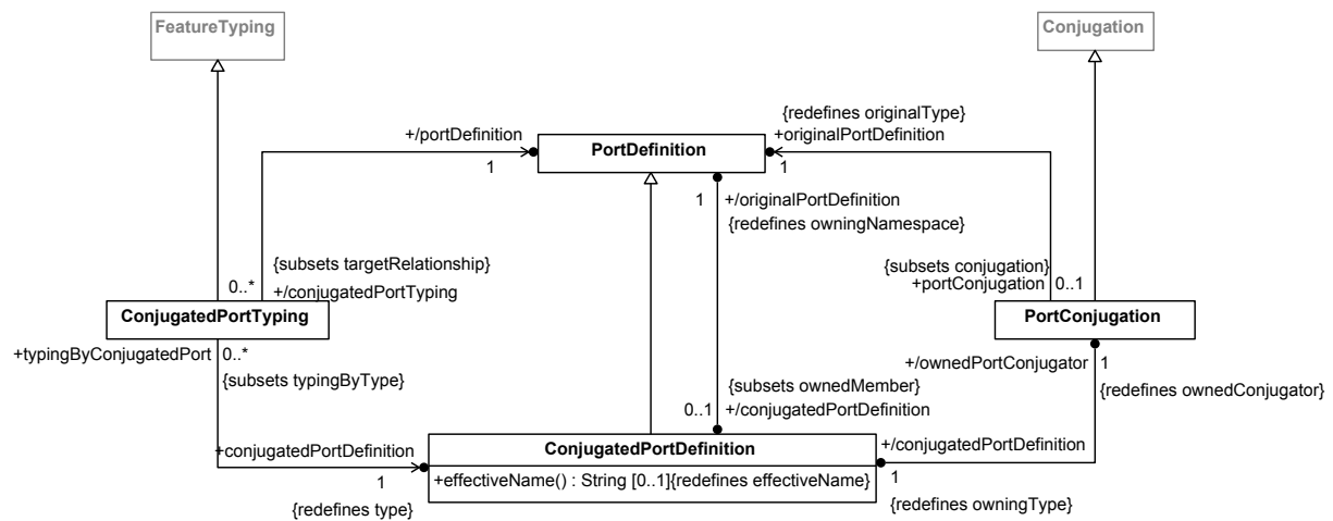
Figure 17. Port Conjugation
