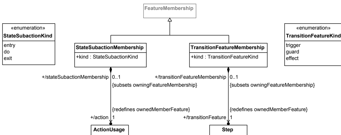
Figure 31. State Membership
