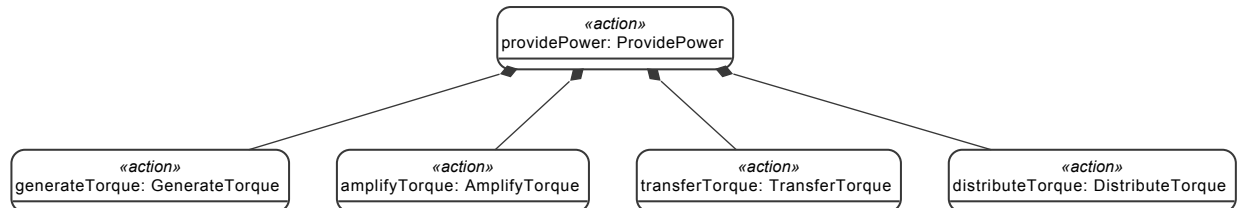
Figure 65. Action providePower
