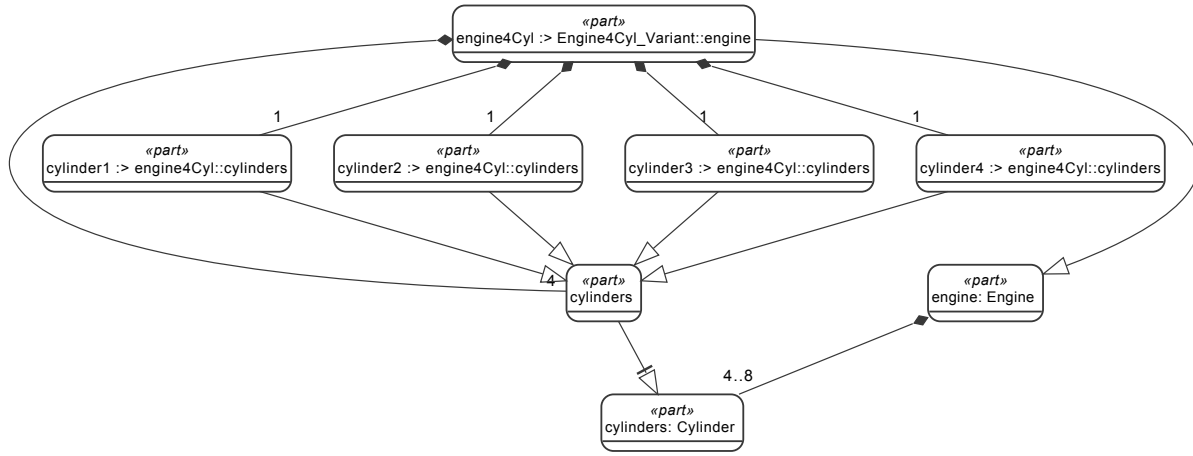
Figure 63. Variant engine4Cyl
