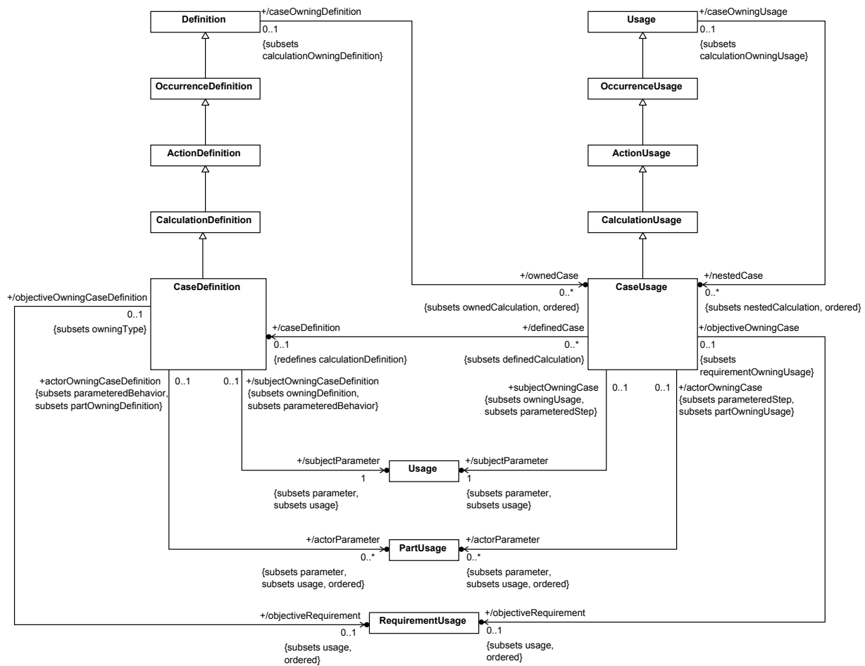
Figure 42. Case Definition and Usage
