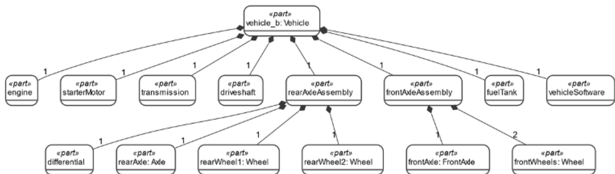
Figure 62. Parts Tree for vehicle_b
