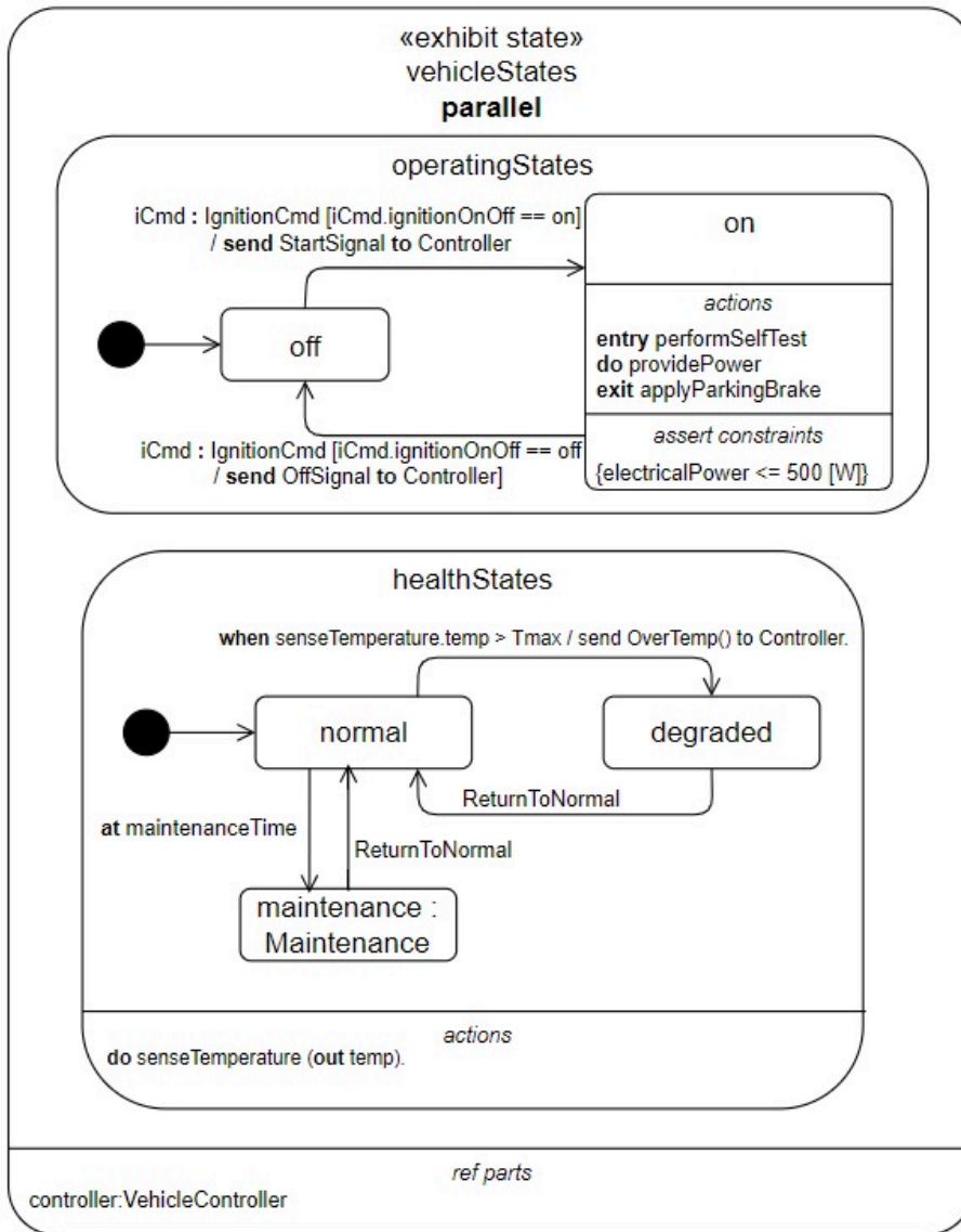
Figure 68. Vehicle States
