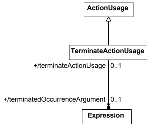
Figure 28. Terminate Actions
