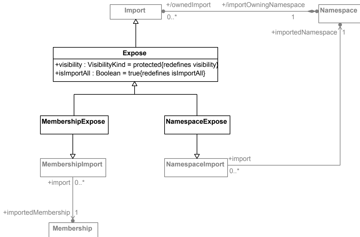
Figure 52. Expose Relationship
