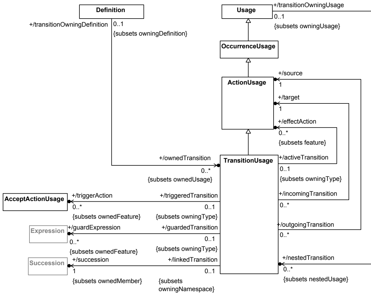
Figure 33. Transition Usage
