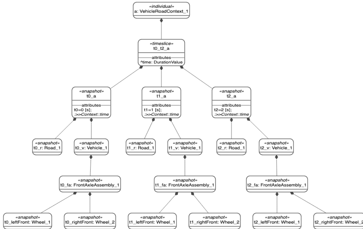
Figure 76. Vehicle Individuals and Snapshots
