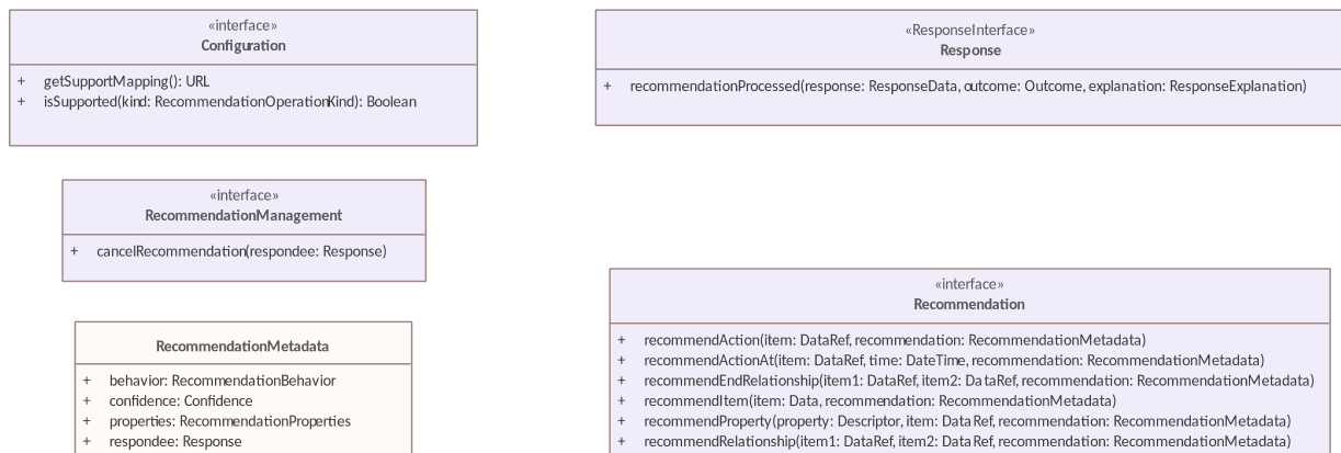
Figure 8.5 Recommendations (Class diagram)
