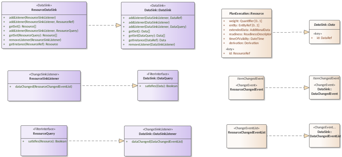
Figure 10.16 ResourceDataSink Realization (Class diagram)
