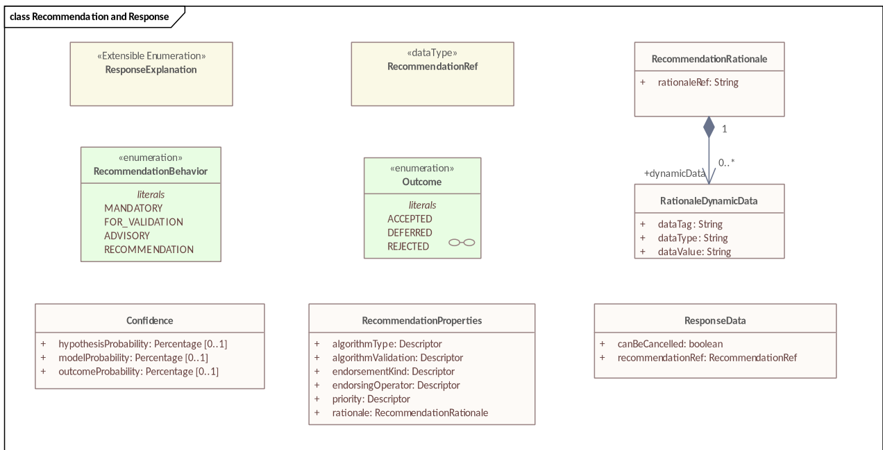
Figure 8.2 Recommendation and Response (Class diagram)
