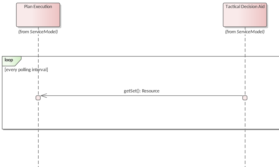
Figure 10.13 ResourceDataSink – All Resources – Polling (Interaction diagram)
