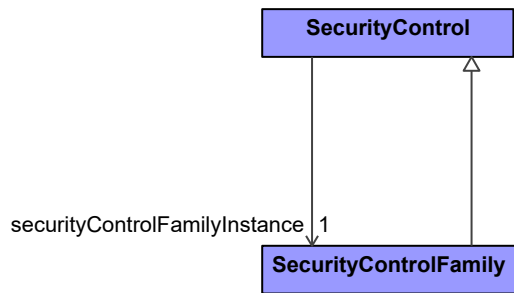
Figure 9-203: SecurityControlFamily
