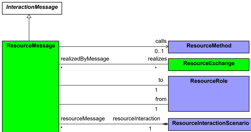
Figure 9-186: ResourceMessage
