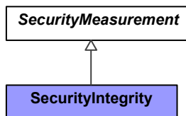
Figure 9-221: SecurityIntegrity
