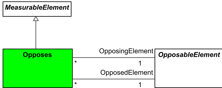
Figure 9-31: Opposes
