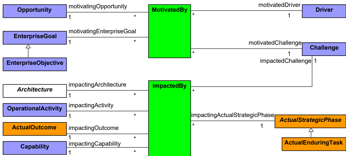
Figure 8-12: Strategic Motivation
