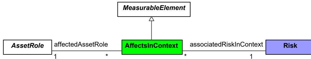
Figure 9-268: AffectsInContext
