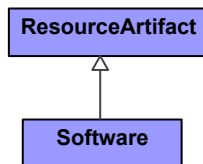
Figure 9-169: Software
