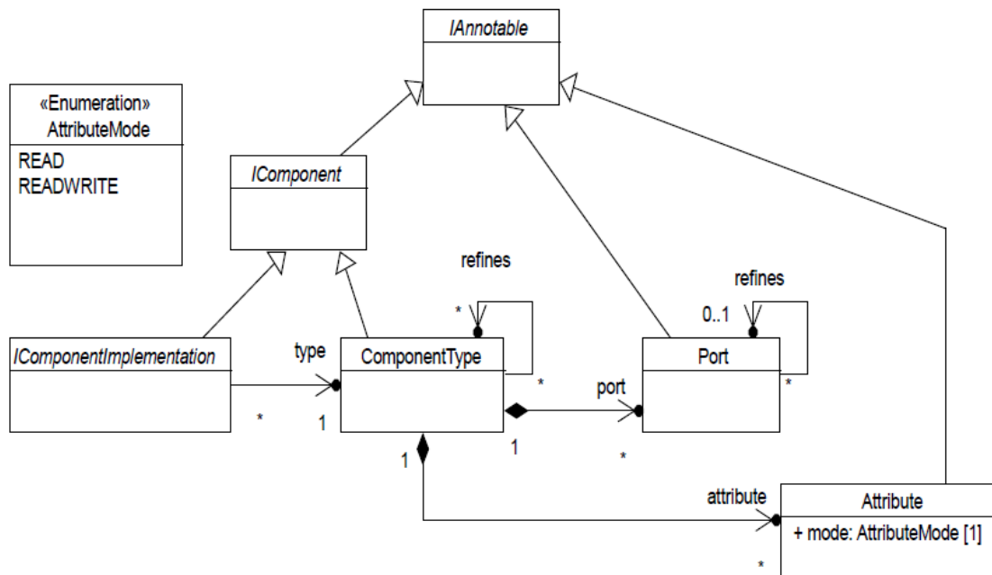
Figure 9.25 - UCM component types
