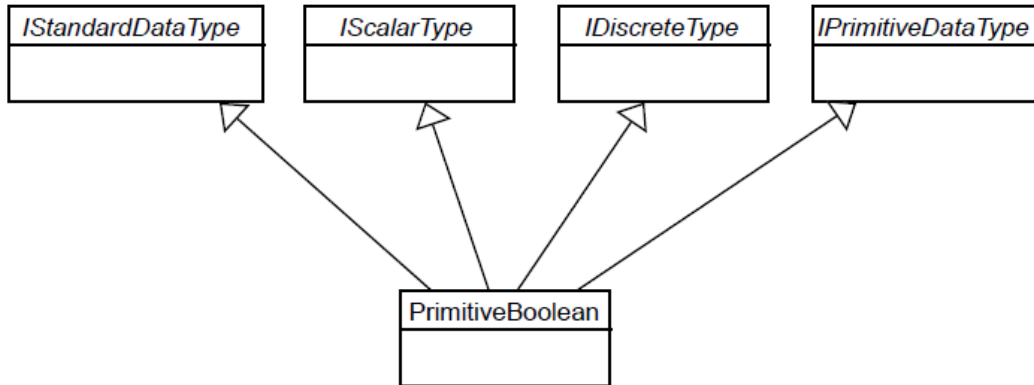
Figure 9.9 - UCM primitive boolean
