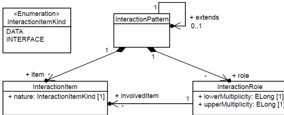
Figure 9.20 - UCM interaction patterns
