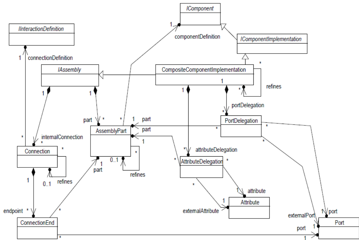
Figure 9.29 - UCM composite component implementations
