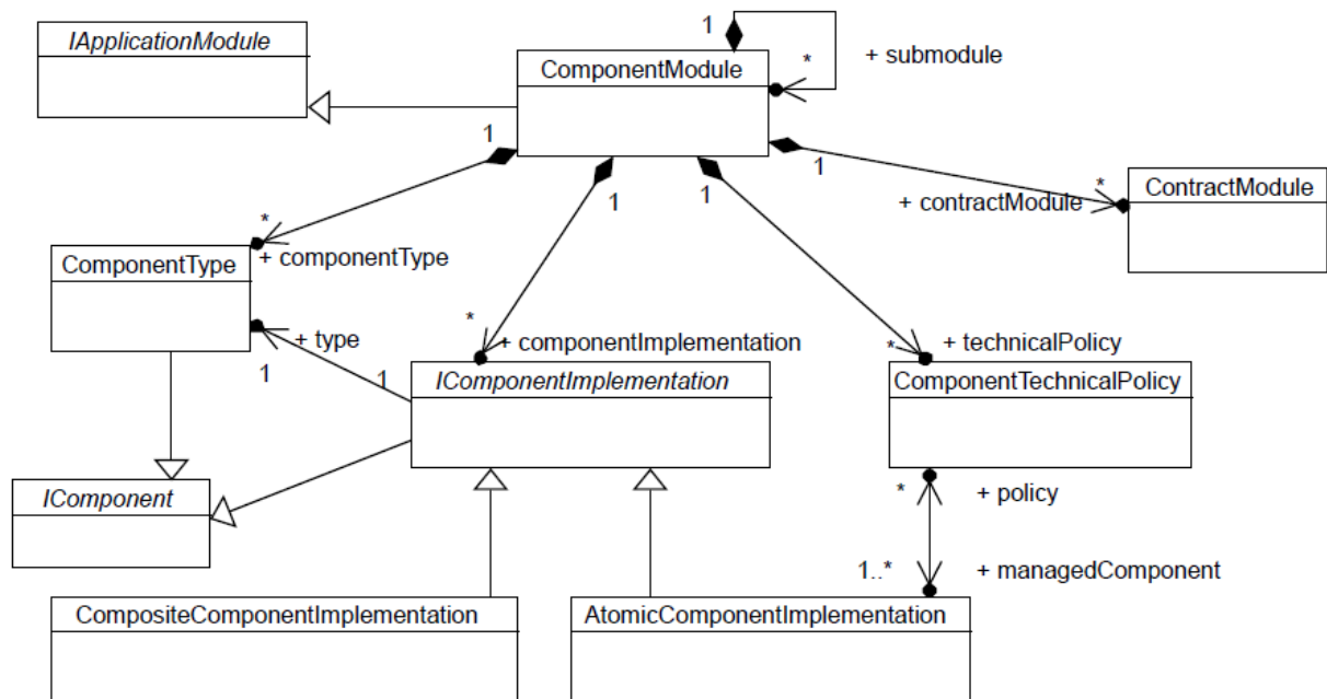
Figure 9.24 - Main classes involved in UCM component package
