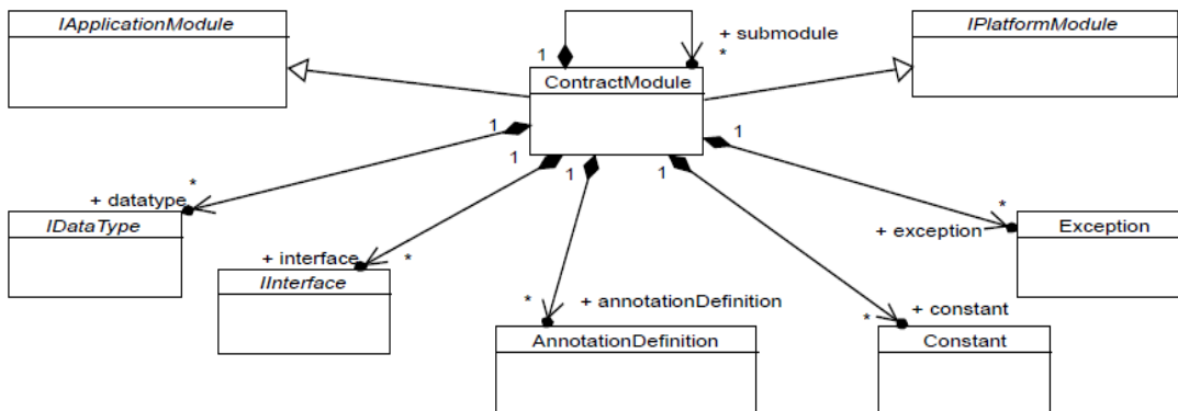
Figure 9.5 - UCM contract base declarations
