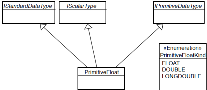
Figure 9.7 - UCM floating point numbers
