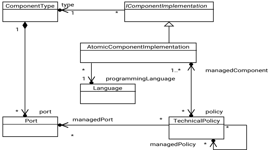
Figure 30: UCM atomic component implementations
