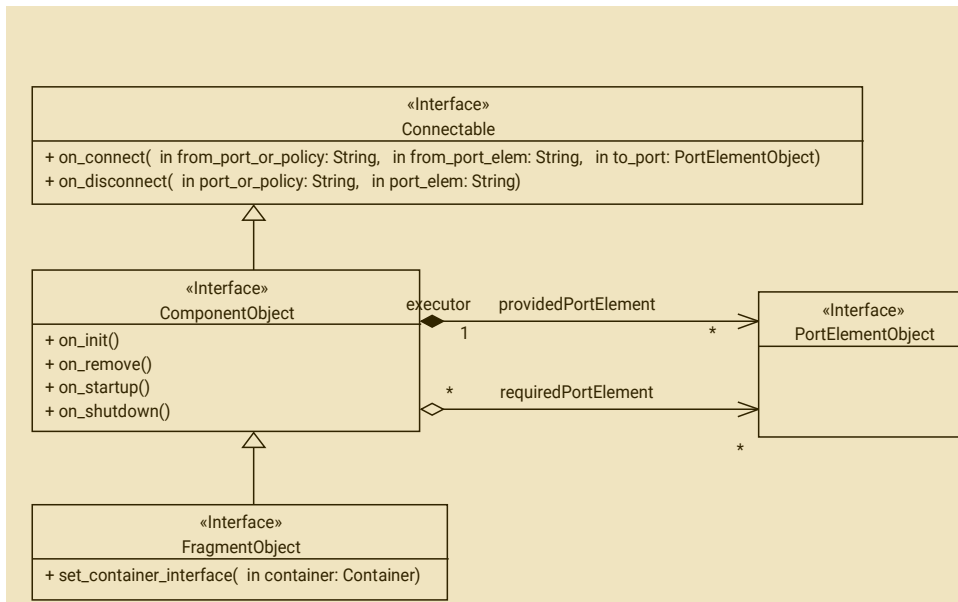
Figure 38: UCM Component Body Interfaces
