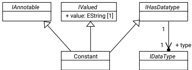
Figure 17: UCM constants
