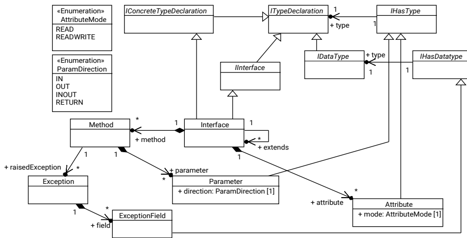
Figure 18: UCM interfaces
