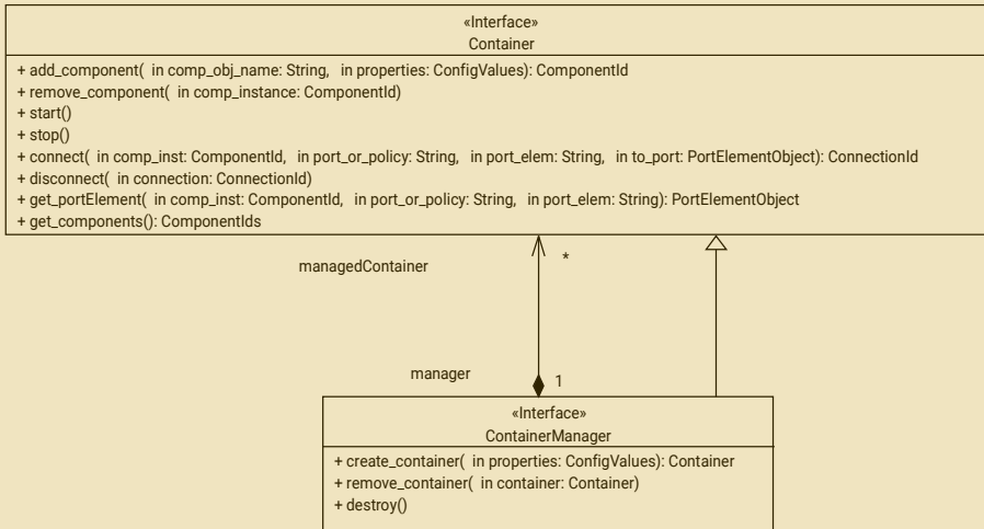
Figure 39: Container and container manager
