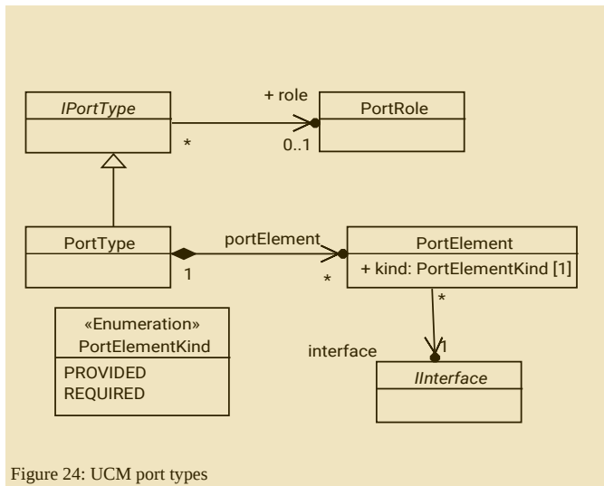
Figure 24: UCM port types
