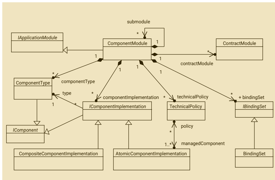
Figure 26: Main classes involved in the UCM component package
