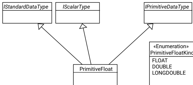
Figure 9: UCM floating point numbers
