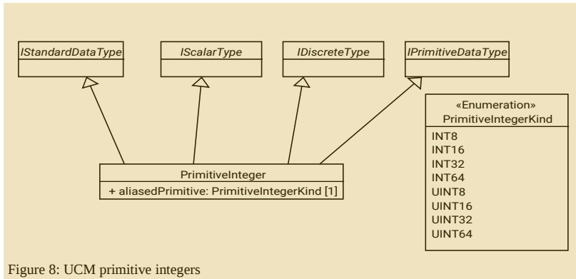
Figure 8: UCM primitive integers
