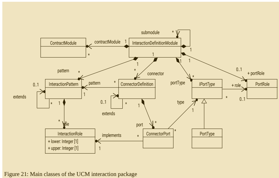
Figure 21: Main classes of the UCM interaction package
