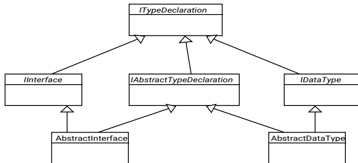
Figure 19: UCM abstract types
