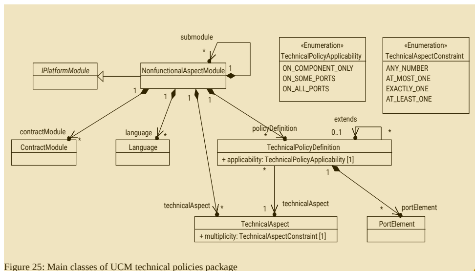
Figure 25: Main classes of UCM technical policies package
