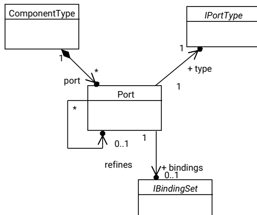
Figure 29: UCM component ports
