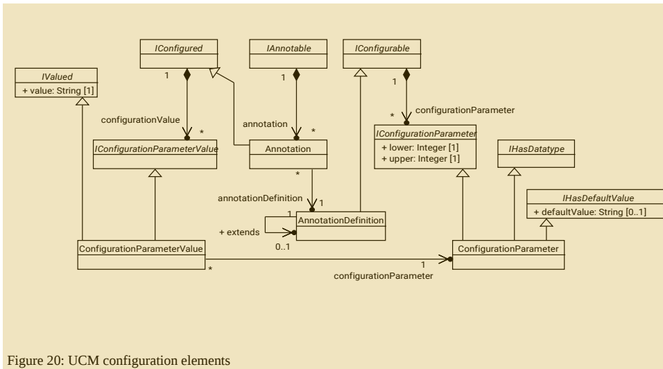
Figure 20: UCM configuration elements
