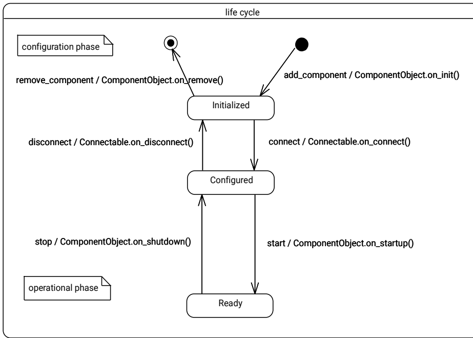
Figure 40: UCM Component Instance Life Cycle
