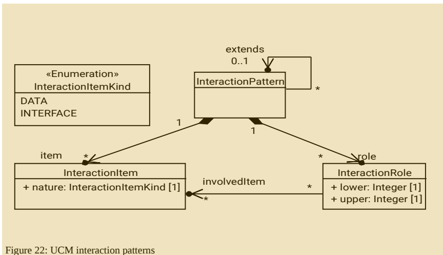
Figure 22: UCM interaction patterns
