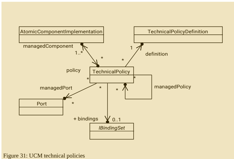
Figure 31: UCM technical policies
