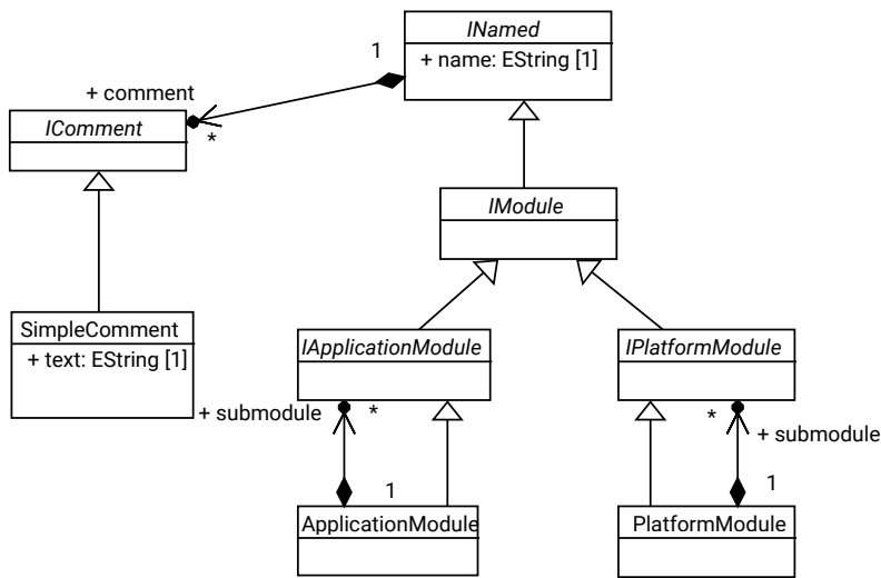
Figure 5: Base classes
