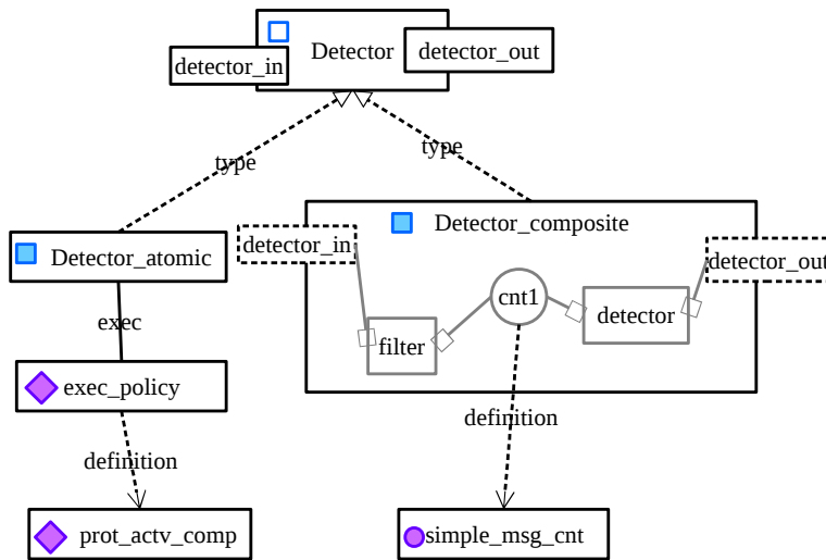
Figure 33: graphical example
