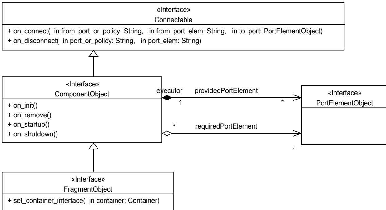
Figure 14.5: UCM Component Body Interfaces
