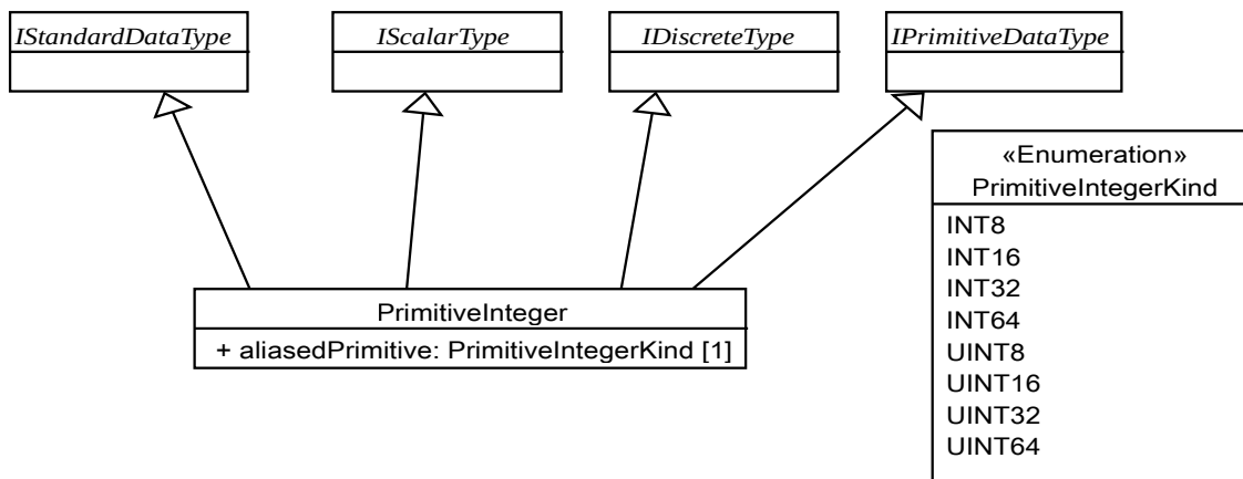
Figure 9.6 - UCM primitive integers
