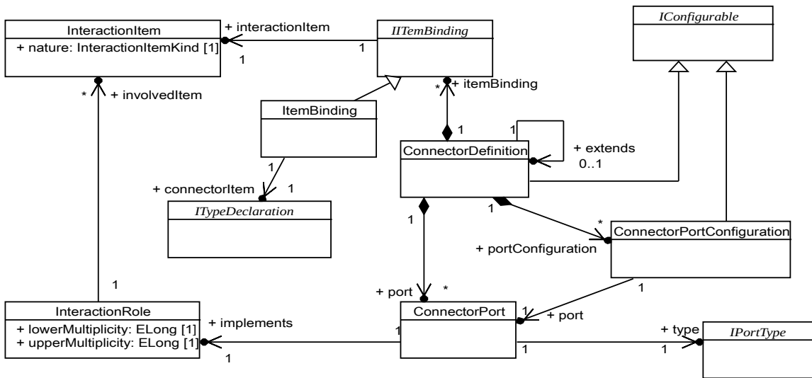
Figure 9.21 - UCM connectors
