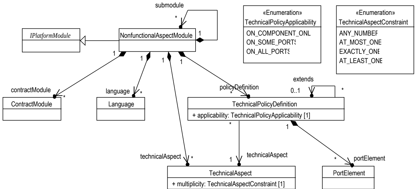
Figure 9.23 - Main classes of UCM technical policies package
