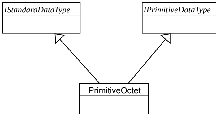
Figure 9.10 - UCM primitive octet
