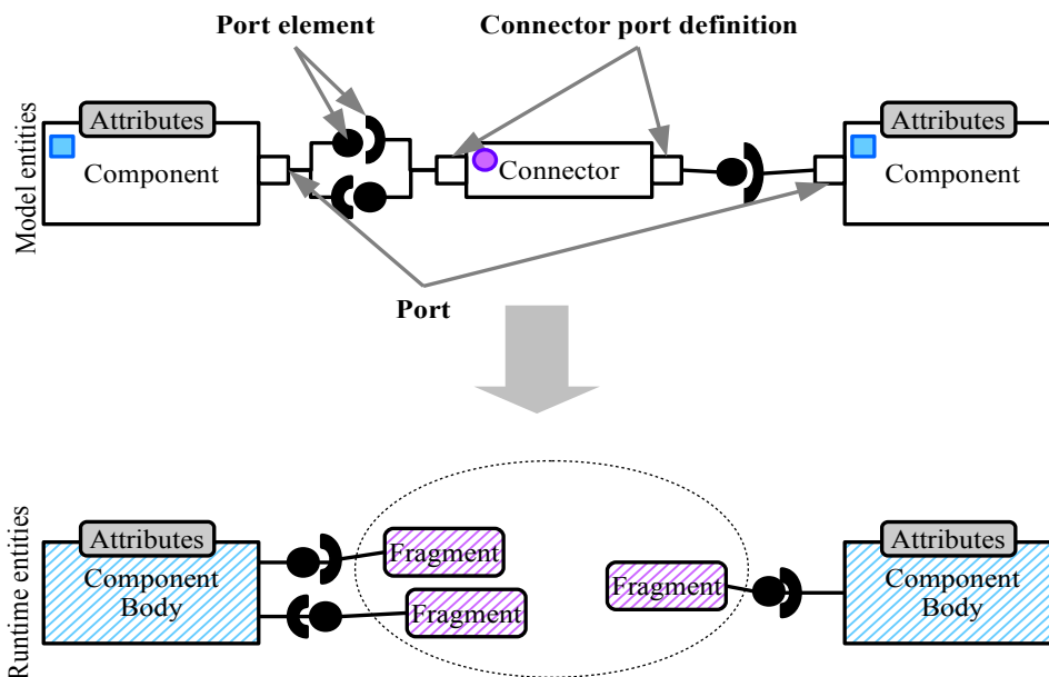
Figure 14.1: Connector fragmentation example
