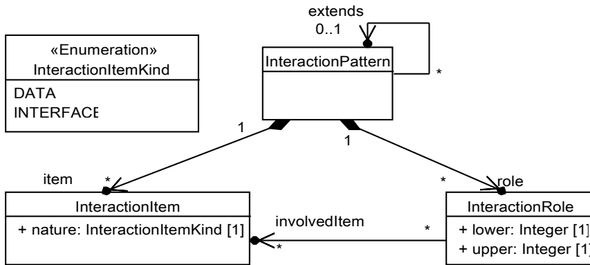
Figure 9.20 - UCM interaction patterns
