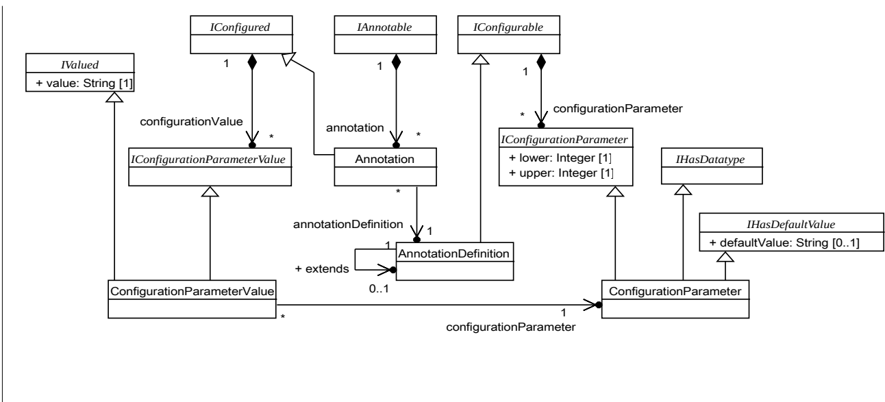
Figure 9.18 - UCM configuration elements
