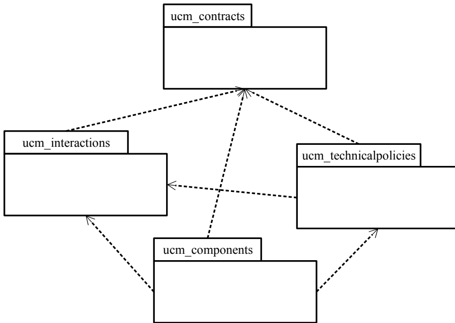
Figure 9.2 - Main packages in the UCM meta-model
