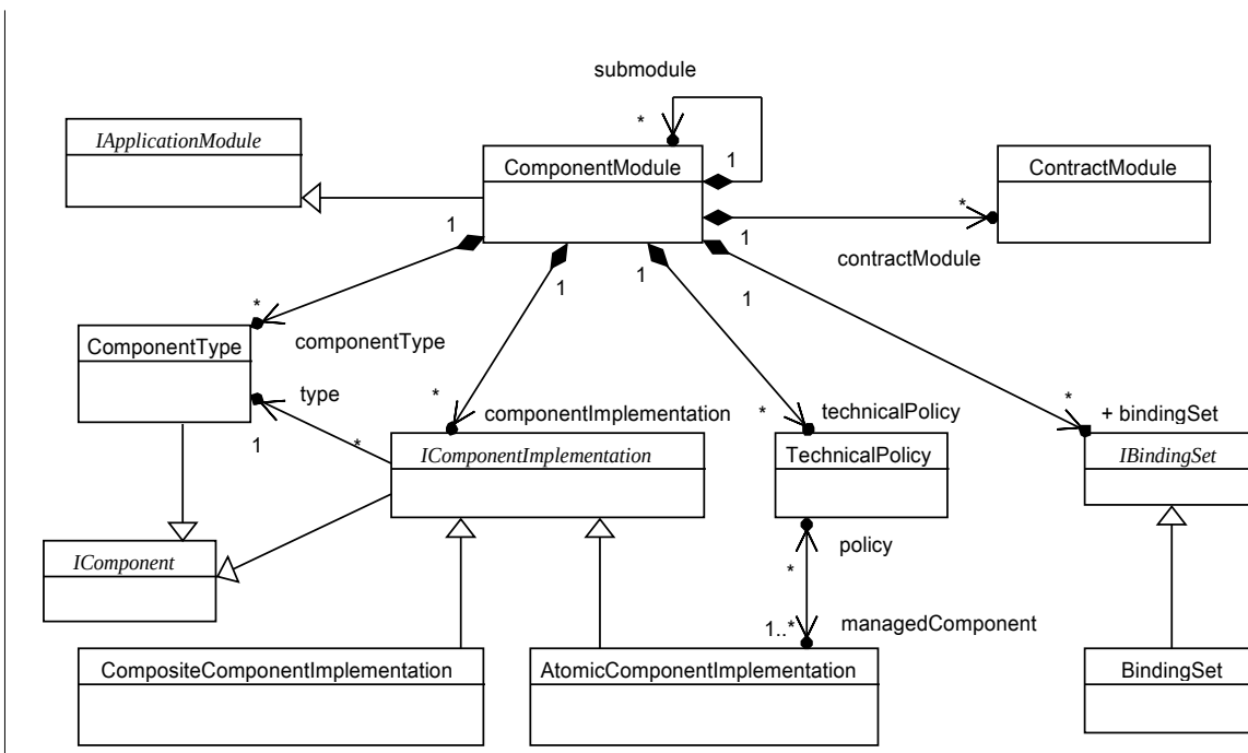
Figure 9.24: Main classes involved in the UCM component package
