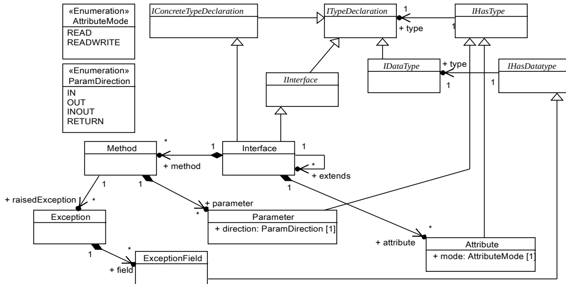
Figure 9.16 - UCM interfaces
