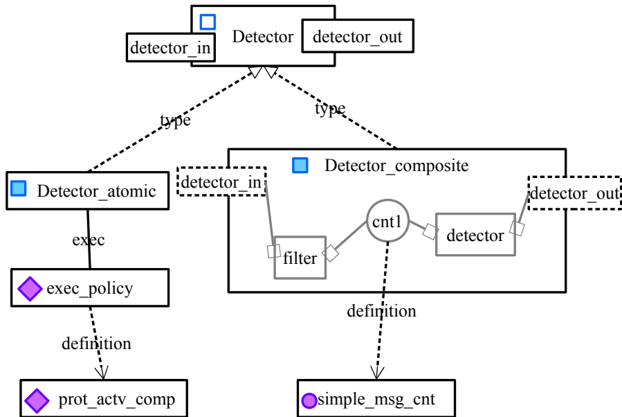
Figure 11.1: graphical example
