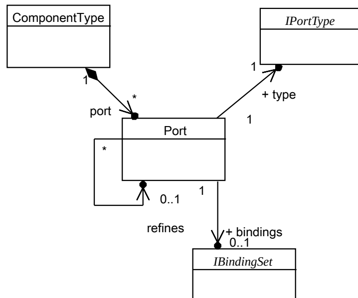
Figure 9.27: UCM component ports
