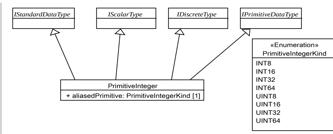
Figure 9.6 - UCM primitive integers
