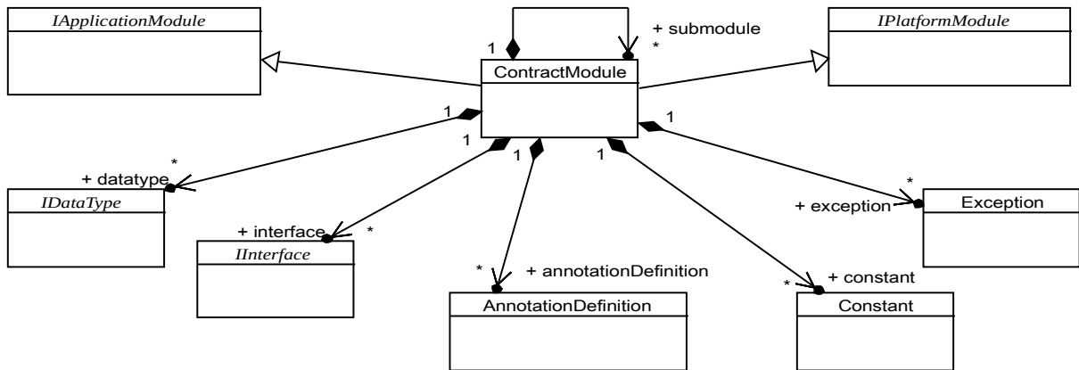
Figure 9.5 - UCM contract base declarations
