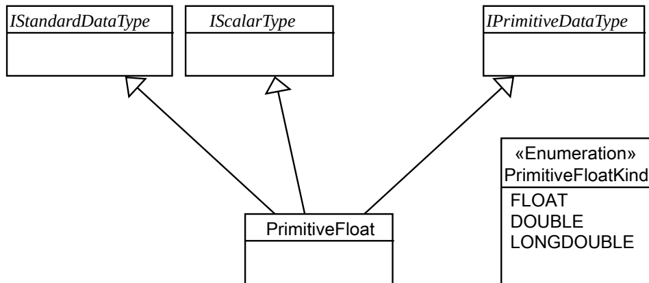
Figure 9.7 - UCM floating point numbers
