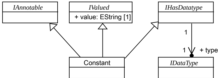
Figure 9.15 - UCM constants
