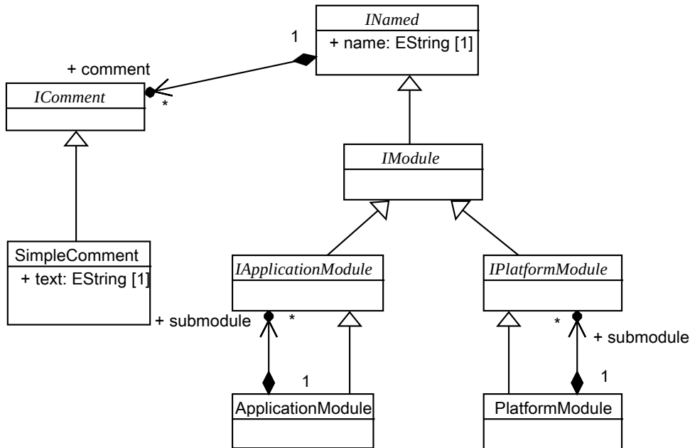
Figure 9.3 - Base classes
