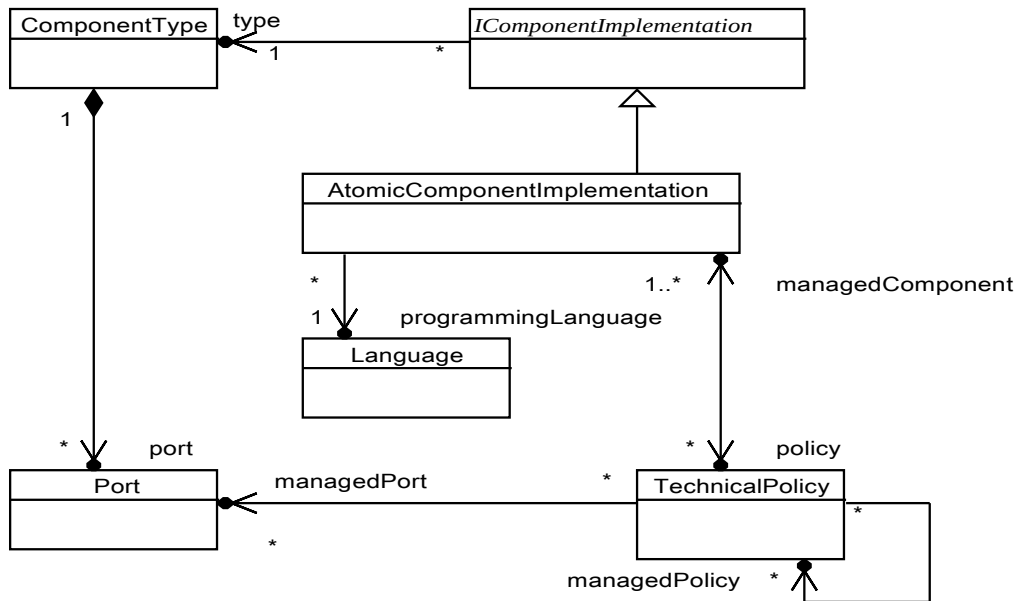
Figure 9.28: UCM atomic component implementations
