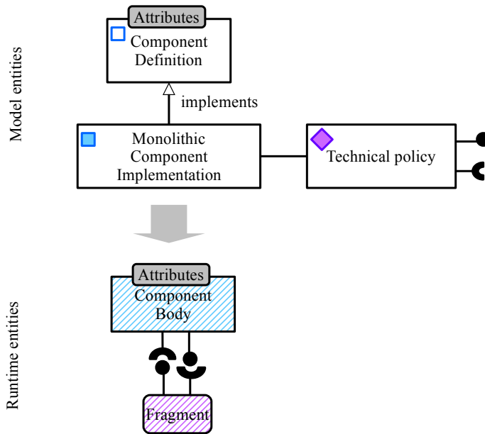
Figure 14.2: Technical policy fragmentation example
