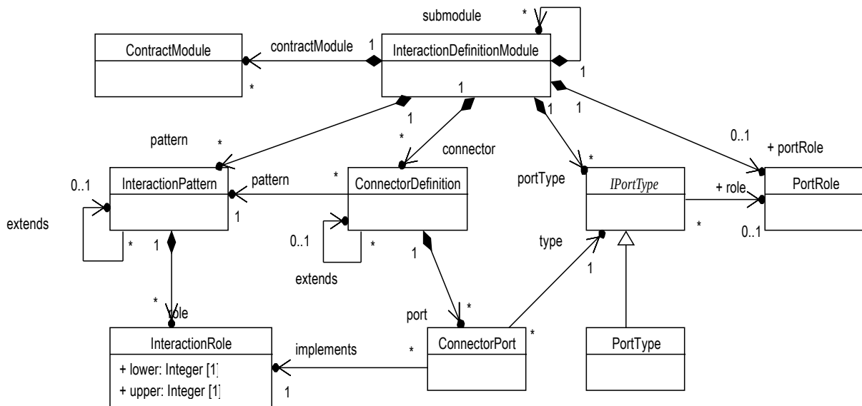
Figure 9.19 - Main classes of the UCM interaction package
