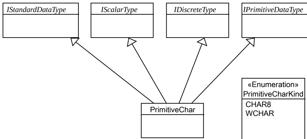
Figure 9.8 - UCM primitive characters
