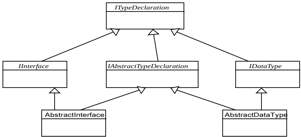
Figure 9.17 - UCM abstract types
