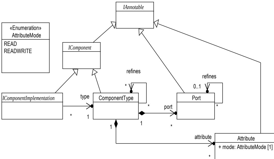
Figure 9.26: UCM component types
