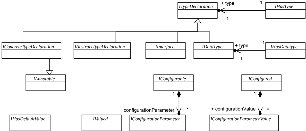
Figure 9.4 - Abstract base classes
