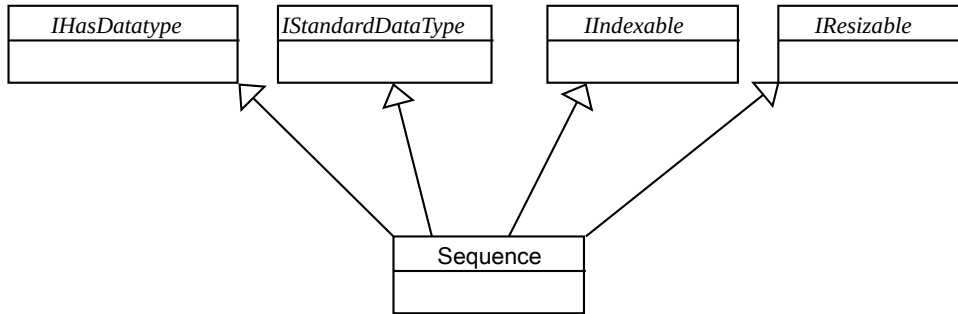
Figure 9.14 - UCM sequence
