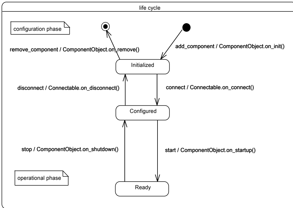
Figure 14.7: UCM Component Instance Life Cycle
