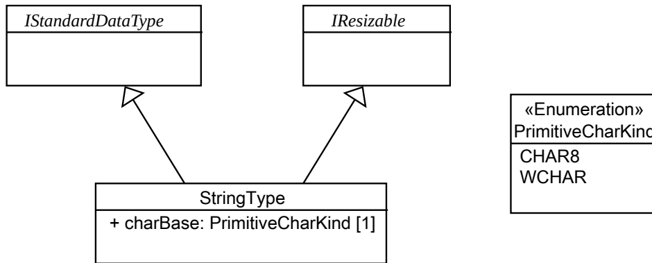
Figure 9.12 - UCM string type
