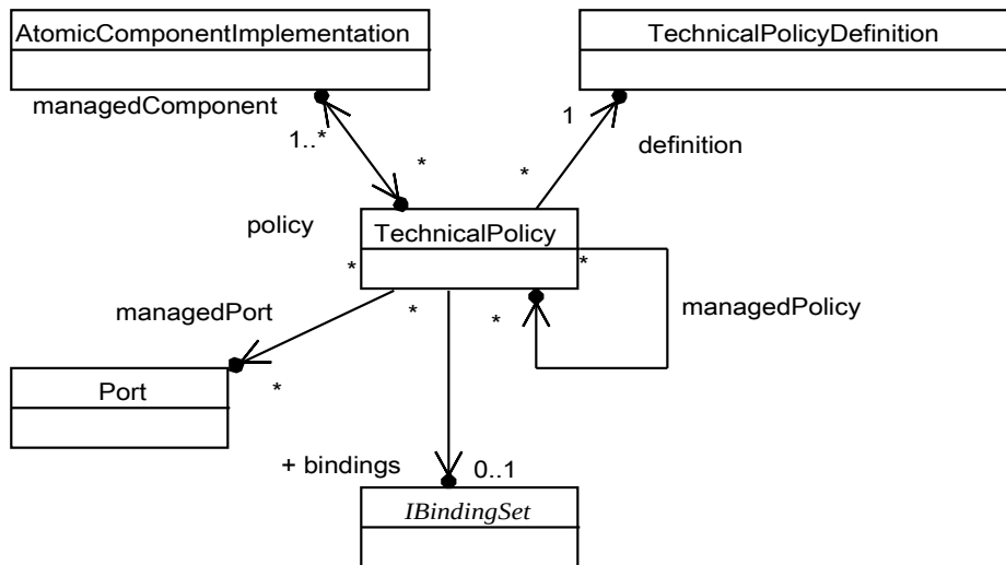
Figure 9.29: UCM technical policies
