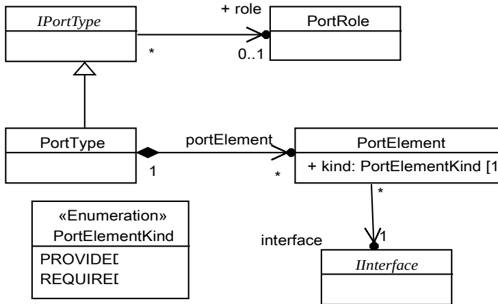
Figure 9.22 - UCM port types
