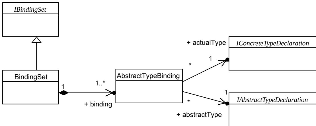
Figure 9.25: UCM binding sets
