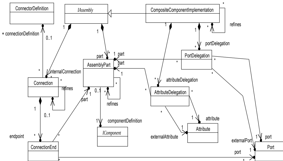
Figure 9.30: UCM composite component implementations
