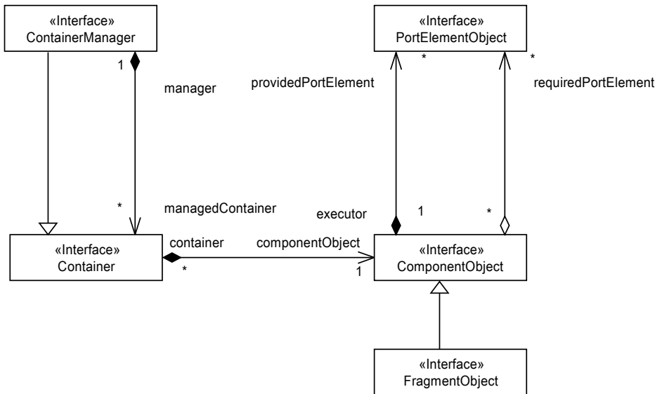
Figure 14.4: UCM Container Programming Model
