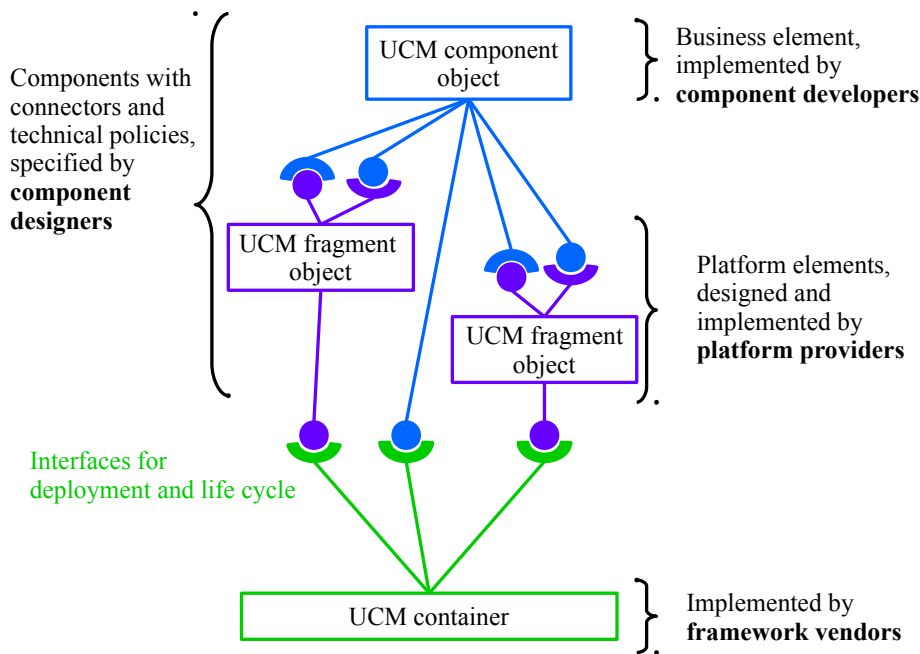
Figure 1.2 - Components implementation architecture and its integration within a UCM infrastructure
