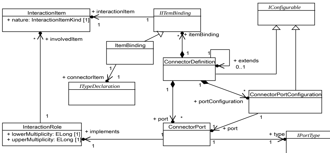
Figure 9.21 - UCM connectors
