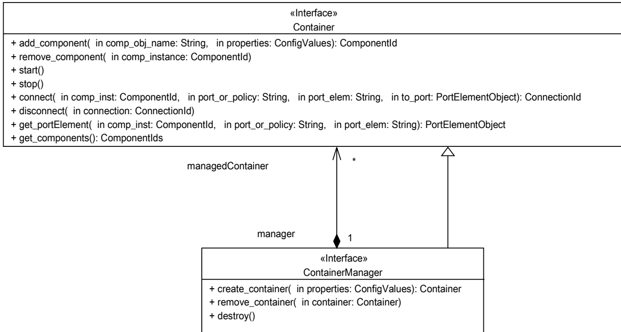
Figure 14.6: Container and container manager
