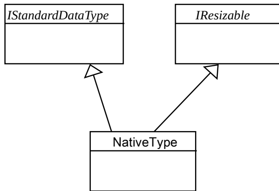
Figure 9.13 - UCM native type
