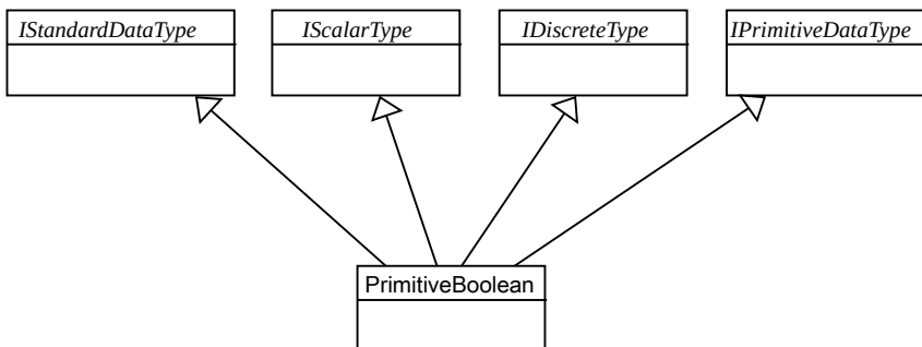
Figure 9.9 - UCM primitive boolean
