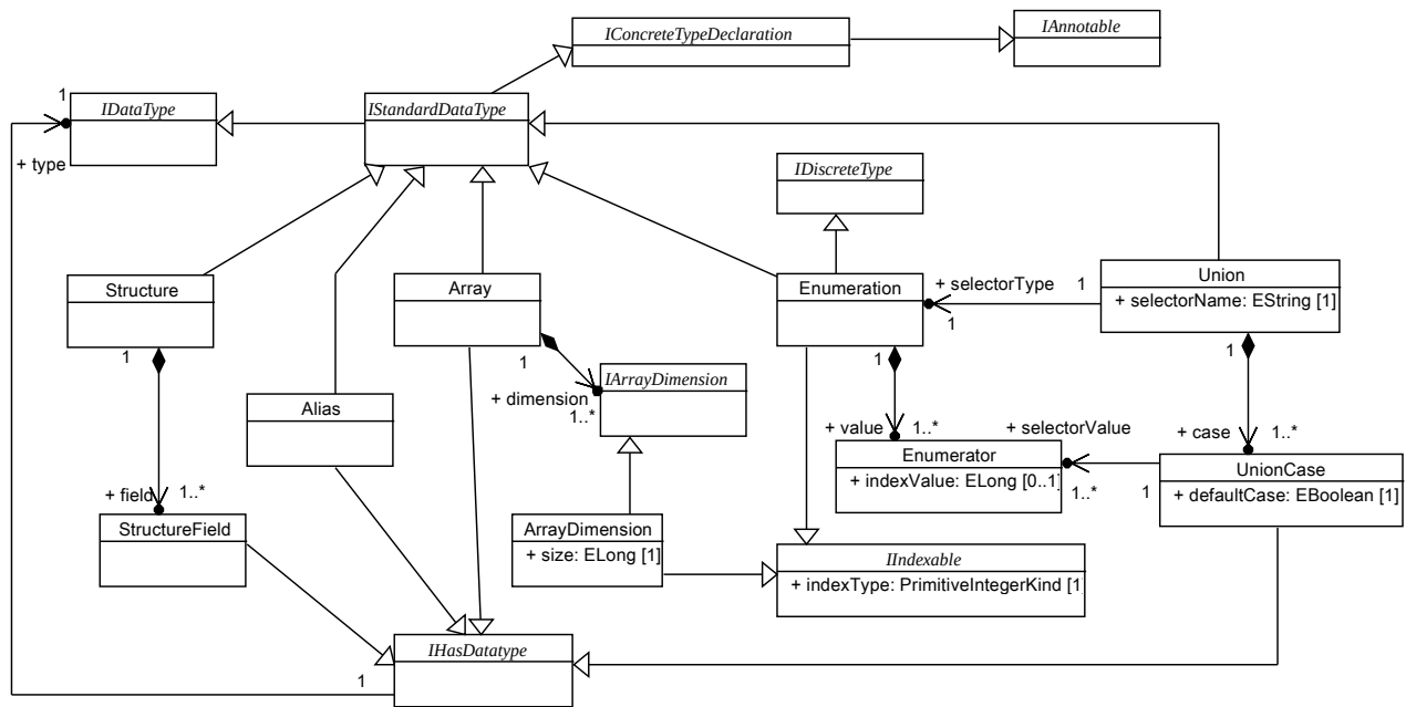
Figure 9.11 - UCM complex data types
