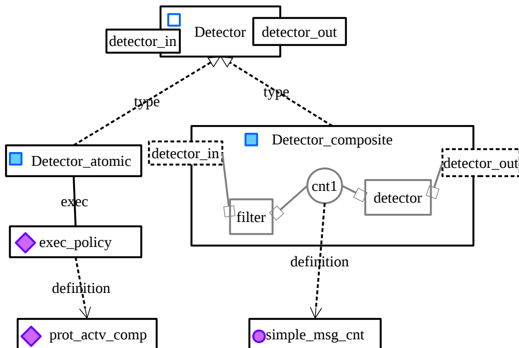
Figure 35: graphical example
