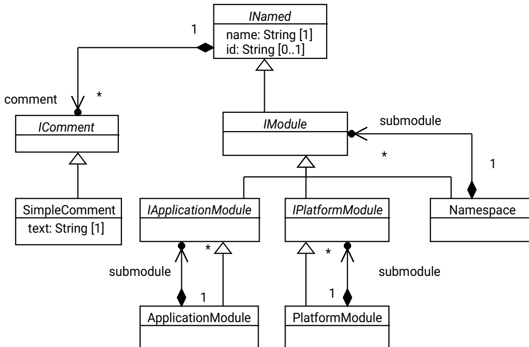
Figure 5: Base classes
