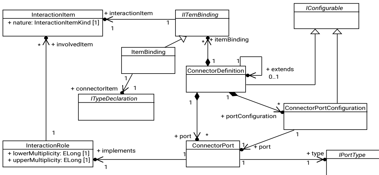
Figure 25: UCM connectors
