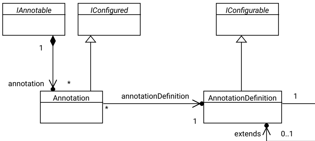
Figure 21: UCM annotations
