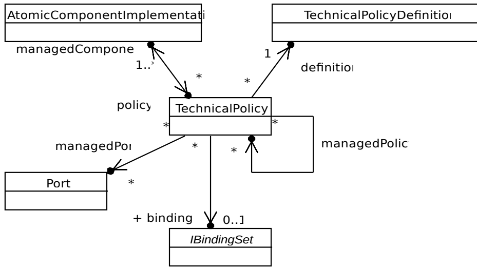
Figure 33: UCM technical policies
