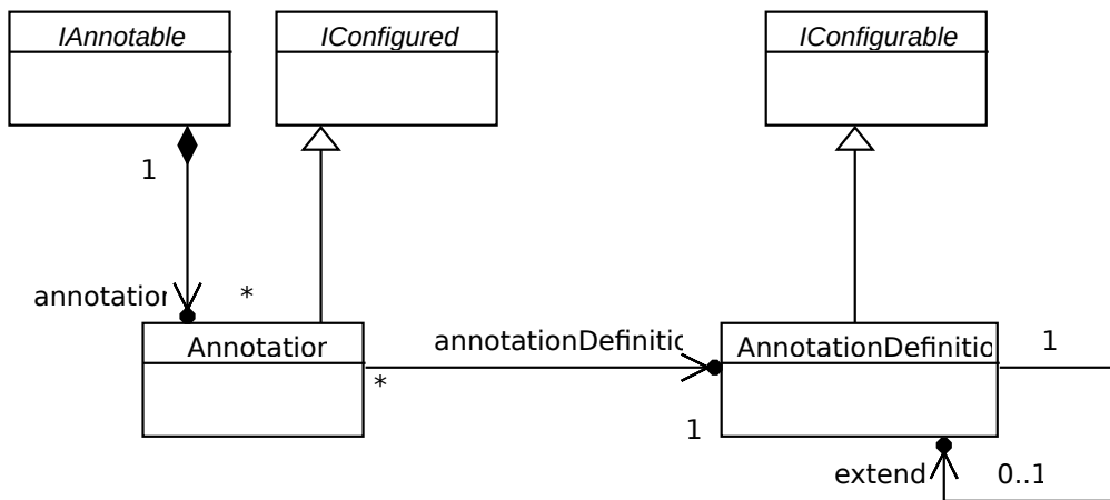
Figure 21: UCM annotations
