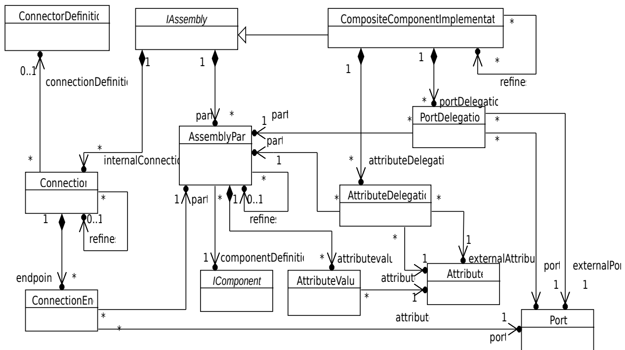
Figure 34: UCM composite component implementations
