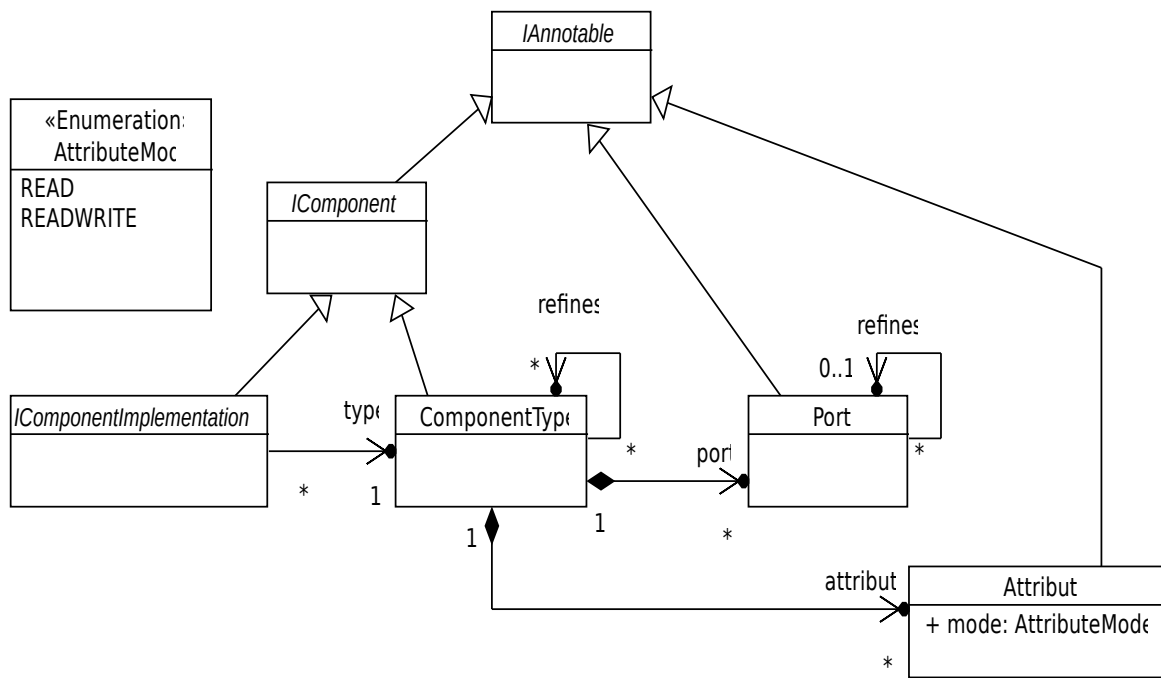
Figure 30: UCM component types
