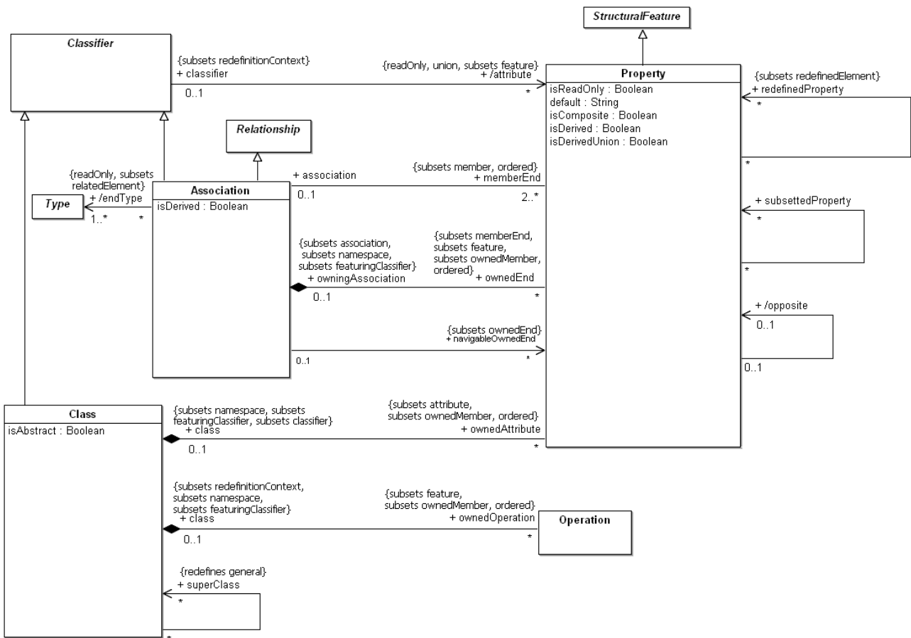
Figure 11.5 - The Classes diagram of the Constructs package
