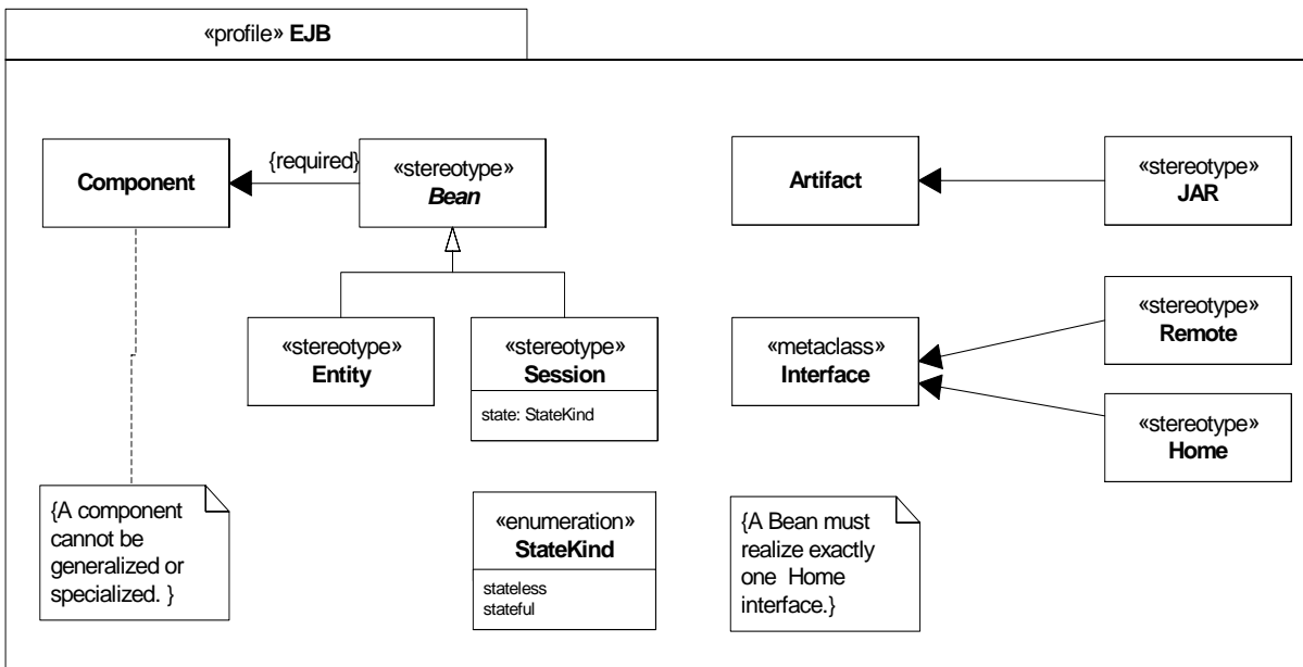
Figure 13.10 - Defining a simple EJB profile
