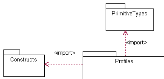
Figure 13.1 - Dependencies between packages described in this chapter
