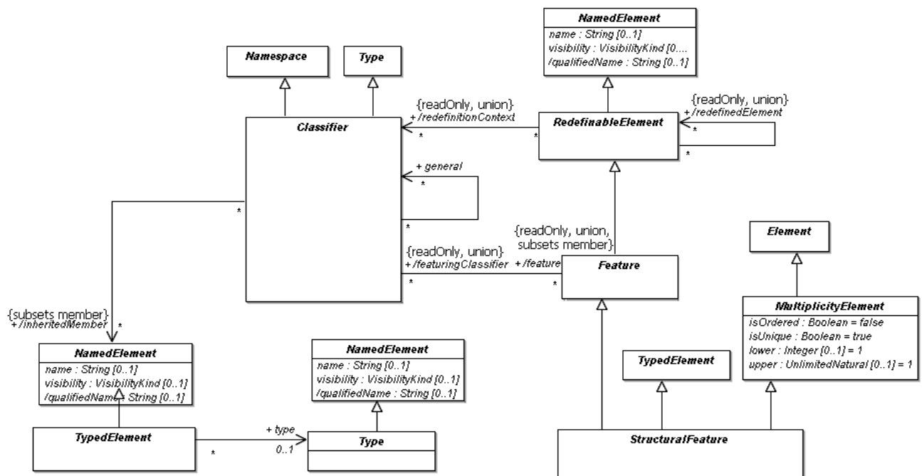
Figure 11.16 - The Classifiers diagram of the Constructs package
