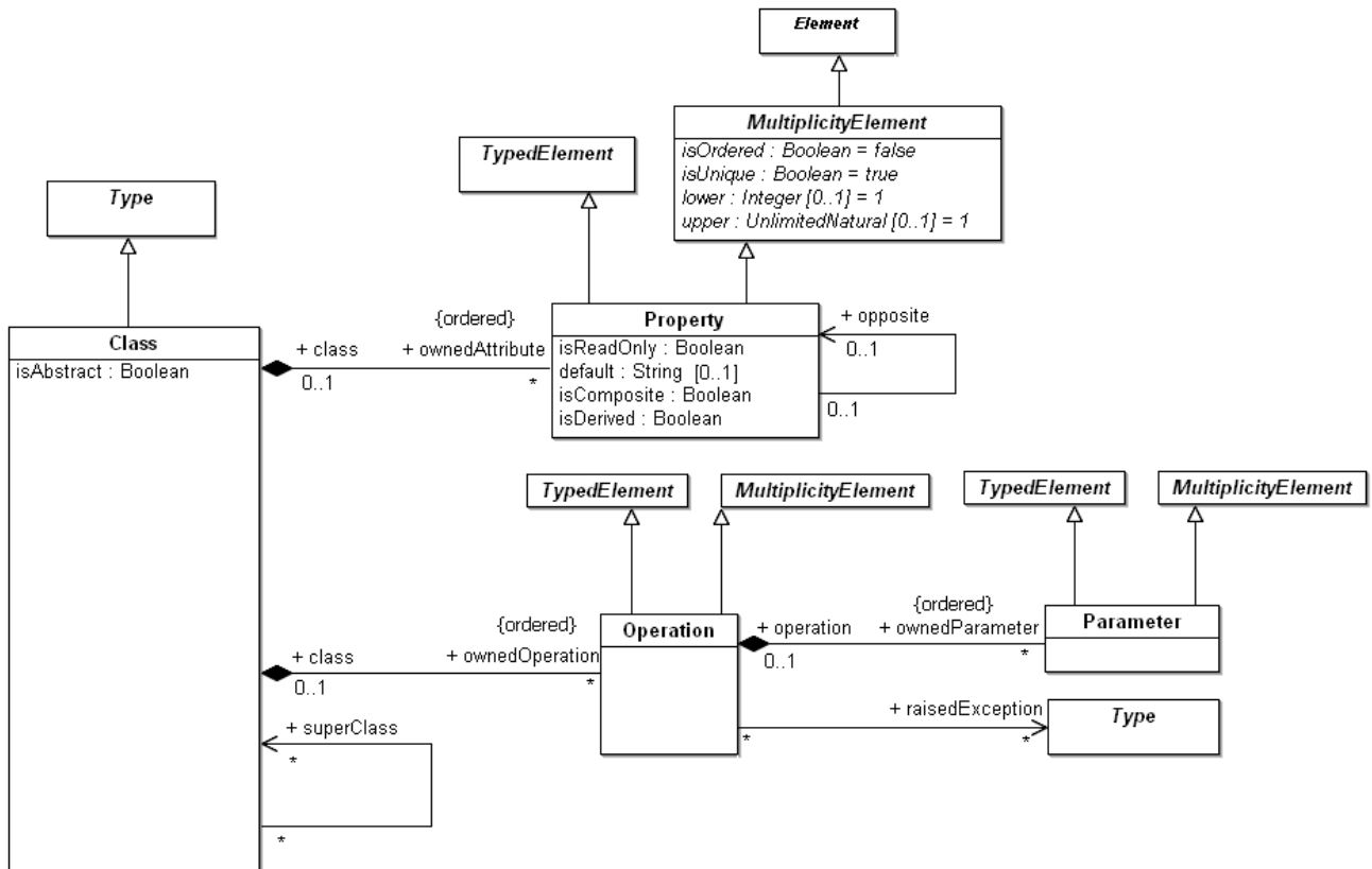
Figure 10.3 - The classes defined in the Classes diagram
