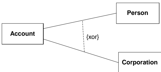
Figure 9.15 - {xor} constraint
