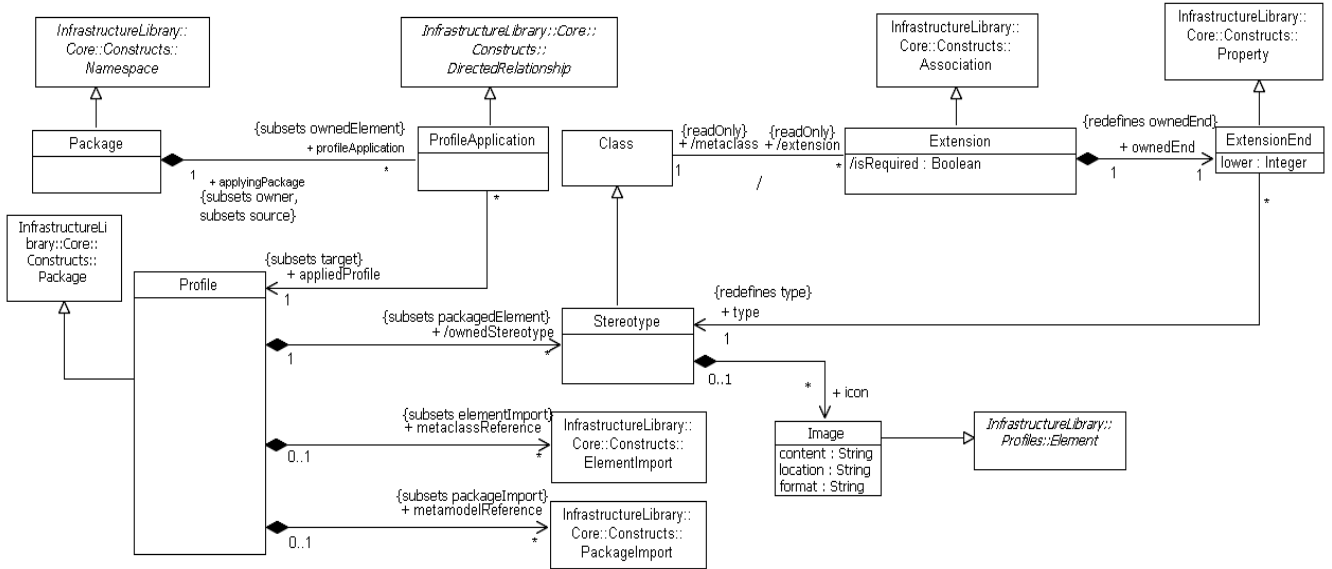
Figure 13.2 - The classes defined in the Profiles package
