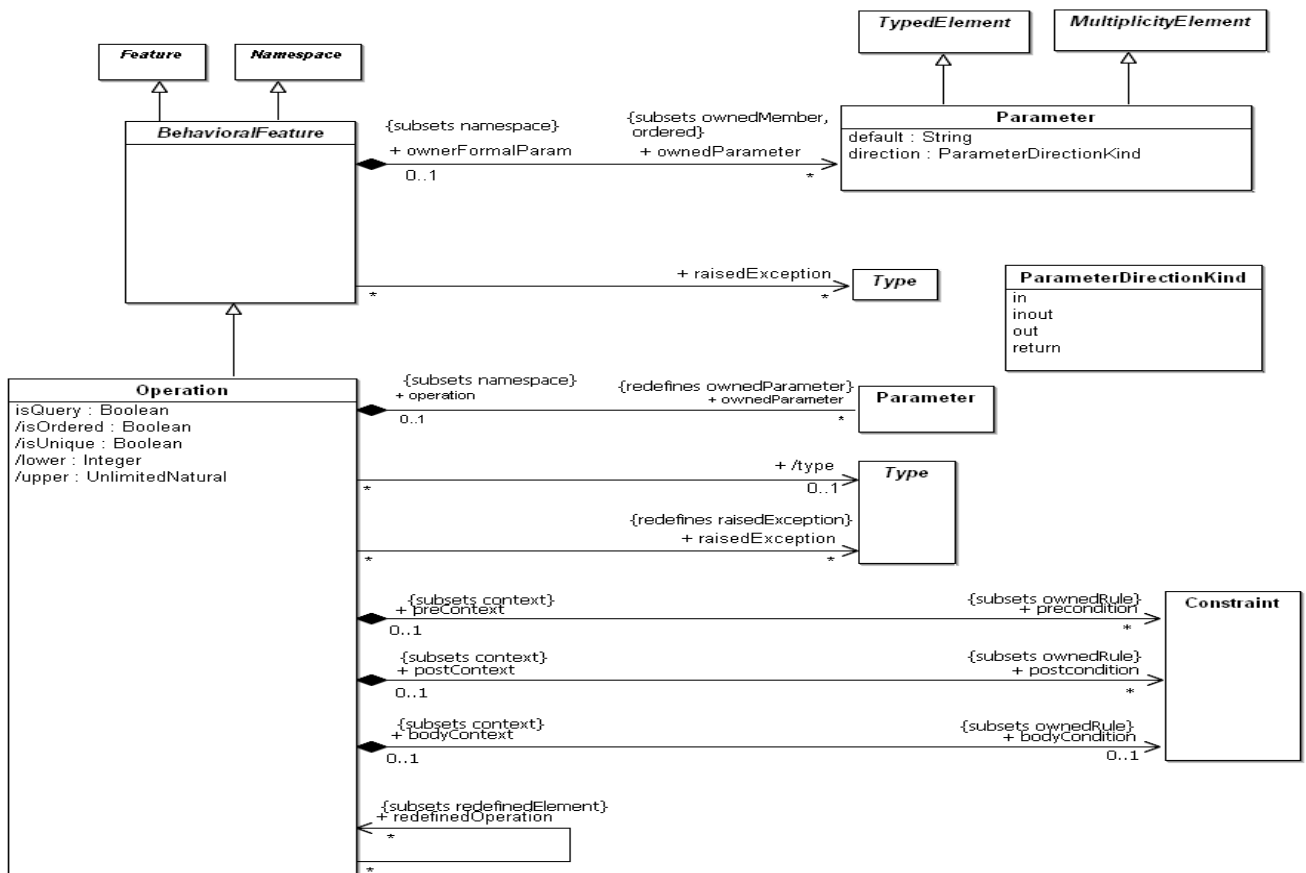
Figure 11.25 - The Operations diagram of the Constructs package
