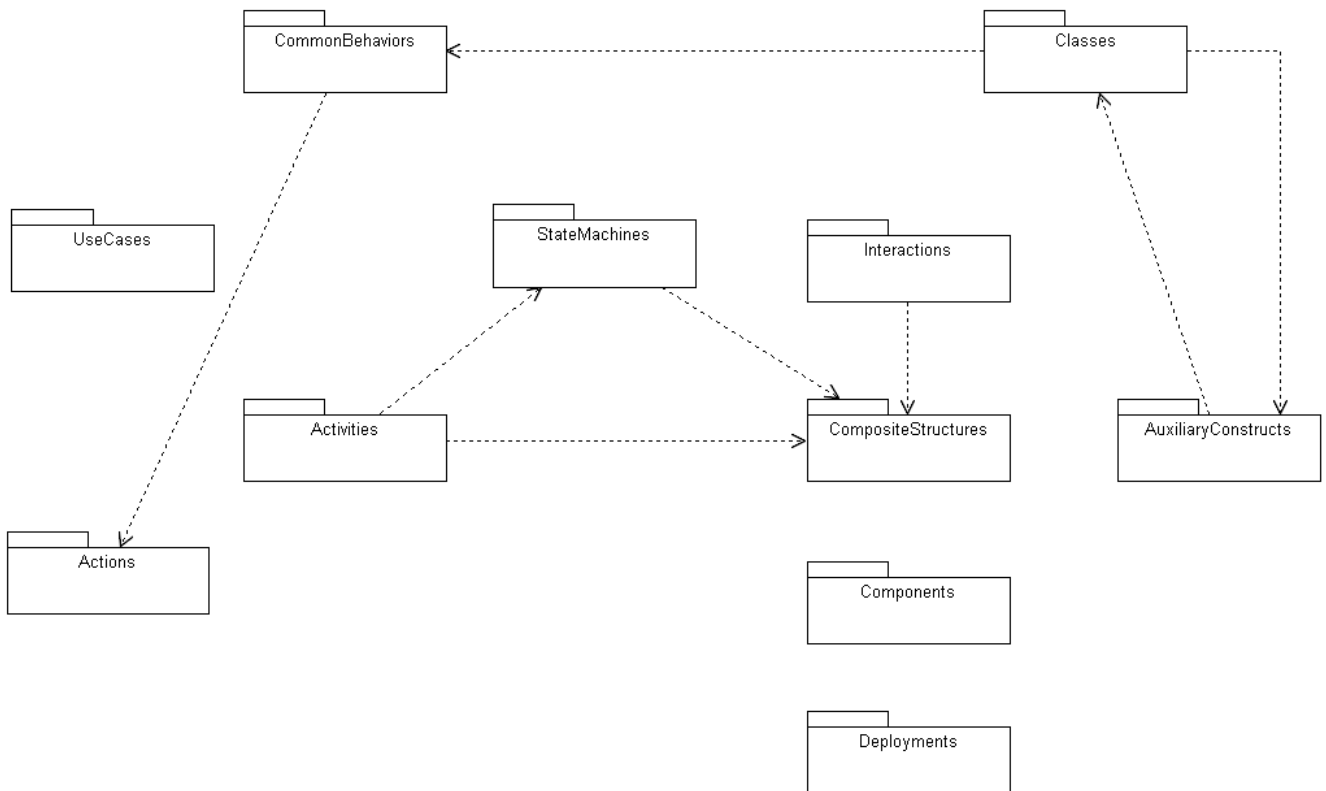
Figure 7.5 - The top-level package structure of the UML 2.1.1 Superstructure
