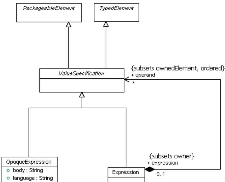
Figure 11.4 - The Expressions diagram of the Constructs package
