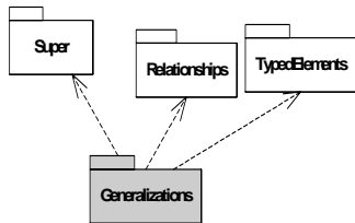
Figure 9.21 - The Generalizations package
