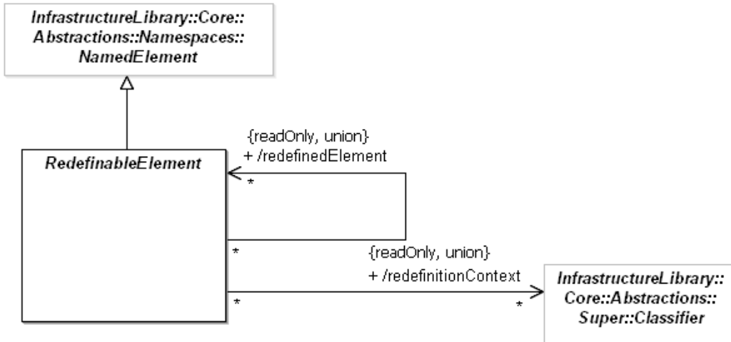
Figure 9.42 - The elements defined in the Redefinitions package
