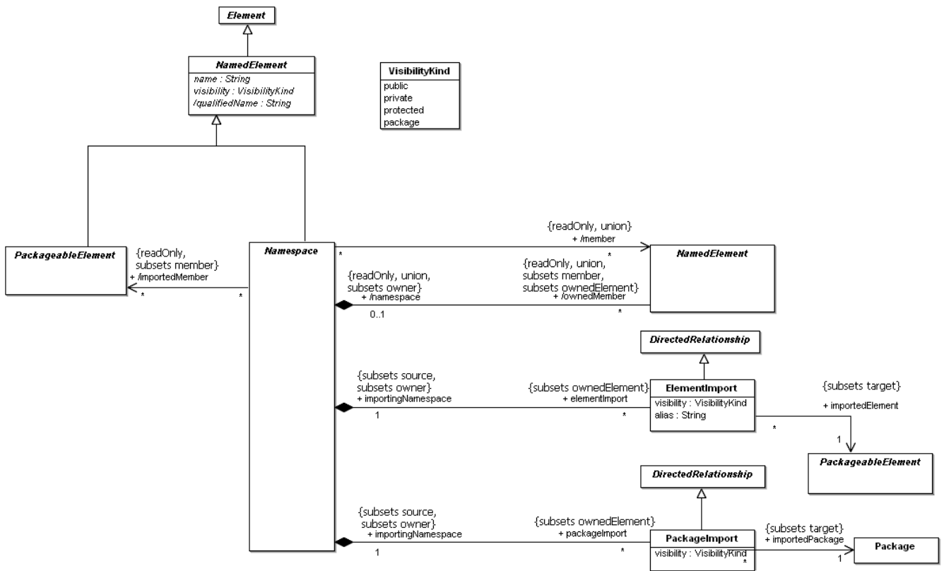
Figure 11.21 - The Namespaces diagram of the Constructs package
