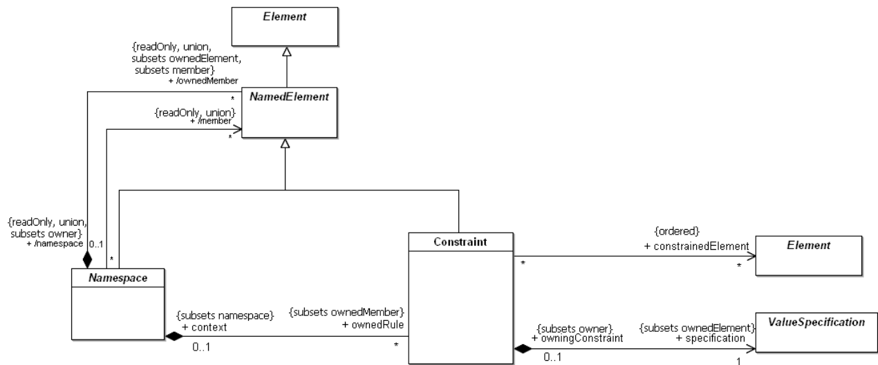
Figure 9.13 - The elements defined in the Constraints package
