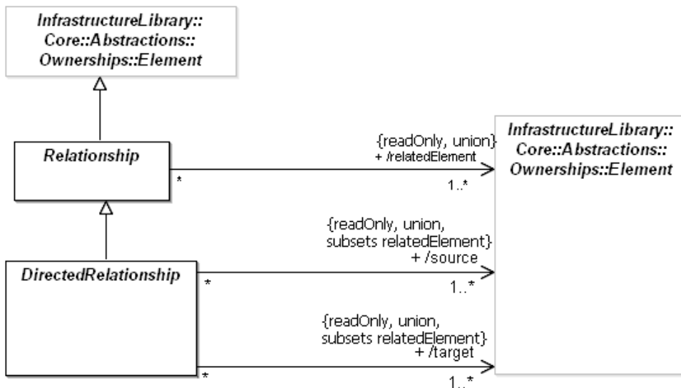
Figure 9.44 - The elements defined in the Relationships package
