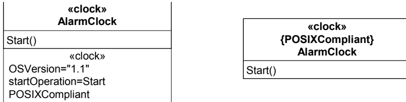
Figure 13.20 - Other notational forms for depicting stereotype values
