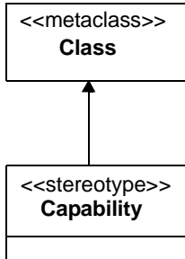
Figure 7.6 - Capabilities Generalization
