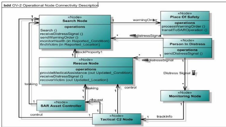
Figure D:15 - OV-2 Class Diagram
