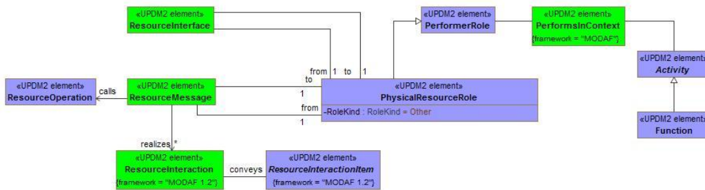
Figure A:34 - SV-10c/SvcV-10c - DMM
