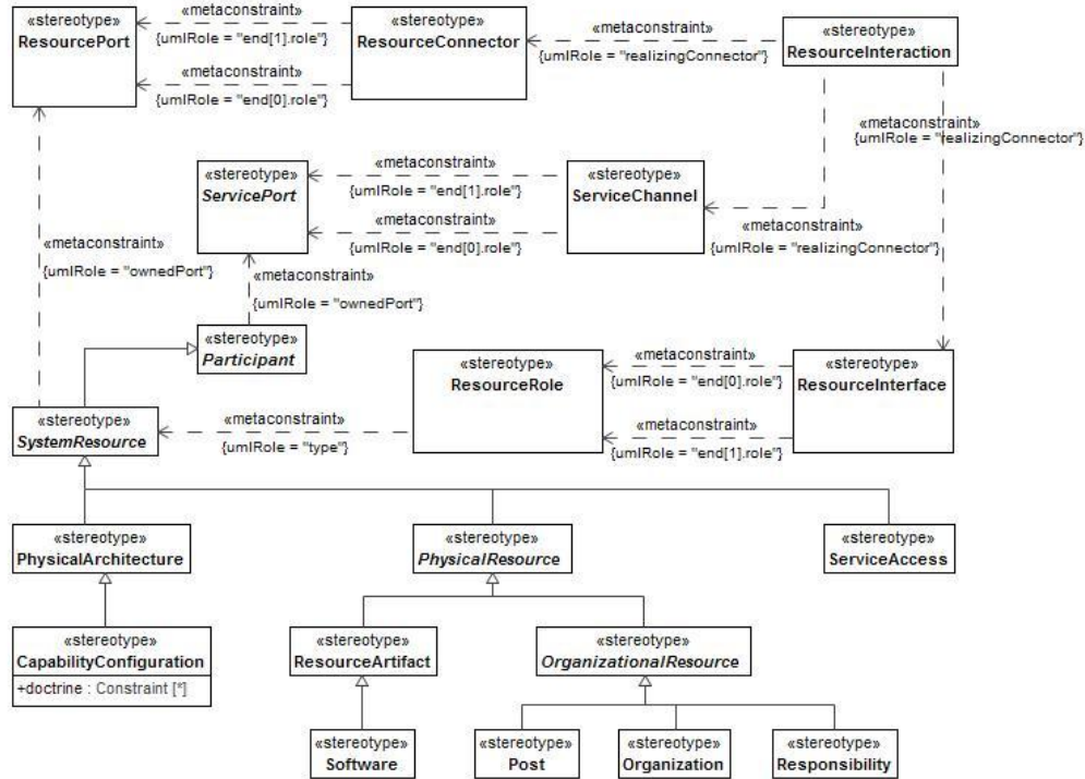
Figure B:40 - SV-3/SvcV-3a/SvcV-3b
