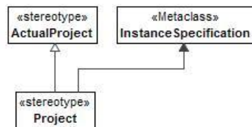
Figure 8:153 - Project
