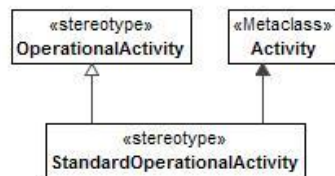
Figure 8:205 - StandardOperationalActivity
