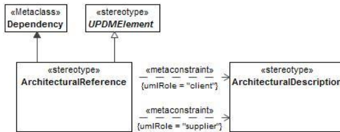
Figure 8:31 - ArchitecturalReference
