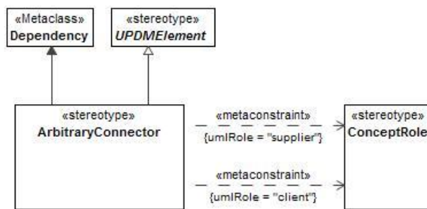
Figure 8:51 - ArbitraryConnector
