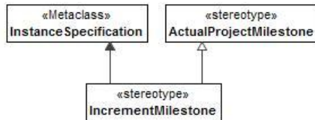
Figure 8:184 - IncrementMilestone
