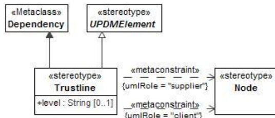
Figure 8:209 - Trustline
