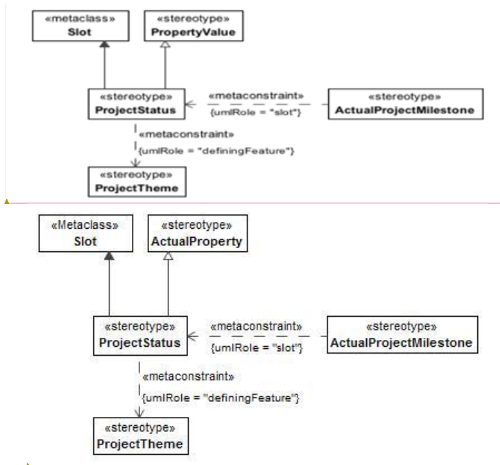
Figure 8:190 - ProjectStatus
