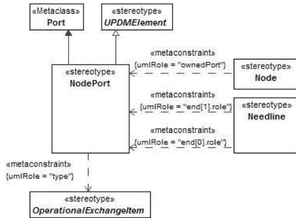
Figure 8:62 - NodePort
