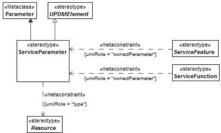
Figure 8:91 - ServiceParameter
