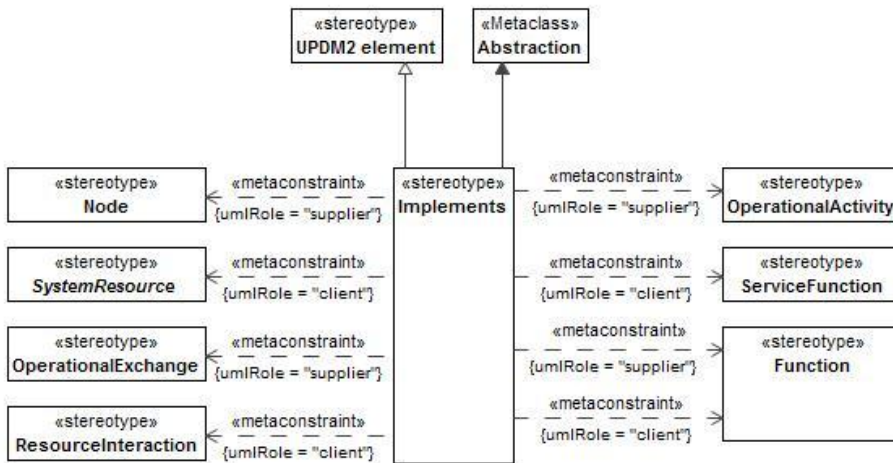
Figure 8:11 - Implements
