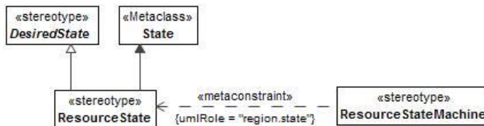
Figure 8:121 - ResourceState
