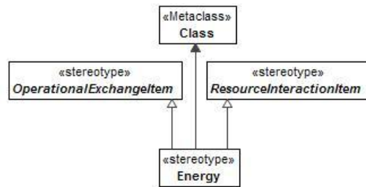
Figure 8:207 - Energy
