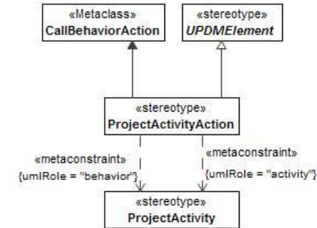
Figure 8:155 - ProjectActivityAction
