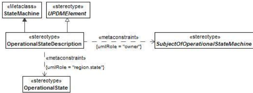
Figure 8:45 - OperationalStateDescription
