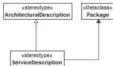
Figure 8:173 - ServiceDescription
