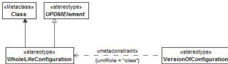
Figure 8:143 - WholeLifeConfiguration
