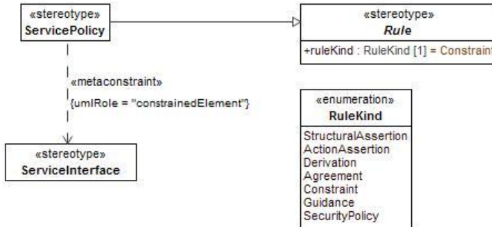
Figure B:22 - SOV-4a
