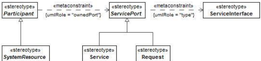
Figure B:38 - SV-12
