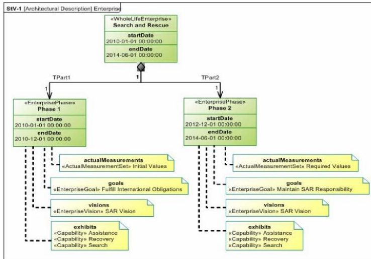
Figure D:7 - StV-1 Enterprise View
