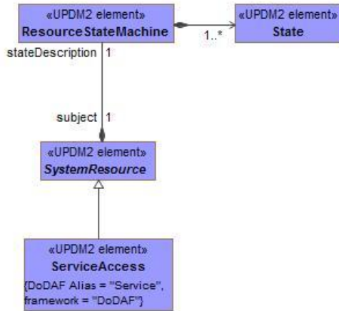
Figure A:33 - SV-10b/SvcV-10b DMM
