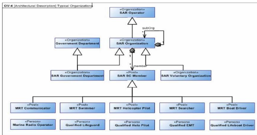
Figure D:18 - OV-4 Typical
