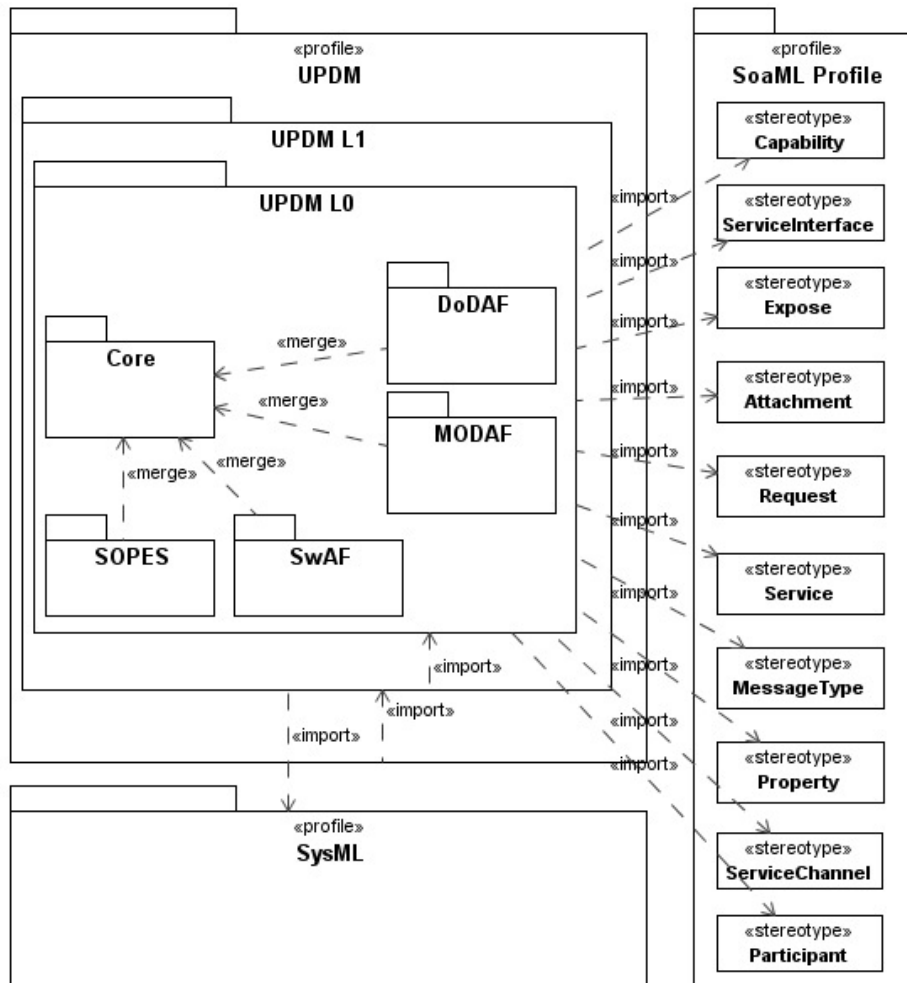
Figure 2:2 - L0 and L1
