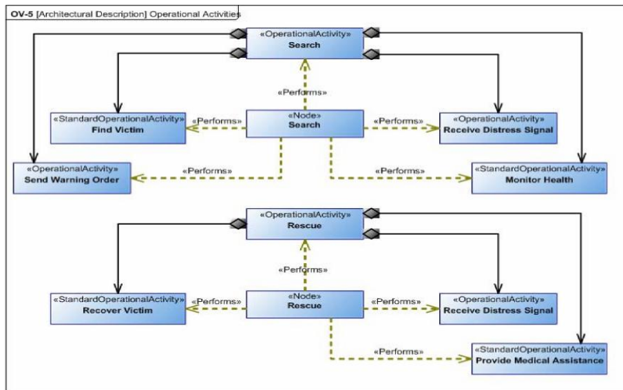
Figure D:20 - OV-5
