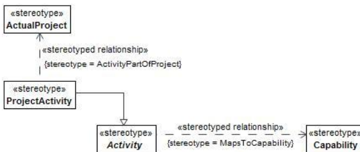
Figure B:3 - PV-3 Derived from Project Activity
