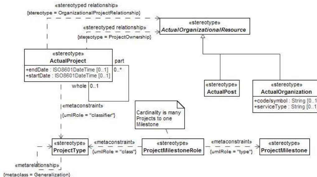
Figure B:1 - AcV-1/PV-1
