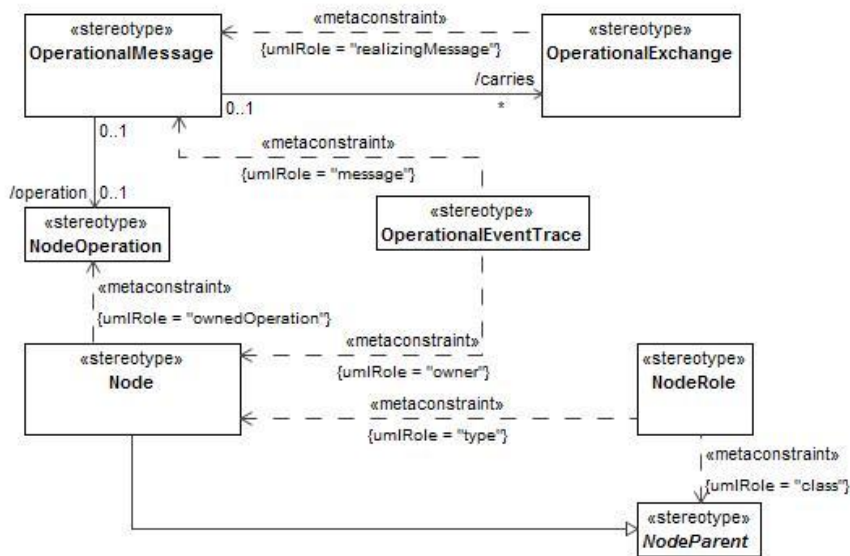
Figure B:17 - OV-6c
