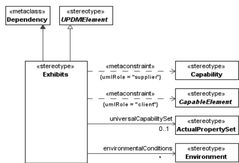
Figure 7:6 – "Exhibits" extends the UML Dependency metaclass
