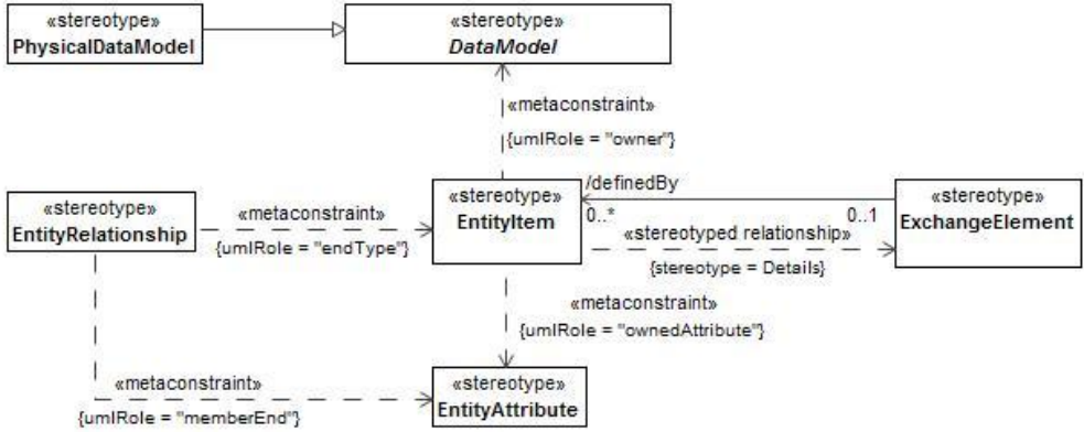
Figure B:37 - SV-11/DIV-3
