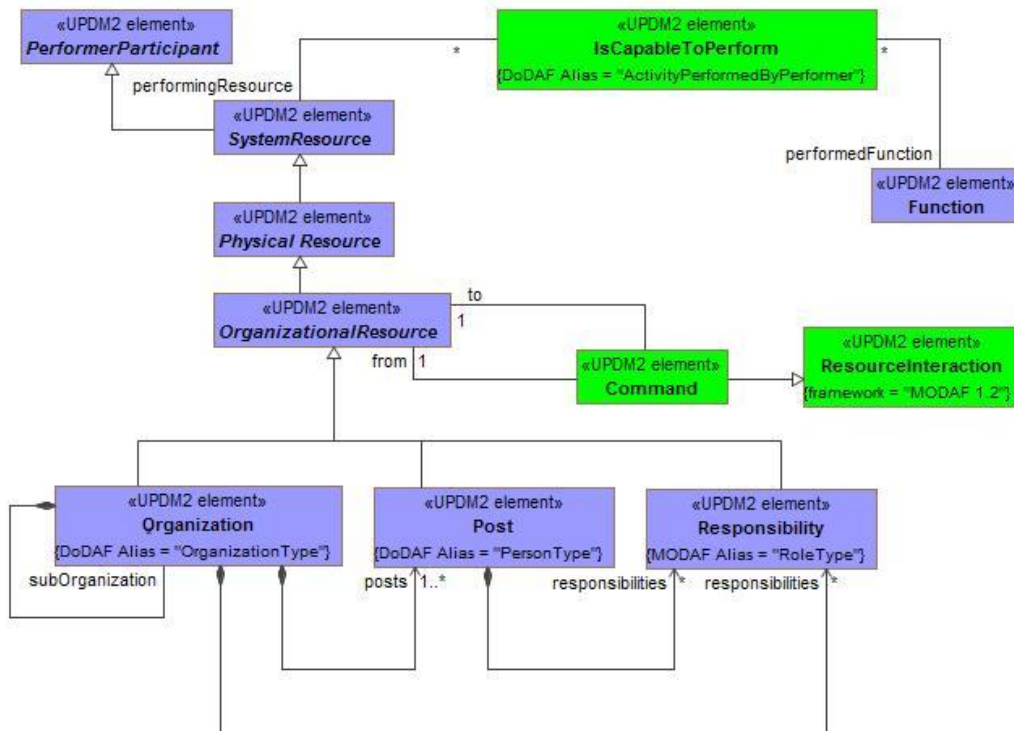
Figure A:11 - OV-4 Typical - DMM
