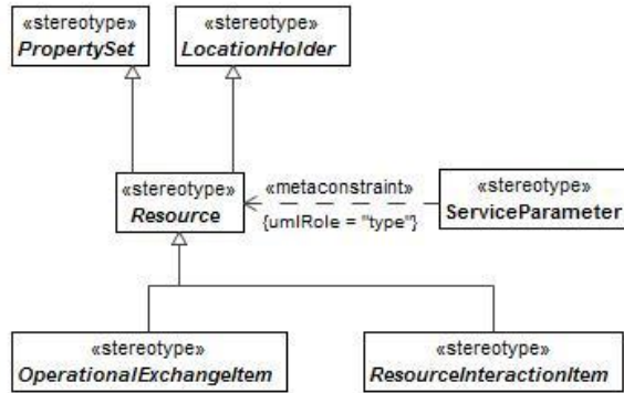
Figure 8:28 - Resource
