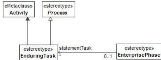
Figure 8:213 - EnduringTask
