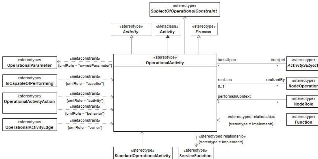
Figure 8:38 - OperationalActivity
