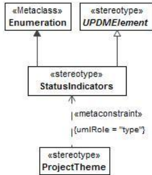
Figure 8:192 - StatusIndicators
