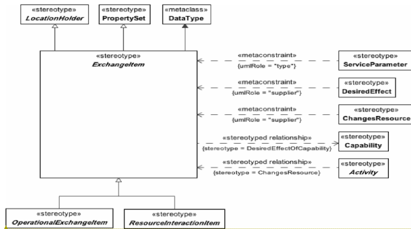
Figure :- ExchangeItem
