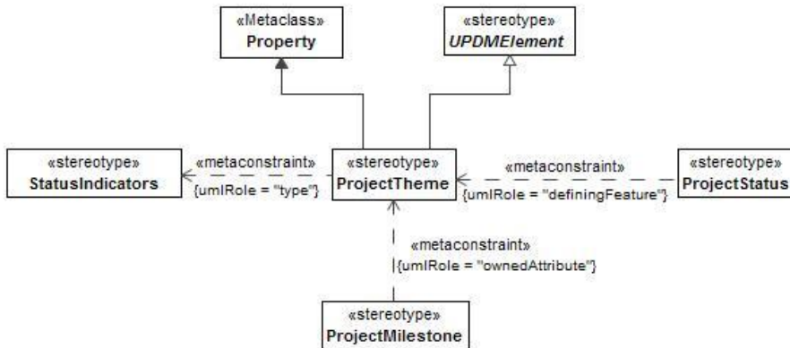
Figure 8:191 - ProjectTheme
