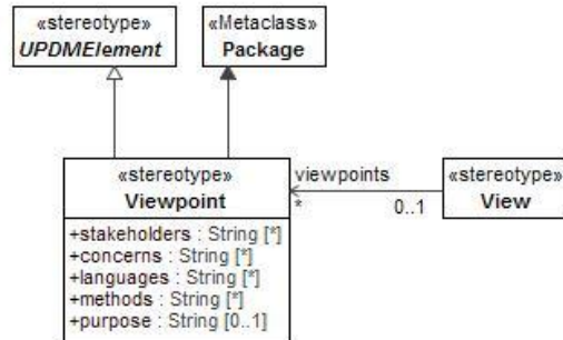
Figure 8:35 - Viewpoint
