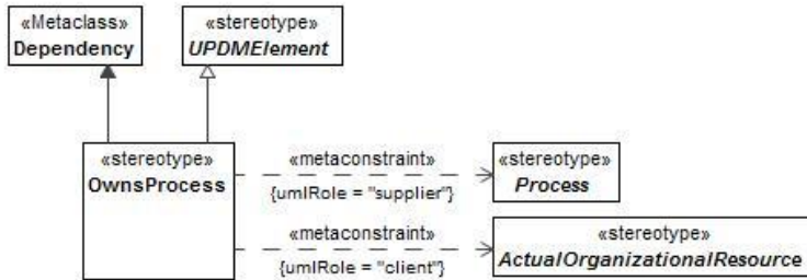
Figure 8:203 - OwnsProcess
