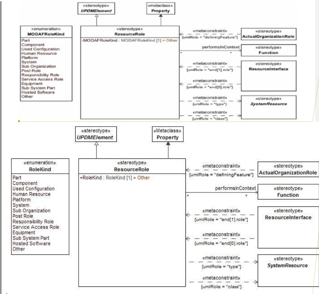
Figure 8:137 - ResourceRole
