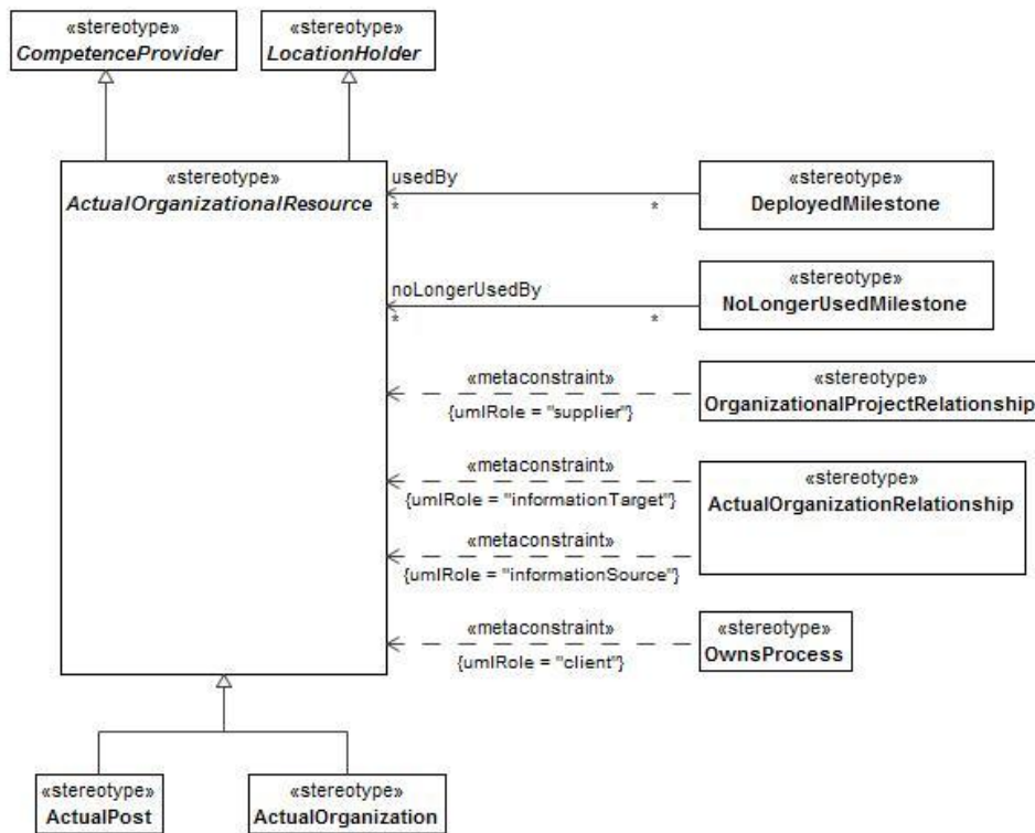
Figure 8:68 - ActualOrganizationalResource
