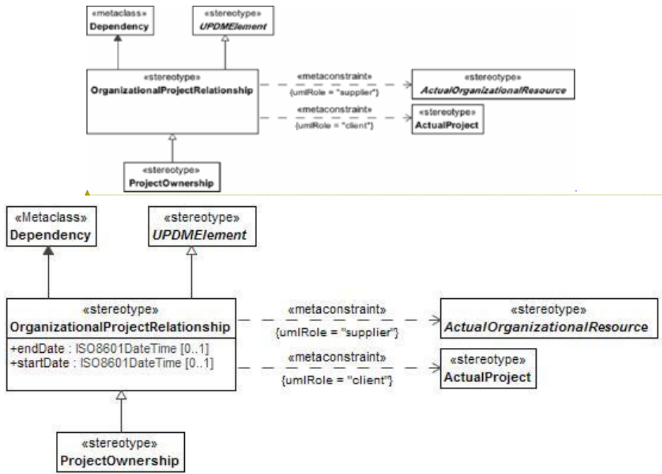
Figure 8:4 - OrganizationalProjectRelationship
