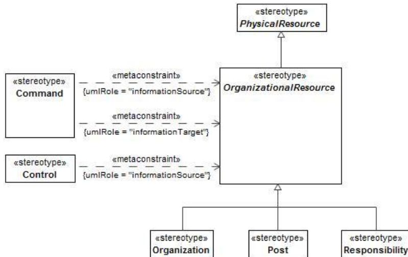
Figure 8:77 - OrganizationalResource
