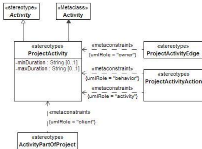
Figure 8:154 - ProjectActivity
