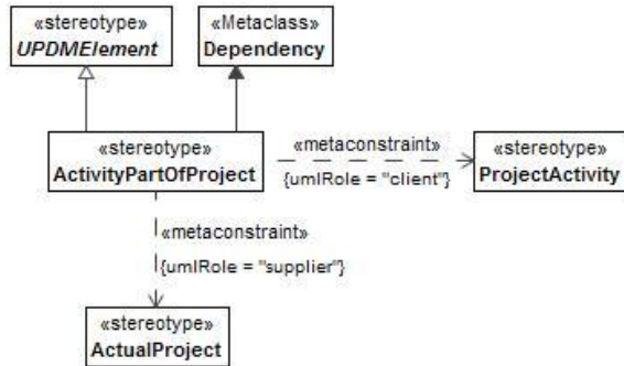
Figure 8:152 - ActivityPartOfProject
