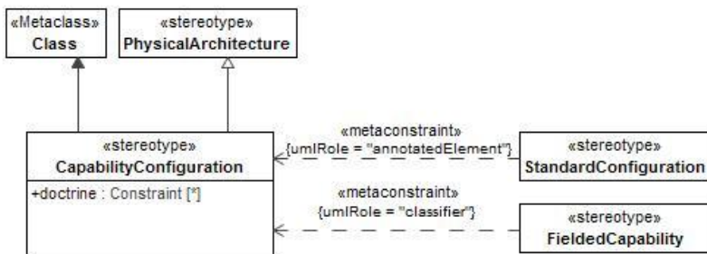
Figure 8:127 - CapabilityConfiguration
