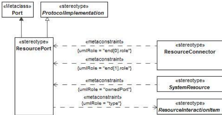
Figure 8:136 - ResourcePort
