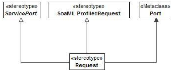
Figure 8:94 - Request
