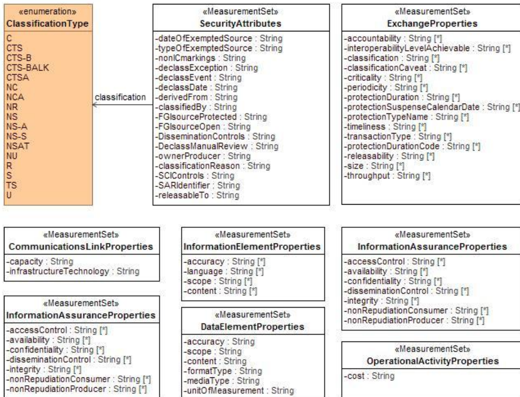
Figure 8:1 - DoDAF Class Library
