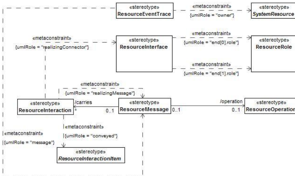
Figure B:36 - SV-10c/SvcV-10c
