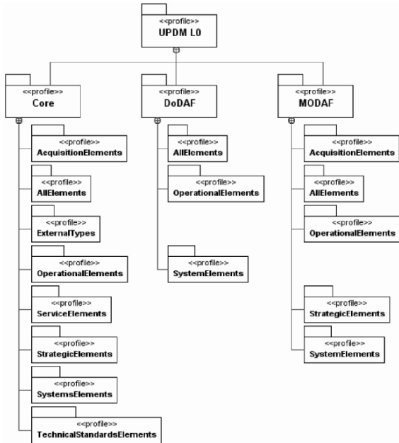
Figure 7.4.2 Middle Level Profile Structure
