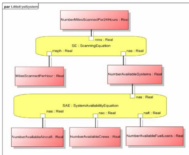
Figure D:48 - Scanning and Availability Equations
