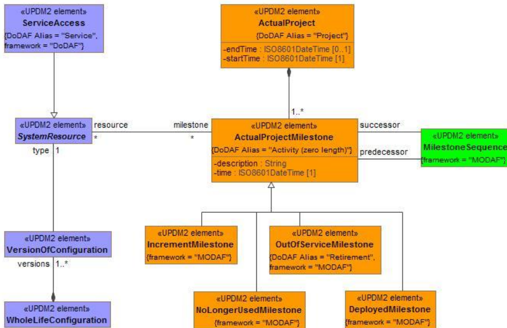
Figure A:43 - SV-8/SvcV-8 - DMM
