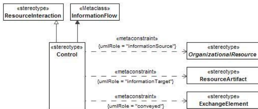
Figure 8:206 - Control
