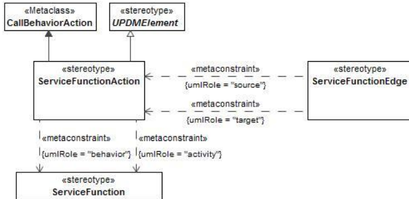
Figure 8:85 - ServiceFunctionAction
