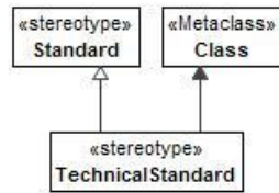
Figure 8:180 - TechnicalStandard
