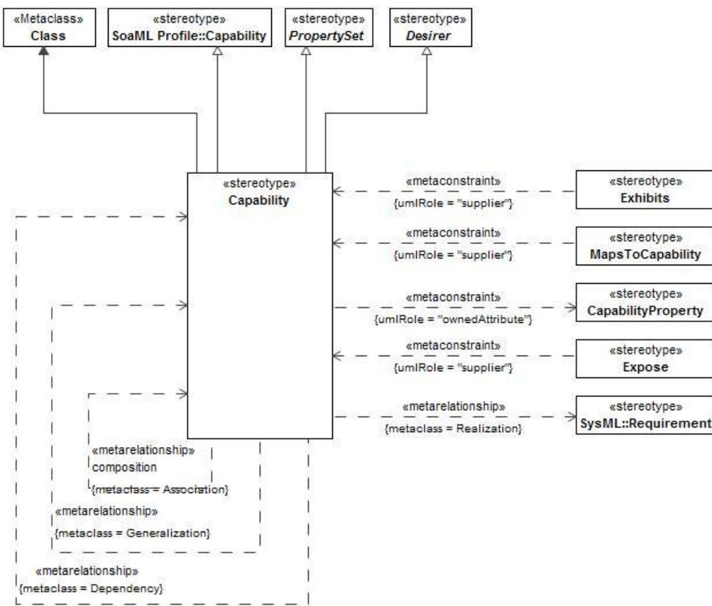
Figure 8:102 - Capability
