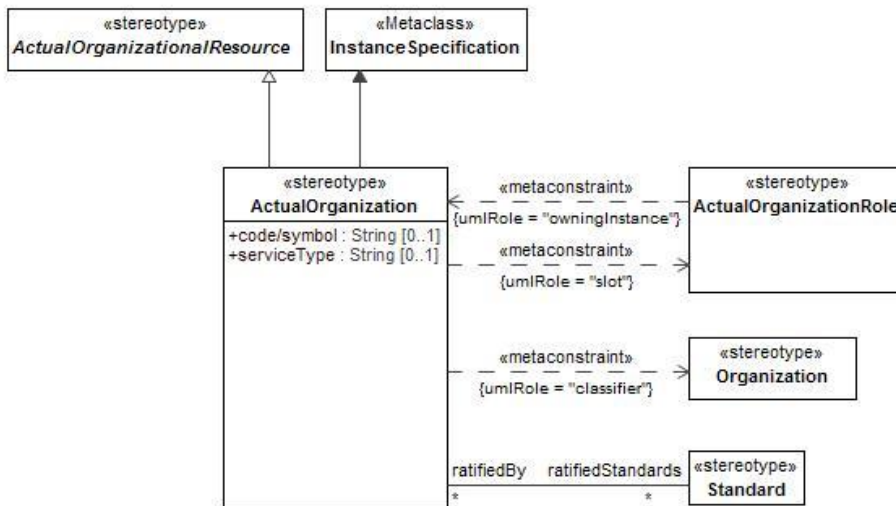
Figure 8:67 - ActualOrganization
