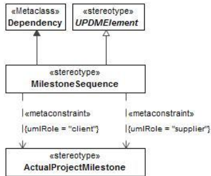
Figure 8:185 - MilestoneSequence
