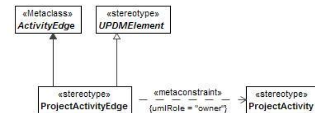
Figure 8:156 - ProjectActivityEdge
