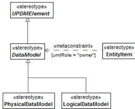
Figure 8:123 - DataModel
