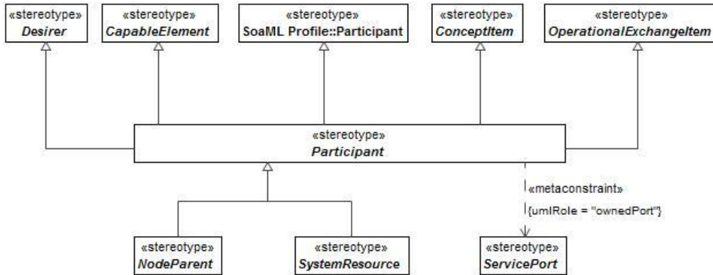
Figure 8:27 - Participant
