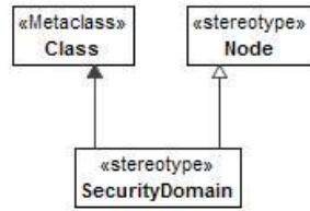
Figure 8:65 - SecurityDomain
