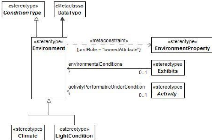
Figure 8:15 - Environment
