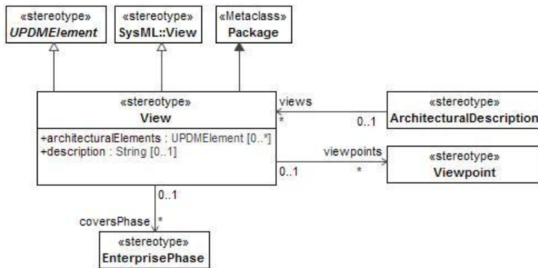
Figure 8:34 - View
