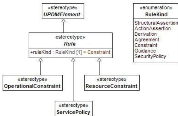
Figure 8:29 - Rule
