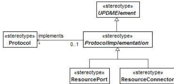
Figure 8:145 - ProtocolImplementation
