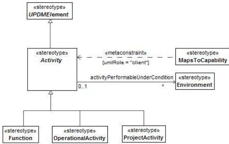
Figure 8:9 - Activity
