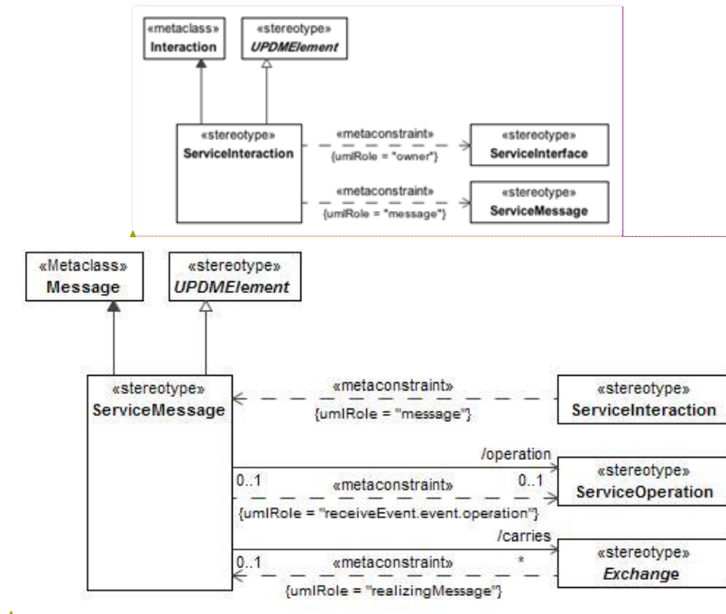
Figure 8:88 - ServiceMessage
