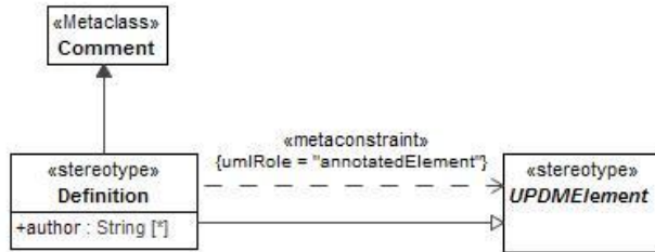
Figure 8:196 - Definition
