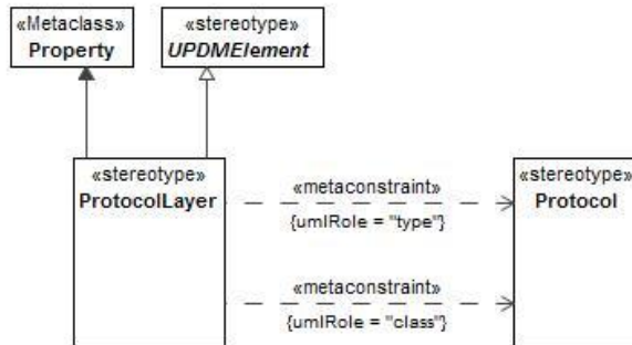
Figure 8:215 - ProtocolLayer
