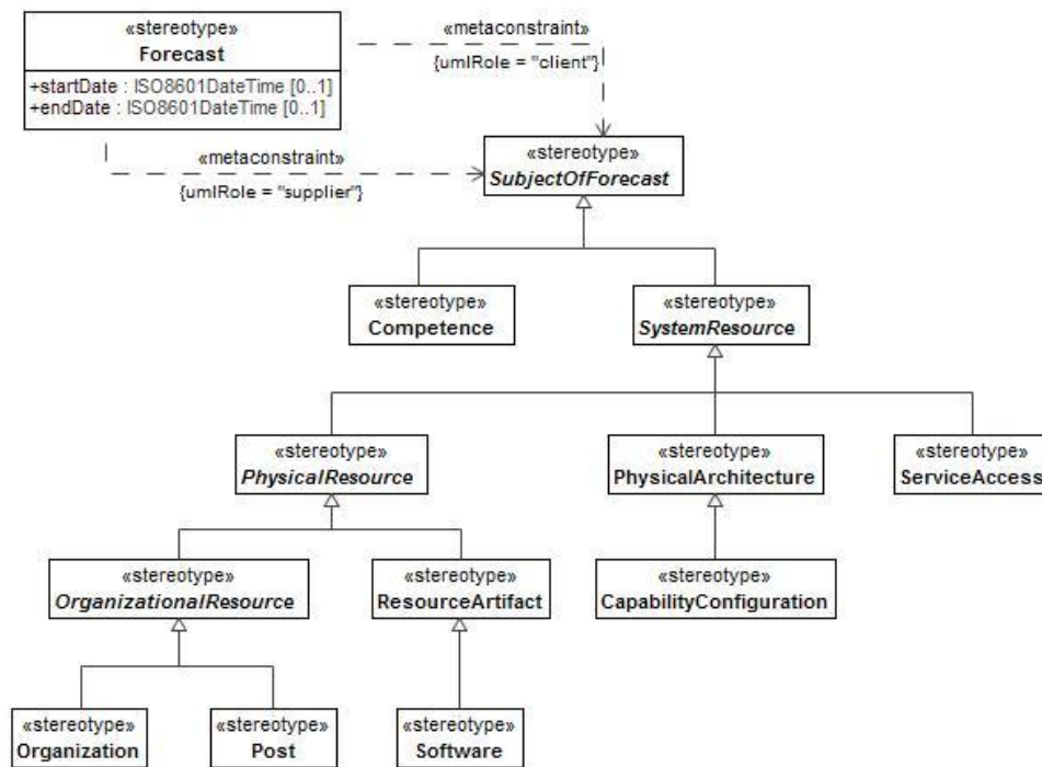
Figure B:46 - SV-9/SvcV-9
