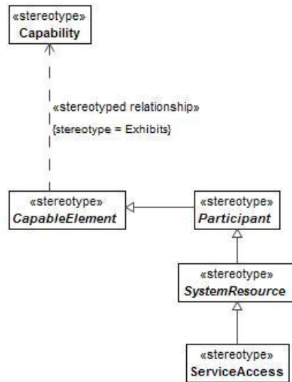
Figure B:26 - CV-7
