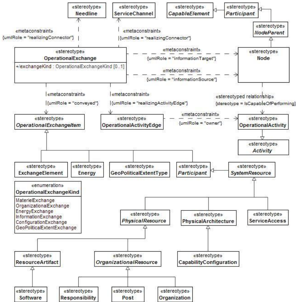
Figure B:11 - OV-3
