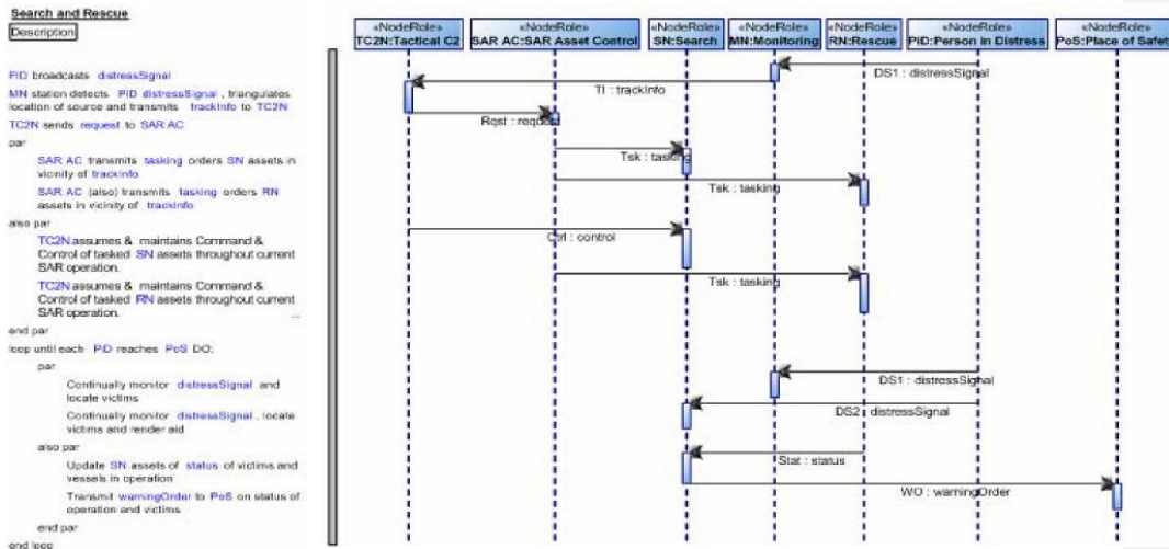
Figure D:23 - OV-6c
