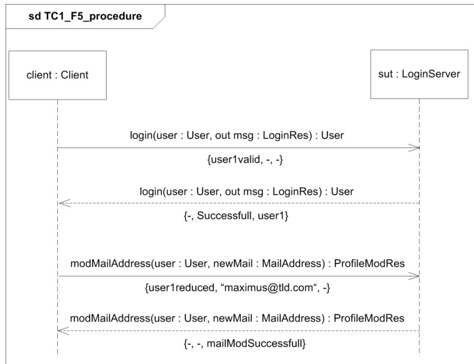
Figure A.17 - Successful Test Case
