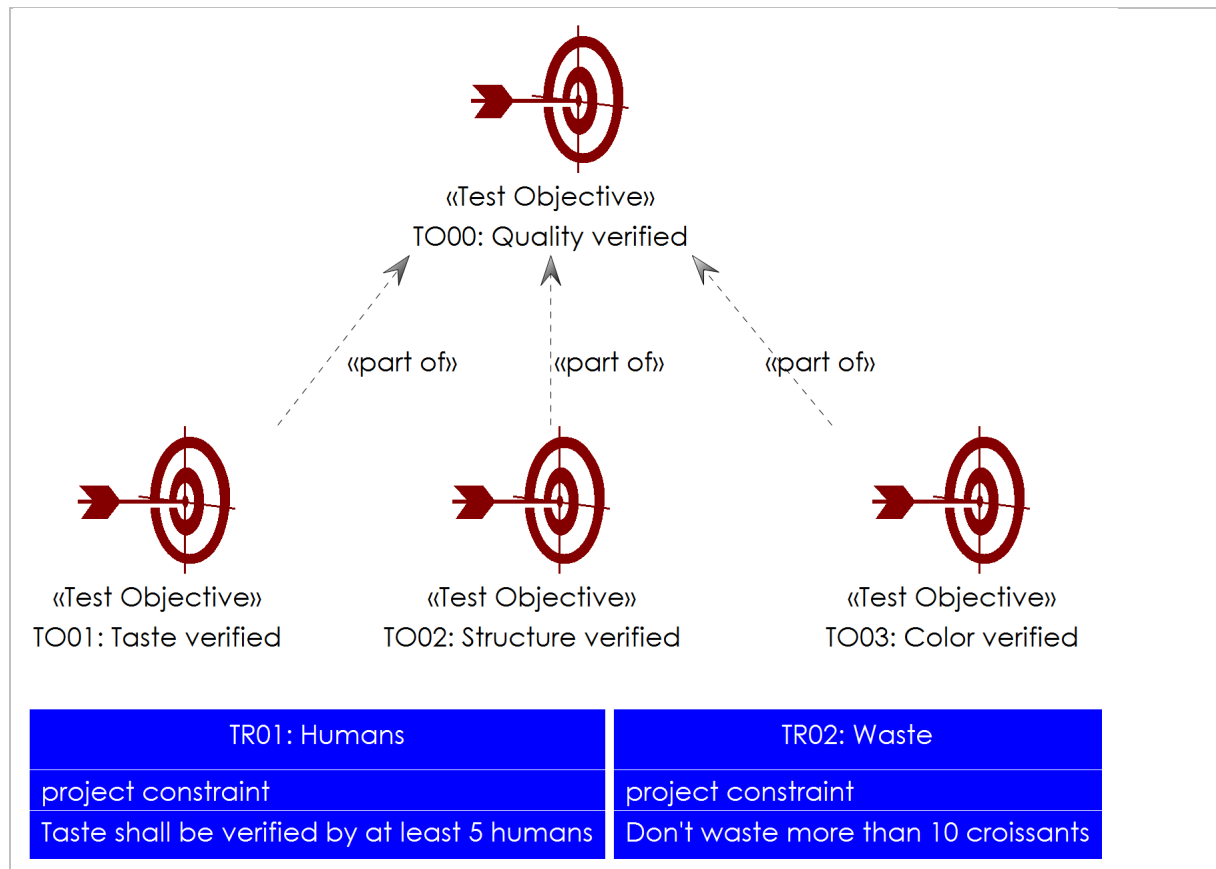
Figure A.2 - Test Objectives
