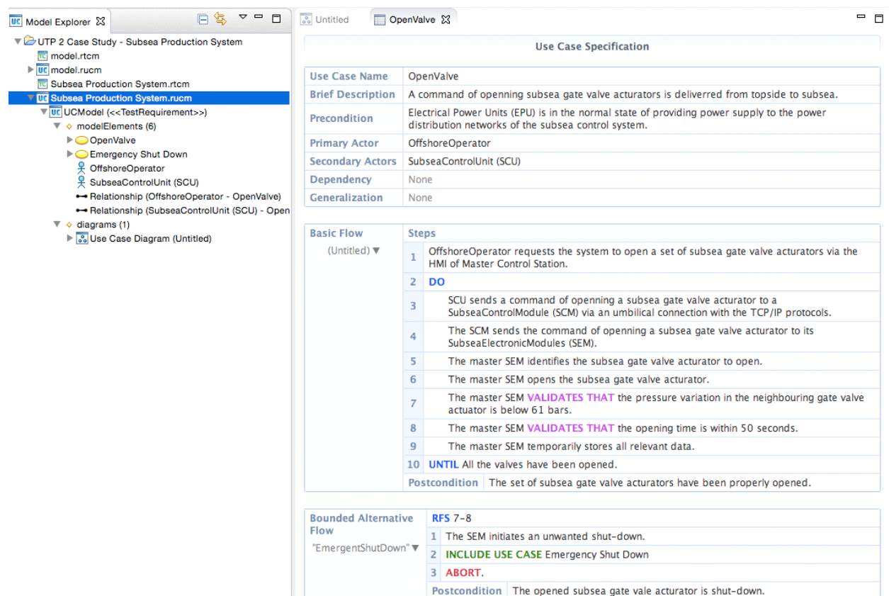
Figure A.1 - Use Case OpenValve (Specified in RUCM)
