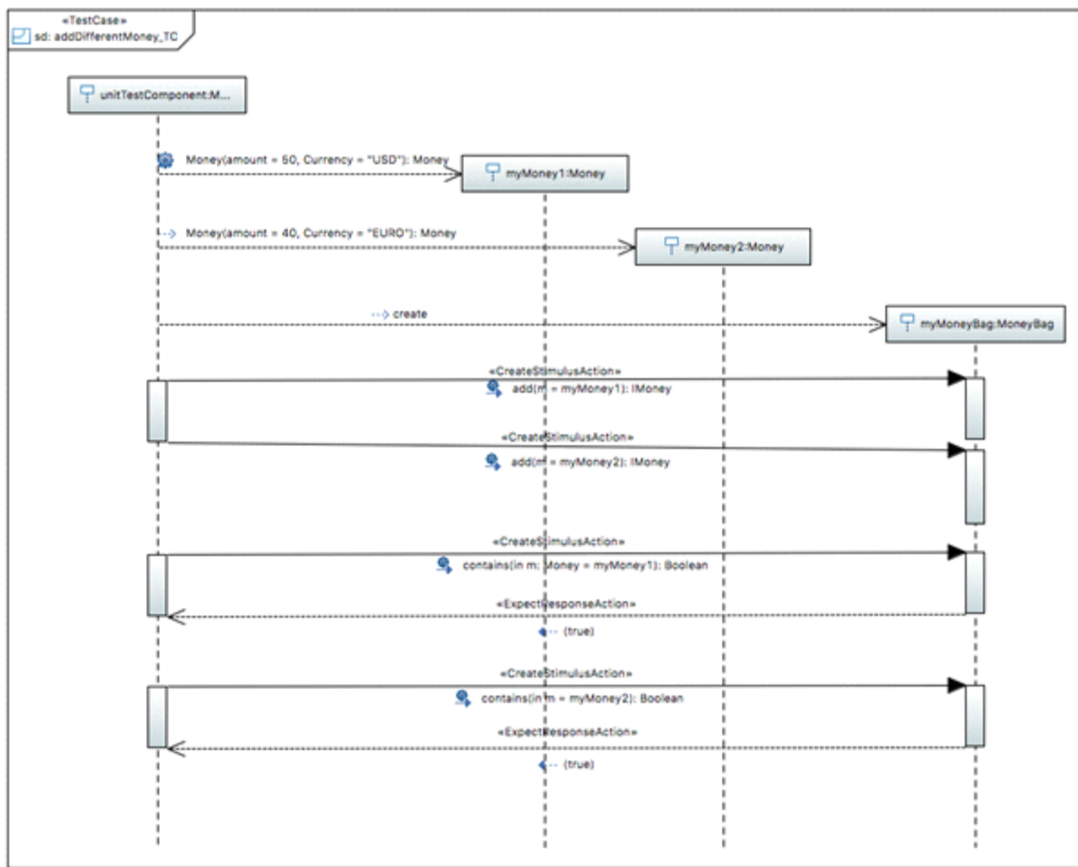
Figure A.10 - Test Case AddDifferentMoney
