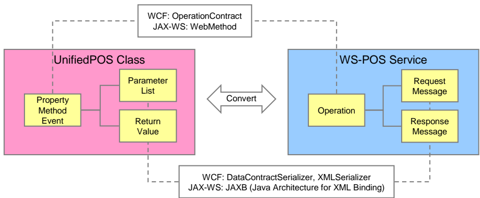
Figure 37: UnifiedPOS and WSDL Mapping
