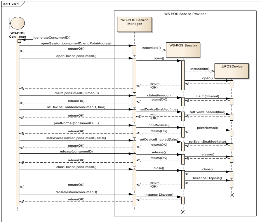
Figure 10: POS Printer - Print Normal example
