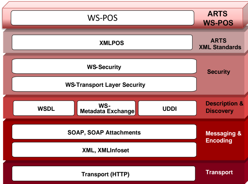
Figure 2: ARTS-WS-POS Stack
