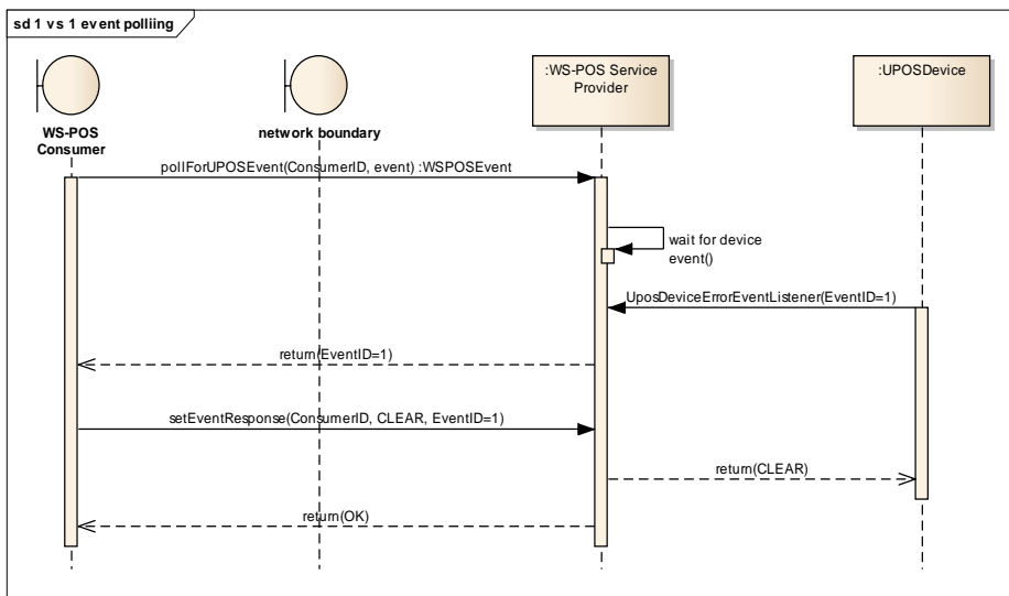
Figure 17: Event Polling
