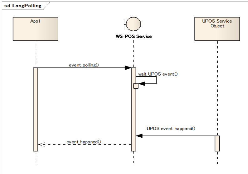
Figure 19: Long Polling Overview
