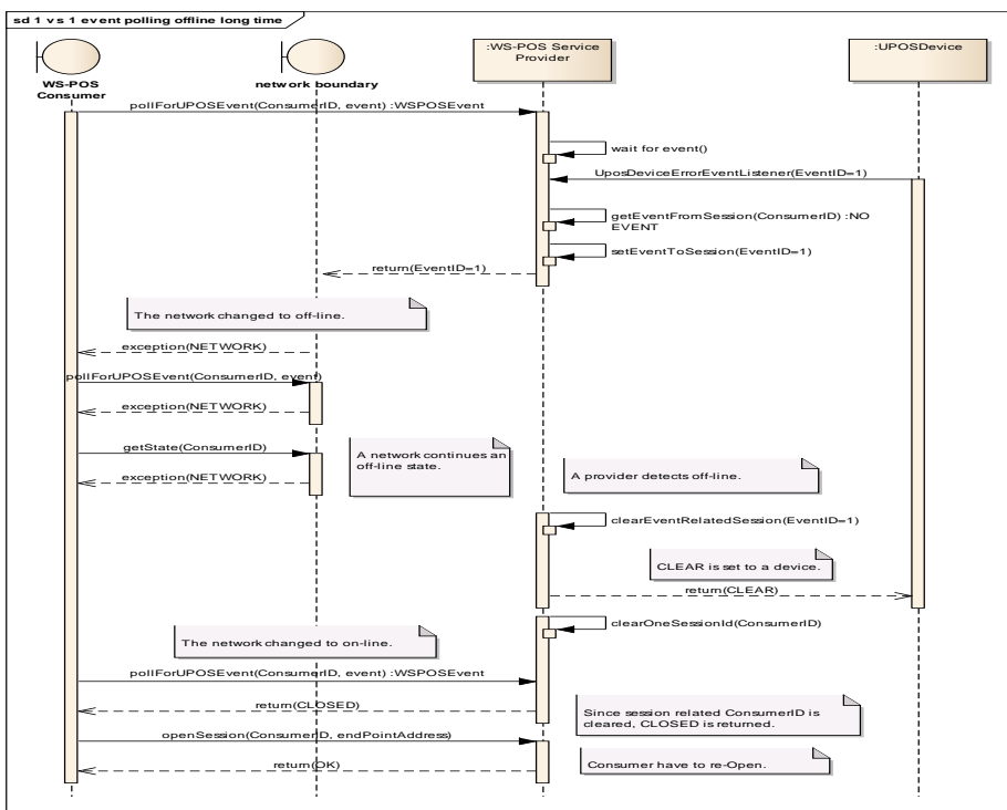
Figure 28: Offline Longer than Session Time Out in Event Polling
