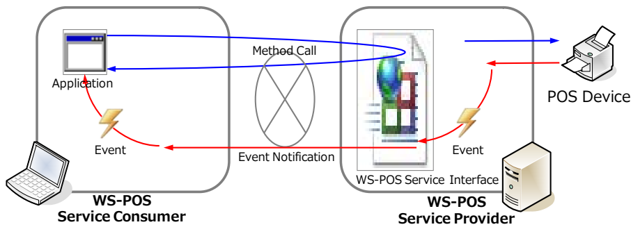
Figure 15: Method Call with Event Notification
