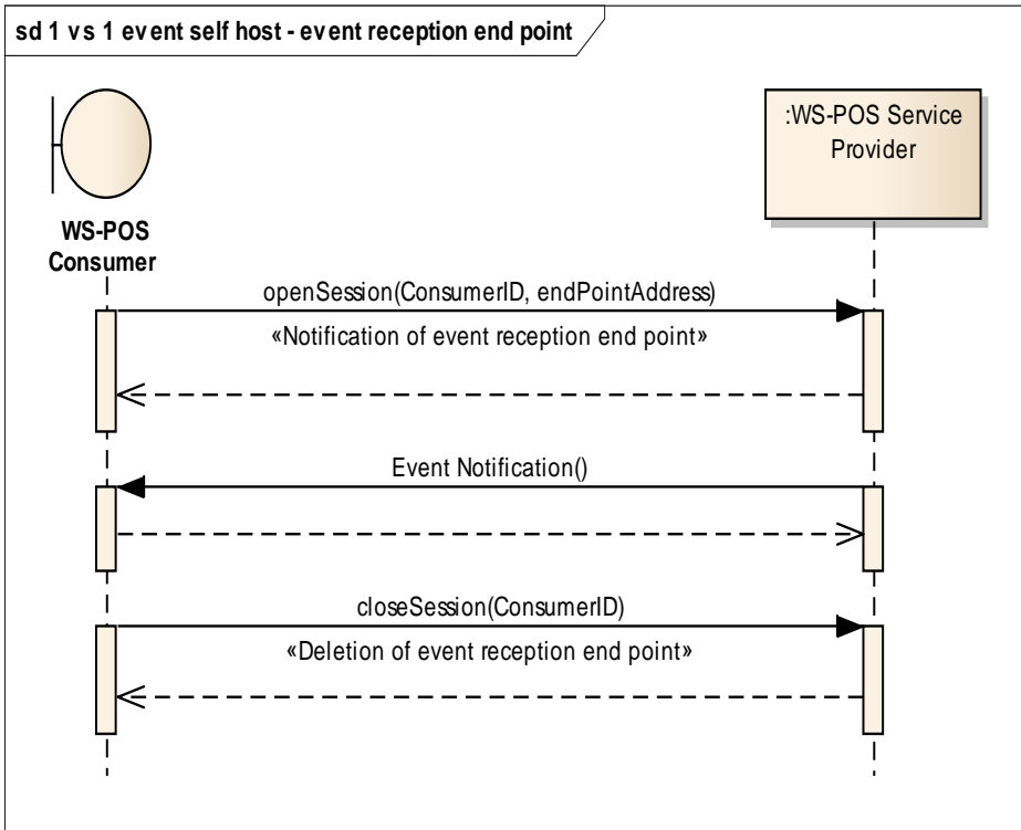
Figure 14: Event Self Host - Event Reception End Point
