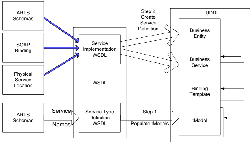
Figure 3: ARTS Schema - WSDL - UDDI Relationship
