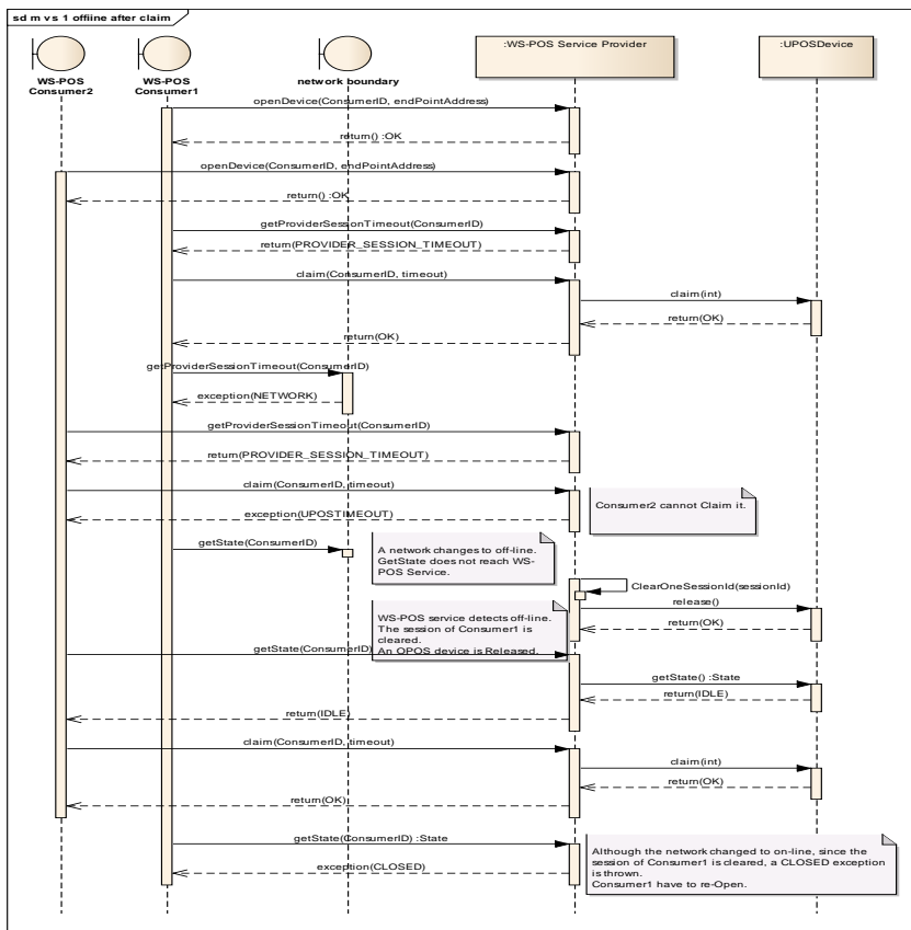
Figure 21: Offline after Claim
