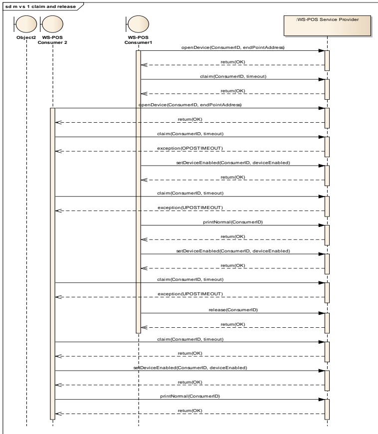
Figure 12: Claim and Release
