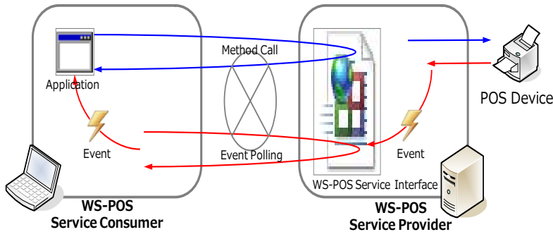
Figure 7 Polling Communication concept
