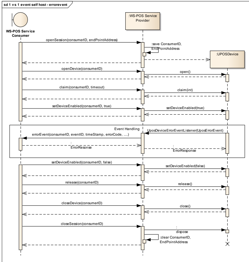
Figure 16: Event Self Host - Error Event
