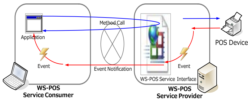
Figure 6 Bi-Directional Communication concept
