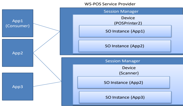
Figure 8: Session Management layer and Device Control layer
