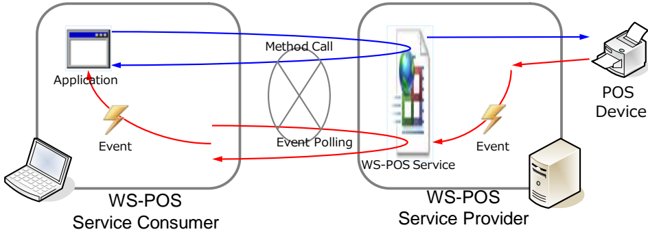
Figure 18 Method call and Event notification
