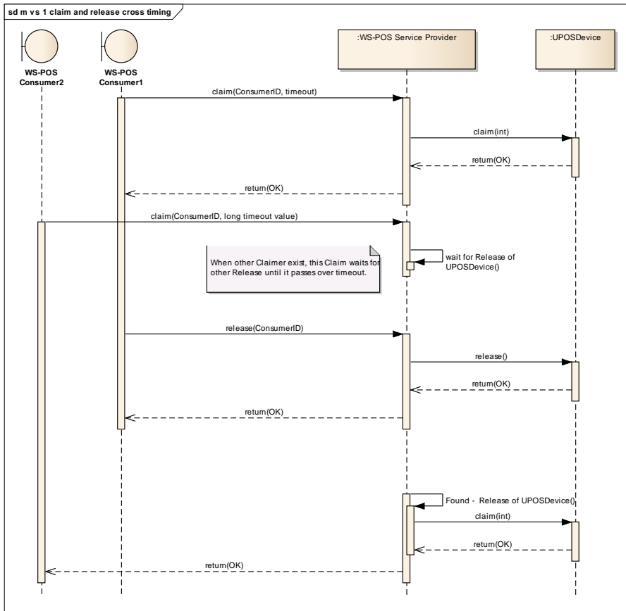
Figure 13: Claim and Release Cross Timing
