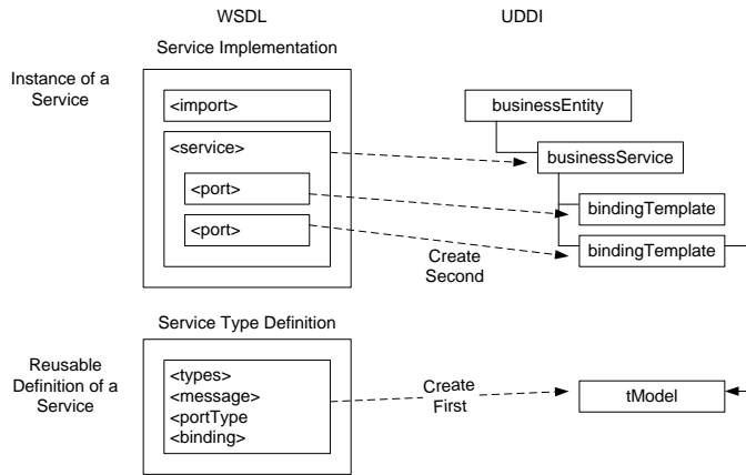
Figure 5: Registering a WSDL with a UDDI Registry
