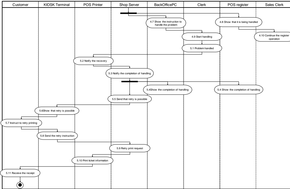
Normal Scenario 2/2
