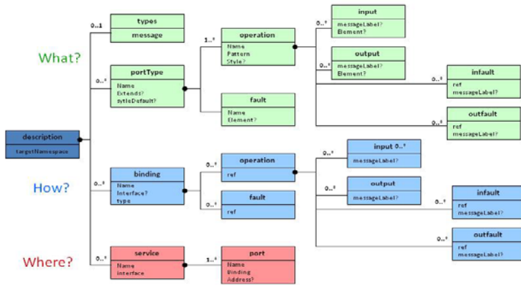
Figure 35: WSDL Overview
