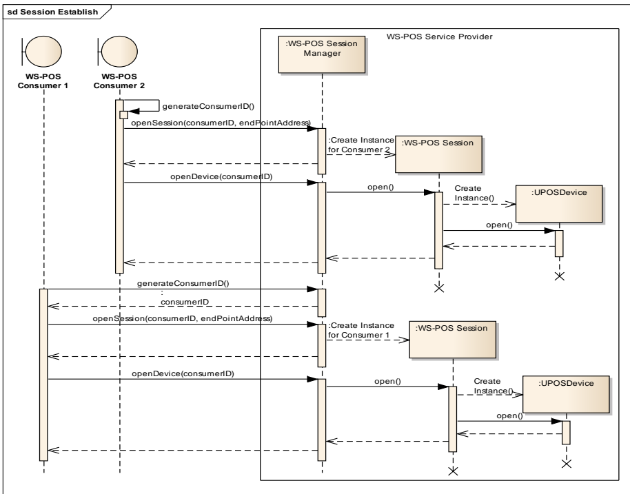
Figure 9: Establish Session
