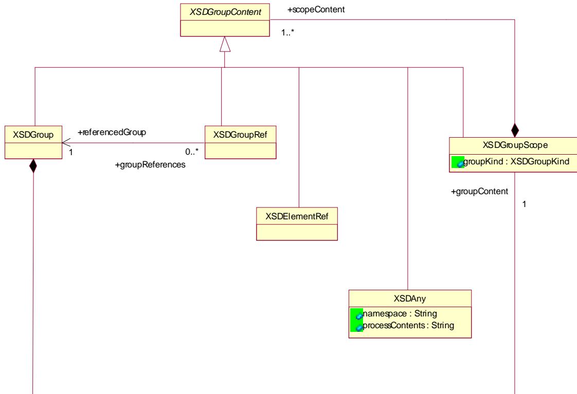
Figure 5-9 XML Schema group declarations
