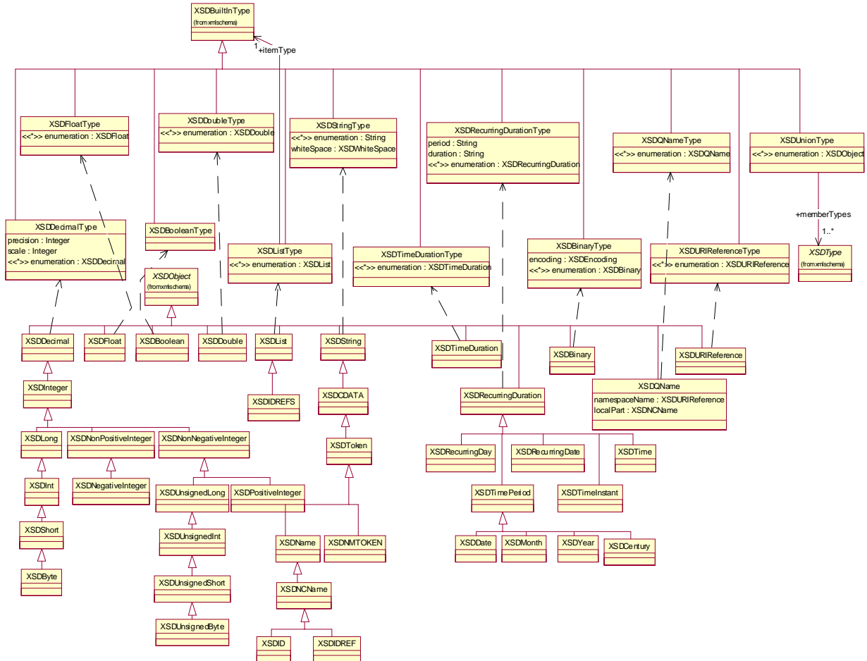
Figure 5-13 XML Schema data types
