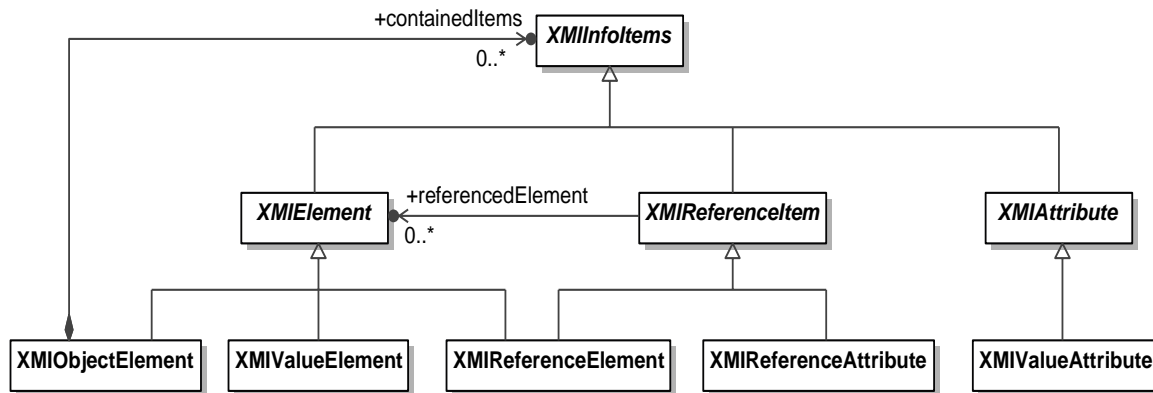
Figure 9.1- Serialization Model
