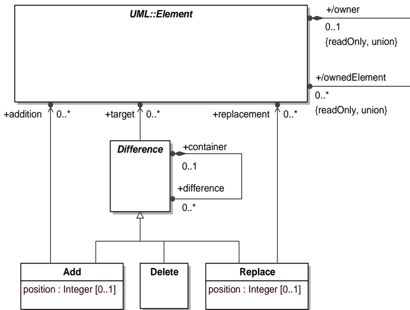
Figure 7.2 - The XMI Model for differences
