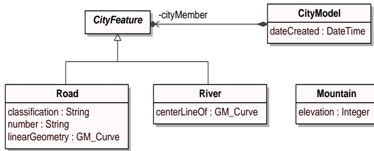
Figure 7.3 - GIS meta model
