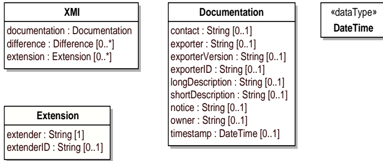
Figure 7.1- The XMI Model for the XMI element, documentation, and extension
