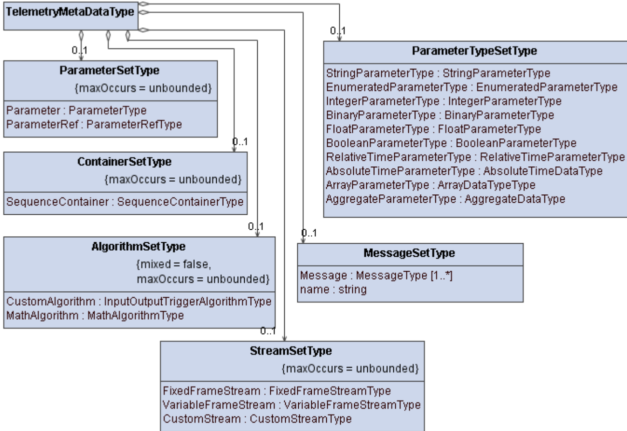
Figure 3 - Telemetry MetaData UML Class Diagram
