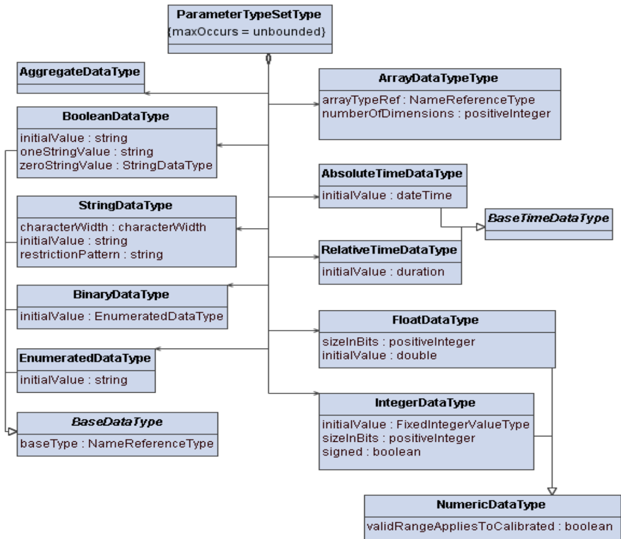
Figure 4 - ParameterTypeSet UML Class Diagram
