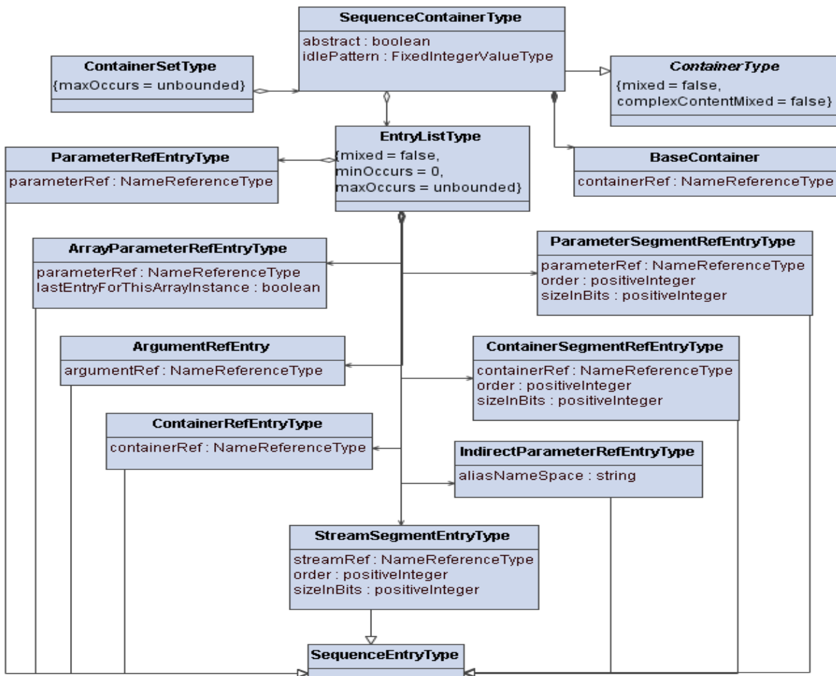
Figure 5 - Container UML Class Diagram
