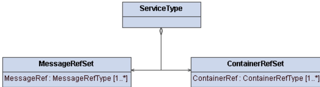
Figure 10 - ServiceType UML Class Diagram
