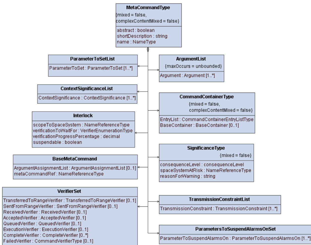
Figure 9: MetaCommandType UML Class Diagram
