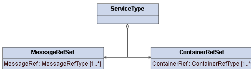
Figure 10: ServiceType UML Class Diagram
