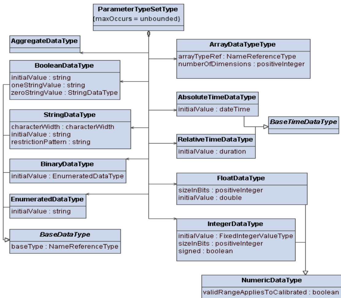
Figure 4: ParameterTypeSet UML Class Diagram
