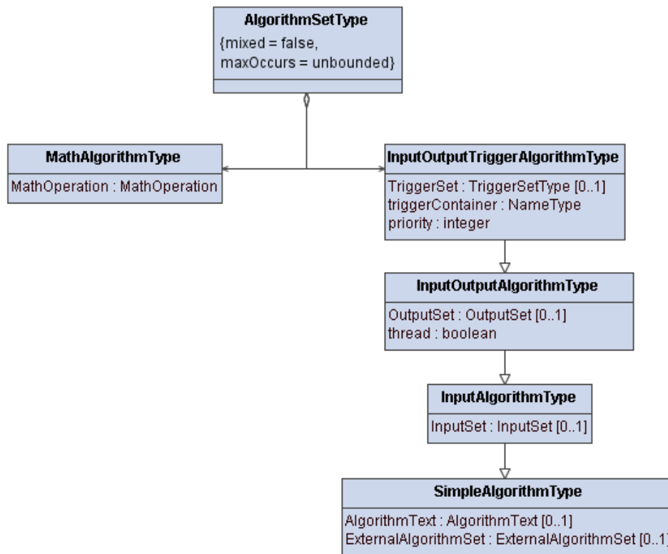
Figure 7: AlgorithmSet UML Class Diagram
